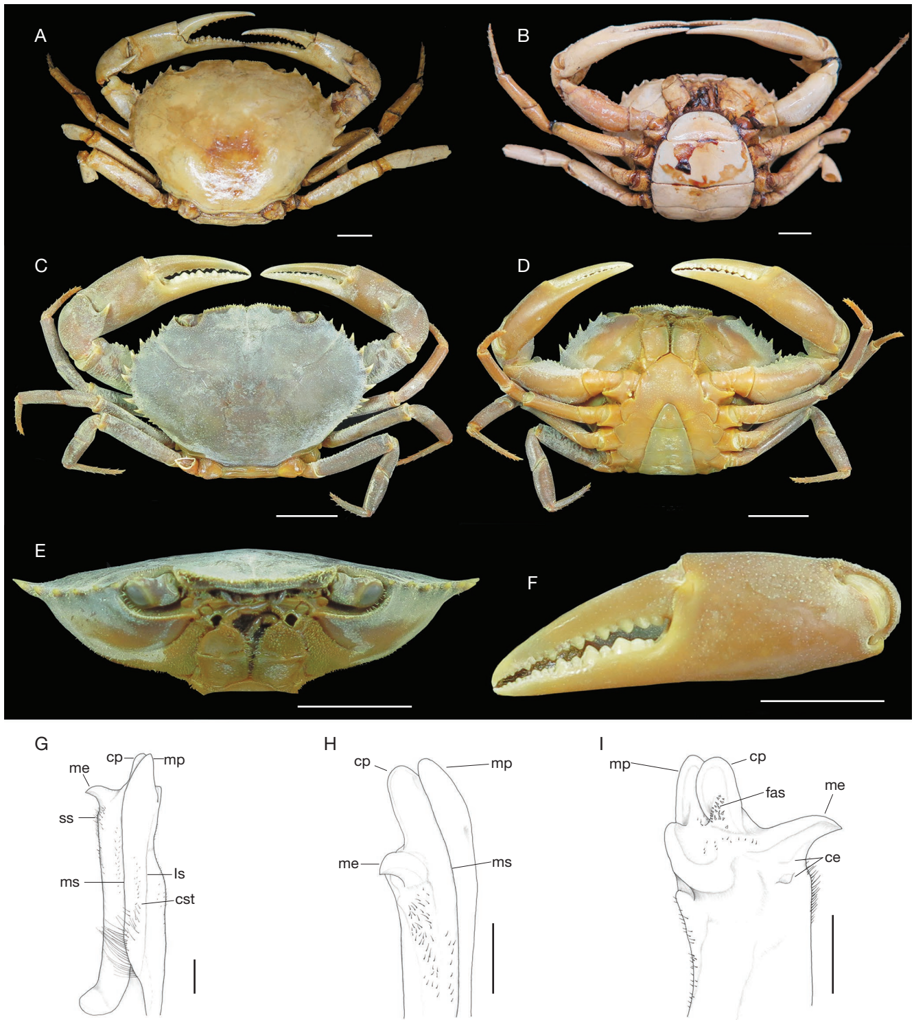
FIG. 1. — Potamocarcinus armatus H. Milne Edwards, 1853, A, B , female, holotype, dry specimen, MNHN-IU-2000-4025 : A , habitus, dorsal view; B , habitus, ventral view; C-I , male, INPA 2123: C , habitus, dorsal view; D , ventral view; E , frontal view; F , left chelae (largest), lateral view; G , G1, left, mesocaudal view; H , left G1, distal portion, cephalic view; I , left G1, distal portion, laterocephalic view. Abbreviations: ce , cephalic process; cp , caudal process; cst , caudal patch of setae; fas , field of apical spines; ls , lateral suture; me , mesial process; mp , marginal process; ms , marginal suture; ss , mesocephalic subdistal patch of setae. Scale bars: A-F, 10 mm; G-I, 1 mm. Photos: C. Magalhães.
