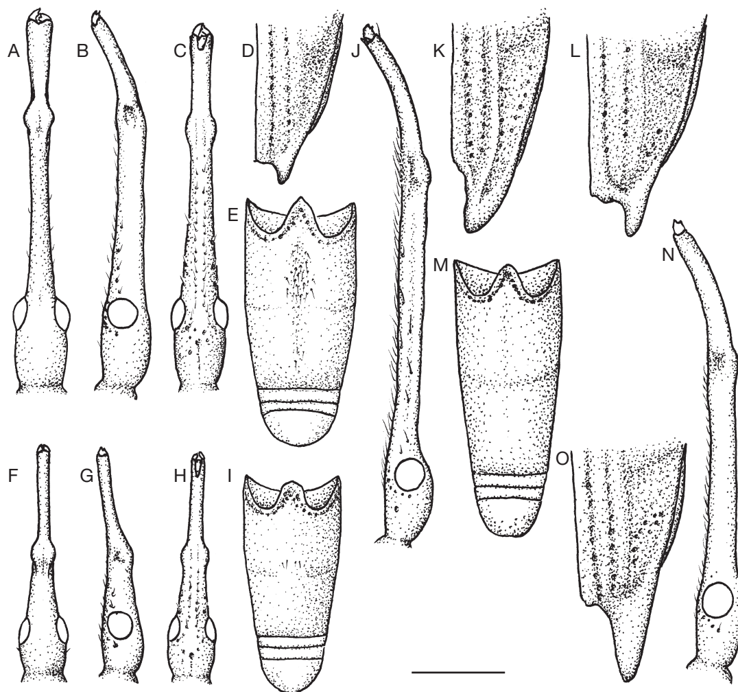
FIG. 7. — A-I , Teramocerus badius Boheman, 1840 comb. rev.; A-E , ♂: A , head, dorsal side; B , head, lateral view of left side; C , head, venter side; D , apex of right elytra, dorsal side; E , abdomen; F-I , ♀: F , head, dorsal side; G , head, lateral view of left side; H , head, venter side; I , abdomen; J-M , T. janthinus Boheman, 1840: J , ♂, head, lateral view of left side; K , ♂, apex of right elytra, dorsal side; L , ♀, apex of right elytra, dorsal side; M , ♂, abdomen; N-O , T. opacus (Perty, 1832) n. comb., ♂: N , head, lateral view of left side; O , apex of right elytra, dorsal side. Scale bar: A-C, E-J, M, N, 2 mm; D, K, L, O, 1 mm.
