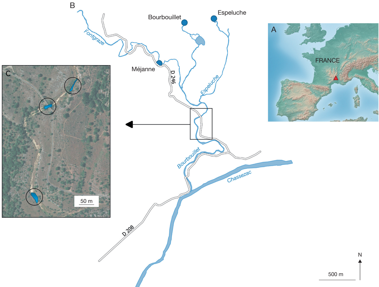
FIG. 2. — Red triangle indicates the locality of the study area (A), hydrographic network of the study area (B) and study site (C). Blue dots represent the main resurgences. Black open circles show remnant pools (in blue). White bands represent roads.
