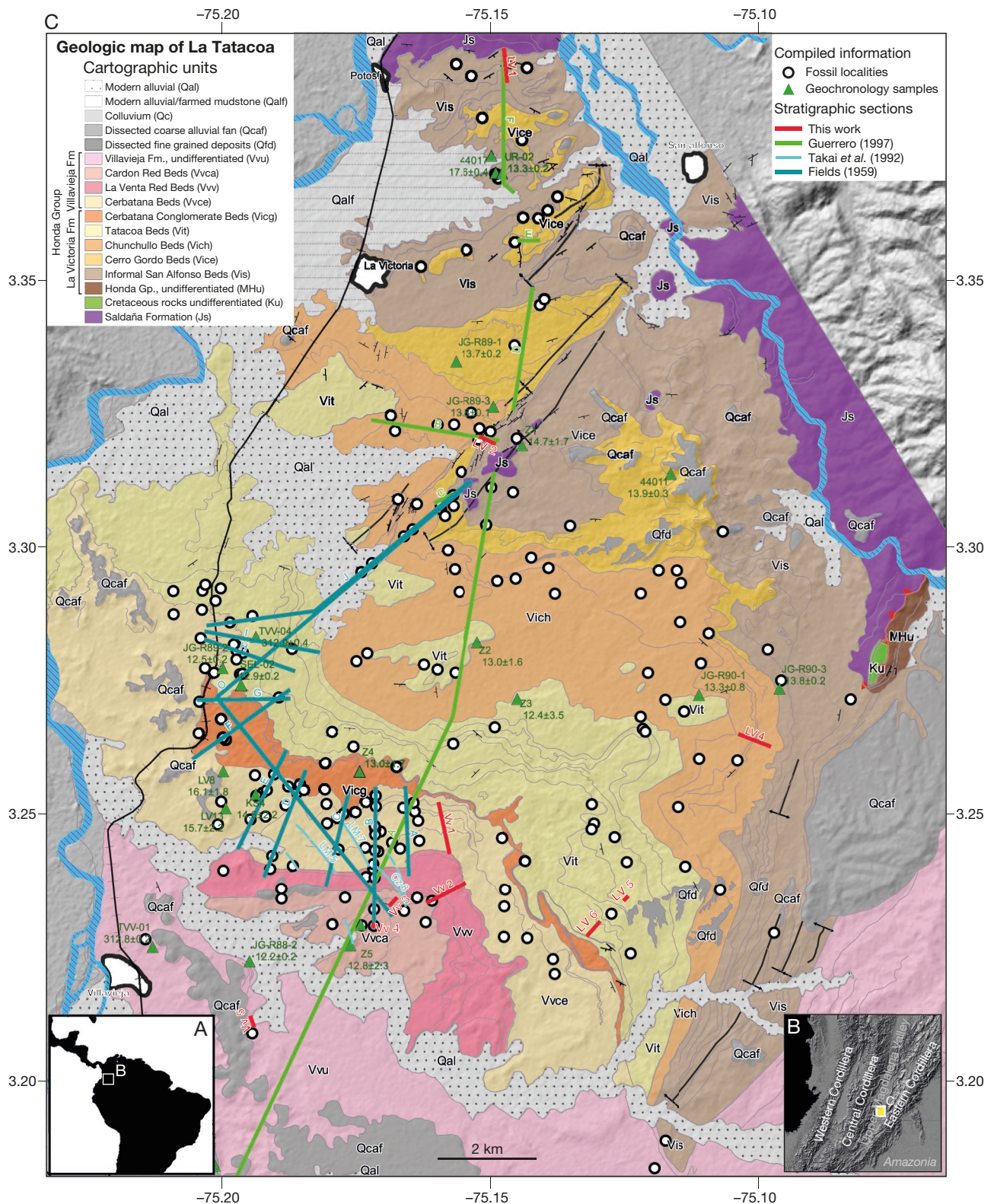
FIG. 1. — Fossil localities, stratigraphic sections, and geochronology samples placed in the geologic map of Montes et al. (2021): A , location of La Venta Site in South America; B , location of La Venta Site in the northern Andes; C , geologic map of La Venta Site (Montes et al. 2021).
