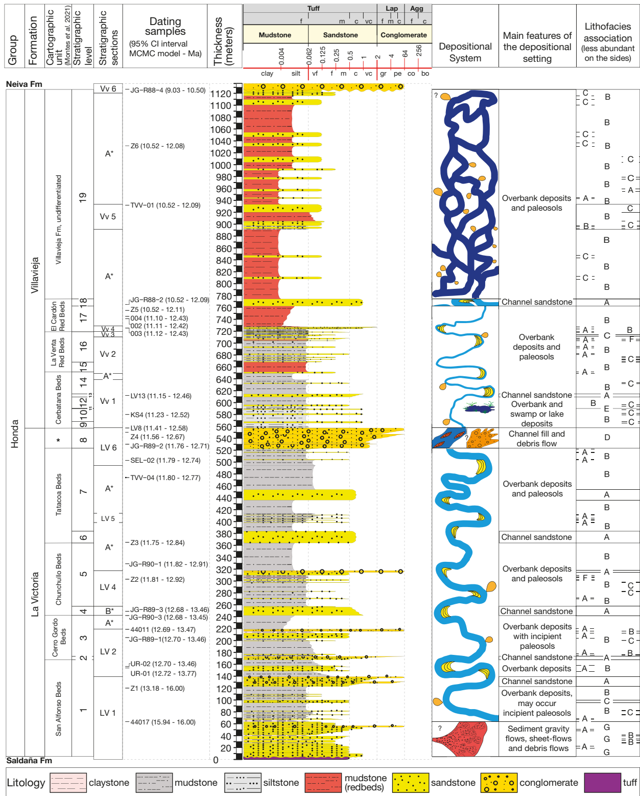
Fig. 2. — Composite standard section ( CS ) of the Honda Group at the La Venta site. We estimated the stratigraphic position of geochronology samples from information reported in the literature, graphic correlations (Supplementary material, Appendix 5), and the geologic map of Montes et al. (2021). Depositional systems, main features of the depositional settings, and lithofacies associations are on the right side of the CS. Cartographic unit: *, Cerbatana Conglomerate Beds; Stratigraphic levels: **, 11 (Fish Bed); ***, 13 (Ferruginous Beds). Stratigraphic sections: LV1 , LV2 , LV4 , LV5 , LV6 , Vv1 , Vv2 , Vv3 , Vv4 , Vv5 , Vv6 , this work. Stratigraphic sections: A* , B* , Guerrero 1997. Geochronology sample references: Takemura et al. (1992): 002, 003, and 004; Takemura & Danhara (1985): LV8, KS4 and LV13; Flynn et al. (1997): JG-R89-2, JG-R89-3, and JG-R88-2; Anderson et al. (2016): Z1, Z2, Z3, Z4, and Z5; Cadena et al. (2020): 46311(UR-01) and 46312 (UR-02); Montes et al. (2021): SEL-02; this work: 44017, 44011, TVV-04, and TVV-01. The stratigraphic position of geochronology samples was estimated by authors' reported information, graphic correlations, and the cartography of Montes et al. (2021).
