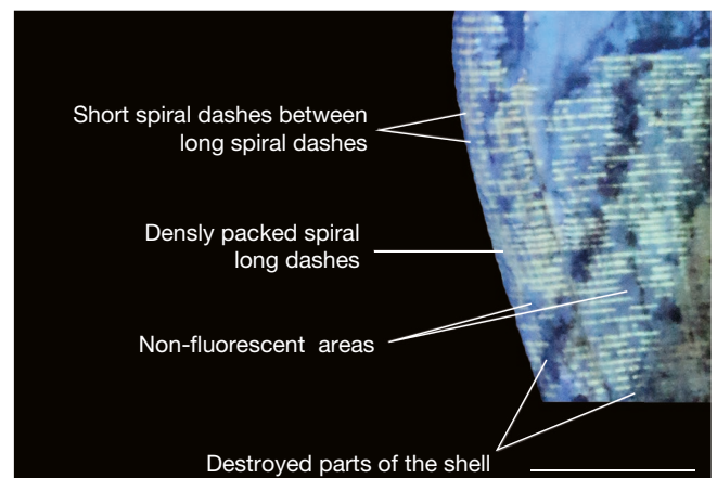
FIG. 23. — Pattern of the dashes on Conus (Kalloconus) letkesensis (Harzhauser & Landau, 2016). Dashed colour pattern is from AMPG(IV) 2682 (Fig. 22) from Filippi, Crete (Greece). Scale bar: 1 cm.
