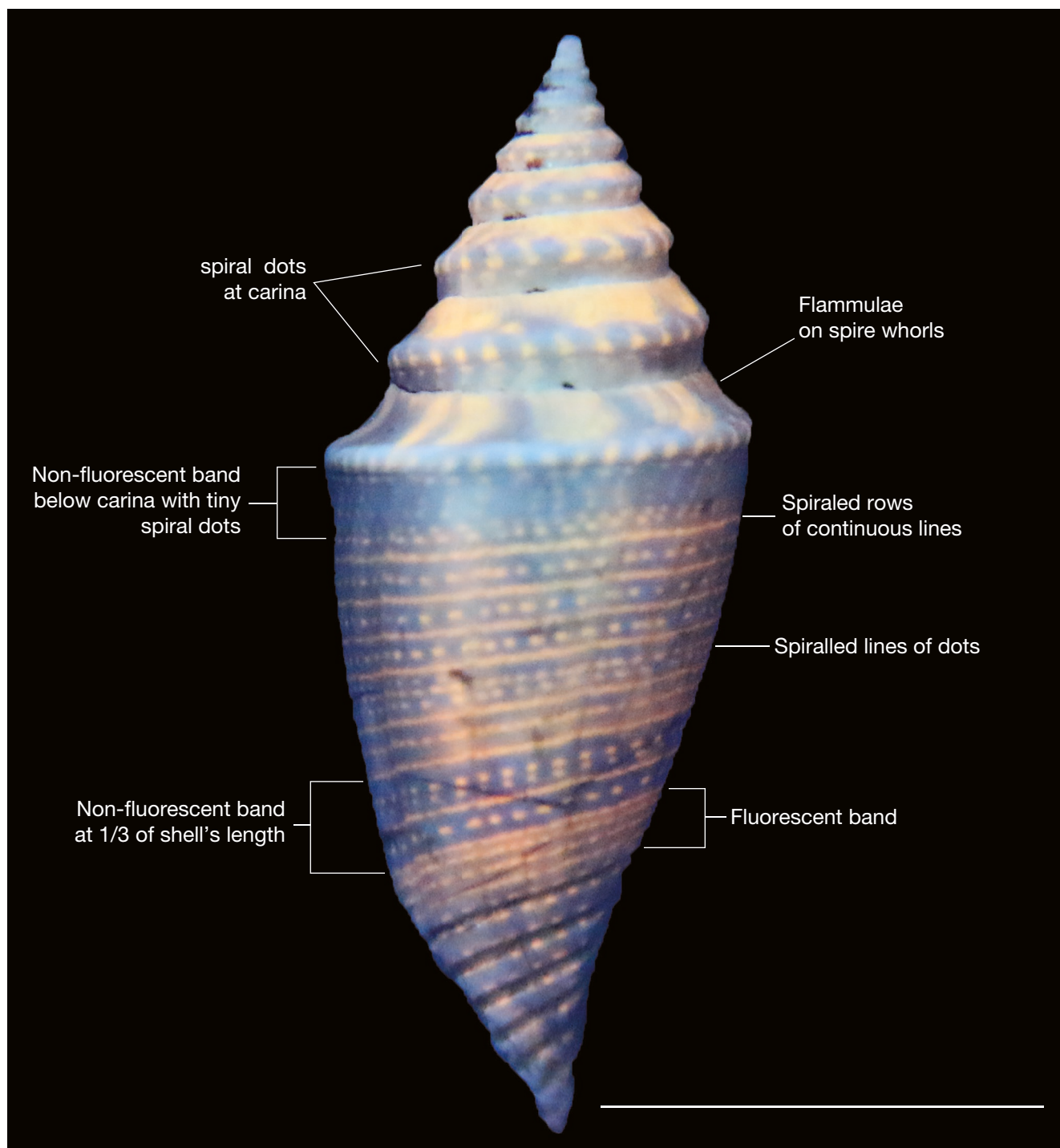
FIG. 3. — Elements constituting the colour patterns of Conilithes brezinae (Hoernes & Auinger, 1879), MNHN.F.A72565 , Tortonian of Crete (Greece). Scale bar: 1 cm.
