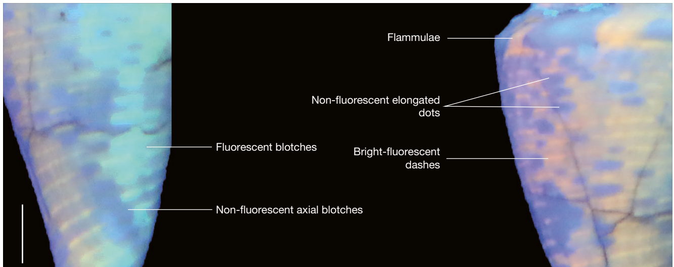
FIG. 8. — Elements constituting the colour pattern of Conilithes sp. (MNHN.F.A72593, Makrilia, Crete, Greece). Scale bar: 0.2 cm.
