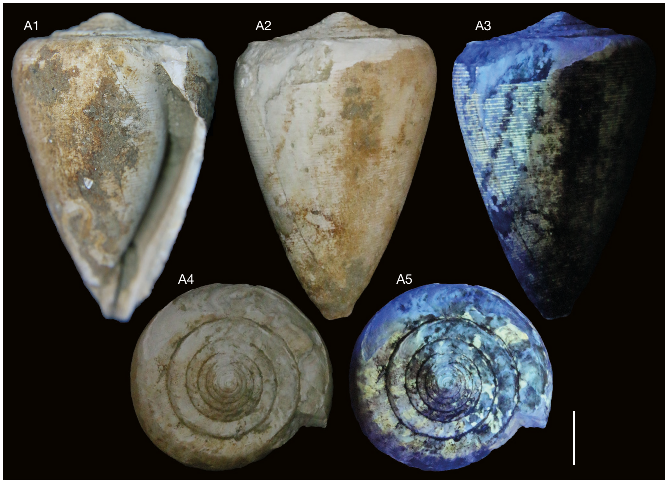
FIG. 22. — Conus (Kalloconus) letkesensis (Harzhauser & Landau, 2016) from Filippi, Crete (Greece). Specimen AMPG(IV) 2682 with small dense dashes and irregular flammulae on the spire. Specimen shown under natural light (A1–A2, A4) and UV light (A3, A5). Scale bar: 1 cm.
