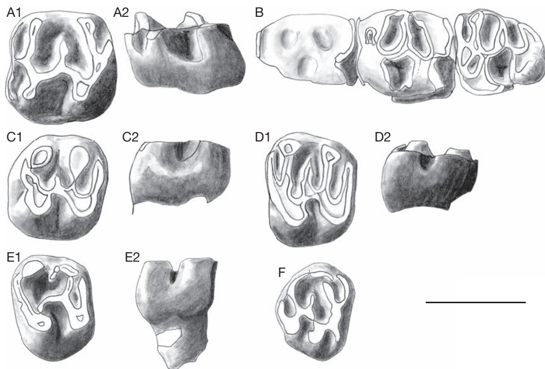
FIG. 14. — Eomys aff. zitteli Schlosser, 1884, from Saint-Privat-des-Vieux (Gard; Lower Chattian, MP 26): A , left m1-2, SPV184, (drawing reversed): A1 , occlusal view, A2 , lingual view; B , digested and worn m1-m3, SPV183, occlusal view; C , left P4, SPV180: C1 , occlusal view, C2 , lingual view; D , left M1-2, SPV181: D1 , occlusal view, D2 , lingual view; E , F , Eomys minor Comte & Vianey-Liaud, 1987, from Mas-de-Pauffié (Lot; Lower Chattian, MP 26): E , left M2, MPF215: E1 , occlusal view, E2 , lingual view; F , right M3, MPF216, occlusal view. Scale bar: 1 mm.
