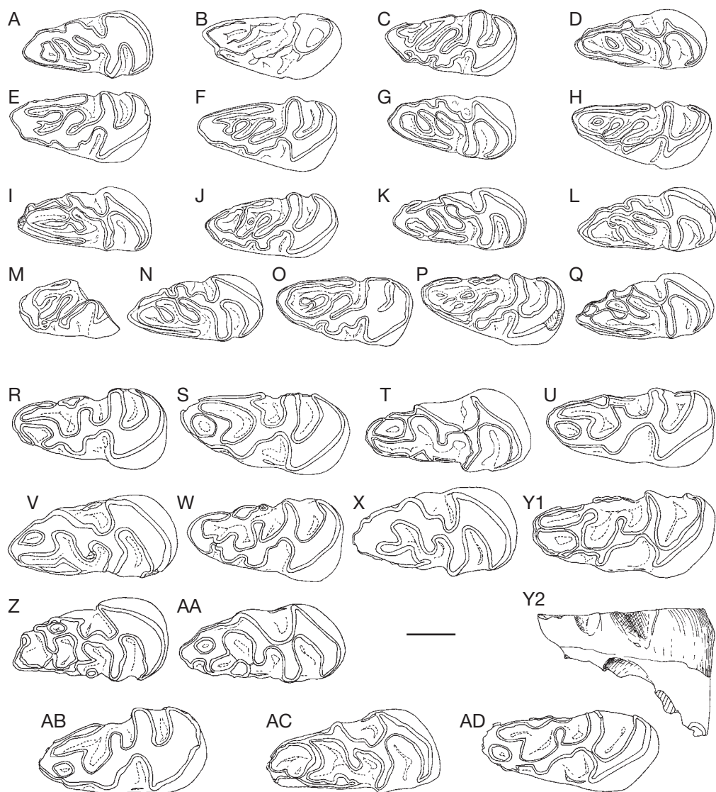
FIG. 4. — Variations of the occlusal surface of lower dp4 of Issiodoromys Bravard in Gervais, 1848: A-Q , I. pauffiensis Vianey-Liaud, 1976, from Saint-Privat-des-Vieux (Gard; Lower Chattian, MP 26): A , SPV415; B , SPV423; C , SPV433; D , SPV424; E , SPV417; F , SPV430; G , SPV425; H , SPV418; I , SPV426; J , SPV419; K , SPV437; L , SPV420; M , SPV439; N , SPV438; O , SPV429; P , SPV427; Q , SPV422; R-AD , I. quercyi (Schlosser, 1884) from Ehrenstein 7 (Germany; MP 27): R-X , Z-AD , occlusal views: R , no. 1983-XVIII 470; S , no. 1983-XVIII 457; T , no. 1983-XVIII 466; U , no. 1983-XVIII 460; V , no. 1983-XVIII 459; W , no. 1983-XVIII 458; X , no. 1983-XVIII 462; Y , no. 1983-XVIII 465, Y1 , occlusal view, Y2 , labial view; Z , no. 1983-XVIII 468; AA , no. 1983-XVIII 463; AB , no. 1983-XVIII 464; AC , no. 1983-XVIII 461; AD , no. 1983-XVIII 467. Scale bar: 1 mm.
