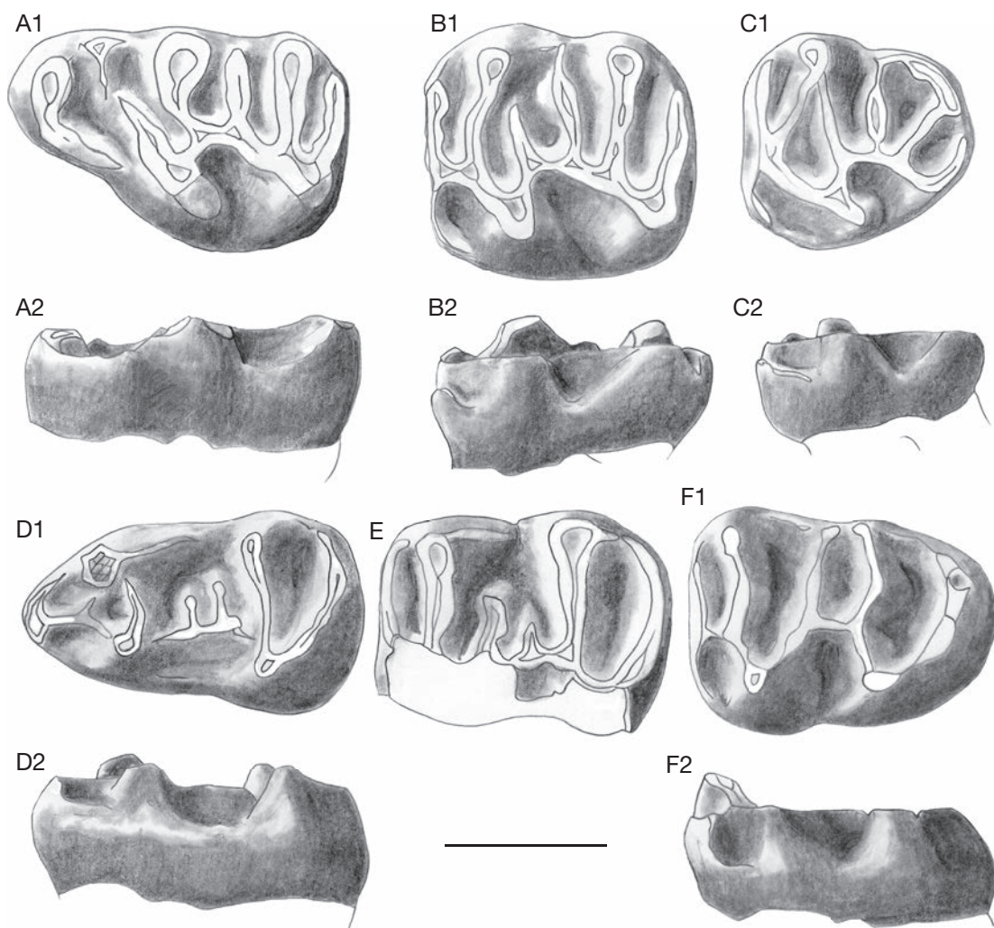
FIG. 12. — Heterocricetodon gaimersheimensis Freudenberg, 1941, from Saint-Privat-des-Vieux (Gard; Lower Chattian, MP 26): A , right M1 (reversed), SPV170: A1 , occlusal view, A2 , lingual view; B , left M2, SPV171: B1 , occlusal view, B2 , lingual view; C , right M3 (reversed), SPV174: C1 , occlusal view, C2 , lingual view; D , right m1 (reversed), SPV175: D1 , occlusal view, D2 , lingual view; E , left m2, SPV178, occlusal view; F , left m3, SPV179: F1 , occlusal view, F2 , lingual view. Scale bar: 1 mm.
