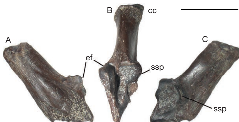
FIG. 16. — Right calcaneus of Lophiomyx cf. chalaniati Pomel, 1853, from Saint-Privat-des-Vieux (Gard; Lower Chattian, MP 26), SPV700. A , lateral side; B , dorsal aspect; C , medial side. Abbreviations: ef , ectal facet; cc , caput calcanei; ssp , sustentacular process. Scale bar: 2.5 cm.
