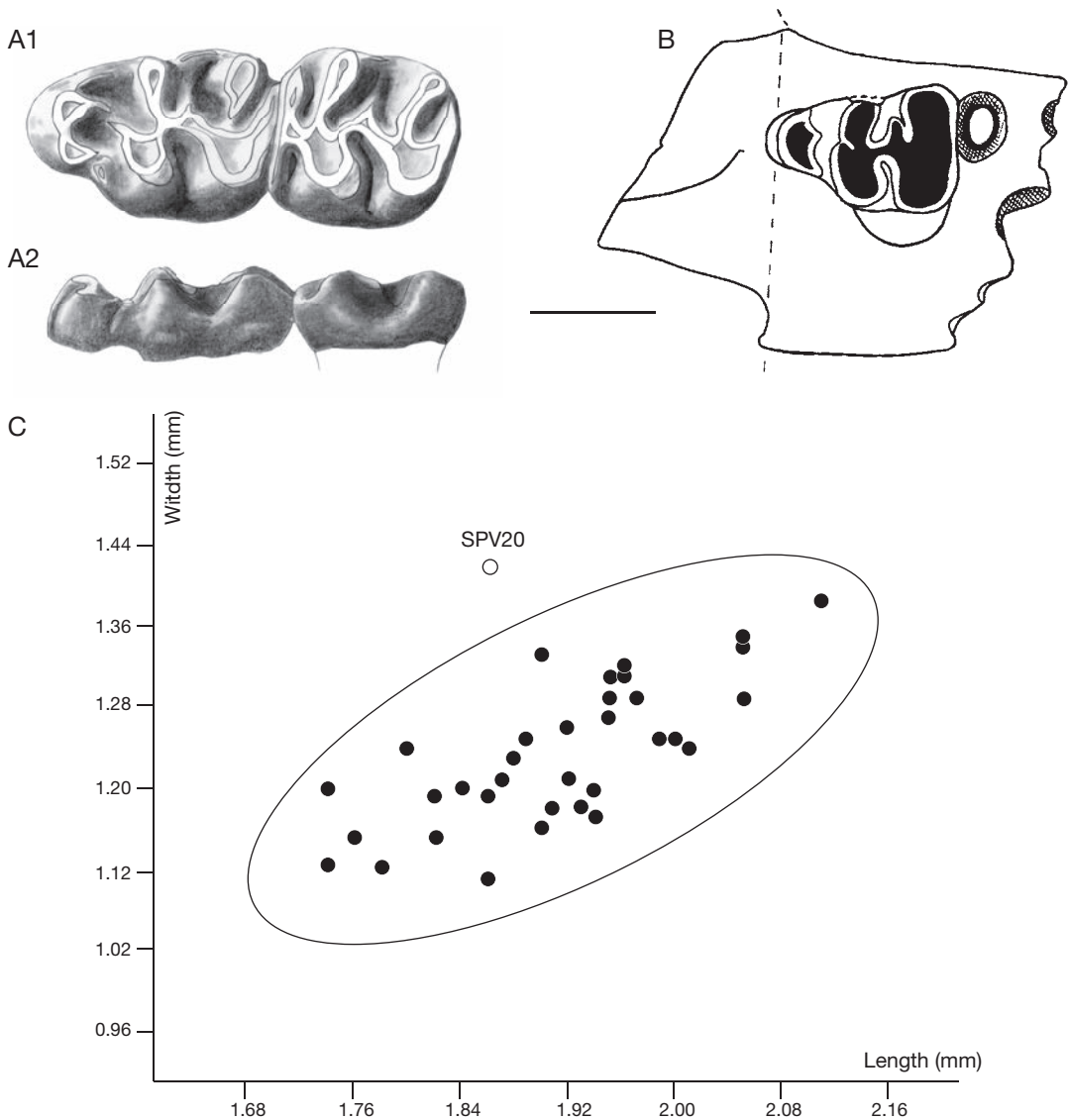
FIG. 11. — Other cricetids from Saint-Privat-des-Vieux (Gard; Lower Chattian, MP 26): A , Eucrietodon huerzeleri Vianey-liaud, 1972, left M1-M2 (reversed), SPV165: A1 , occlusal view, A2 , lingual view; B , Cricetidae indet., fragment of left maxillary with M1, SPV20, occlusal view; C , bivariate (Length and Width) diagram of M1 of Pseudocricetodon incertus (Schlosser, 1884) from Saint-Privat-des-Vieux. The open circle represents the M1 SPV20. The plots for the M1 of P. incertus are surrounded by their calculated equiprobable ellipse. Scale bar: 1 mm.
