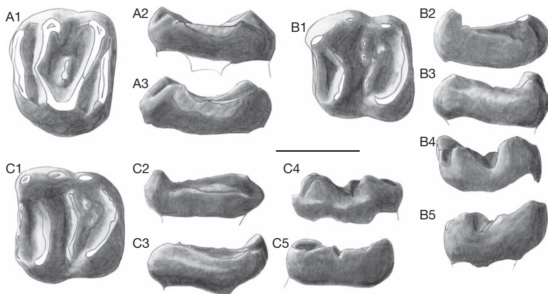
FIG. 13. — Gliravus bruijini Hugueney, 1967, from Saint-Privat-des-Vieux (Gard; Lower Chattian, MP 26): A , right M1-2, SPV192: A1 , occlusal view, A2 , distal view, A3 , mesial view; B , left m1-2, SPV196: B1 , occlusal view, B2 , mesial view, B3 , distal view, B4 , labial view, B5 , lingual view; C , left m1-2, SPV195: C1 , occlusal view, C2 , mesial view, C3 , distal view, C4 , labial view, C5 , lingual view. Scale bar: 1 mm.
