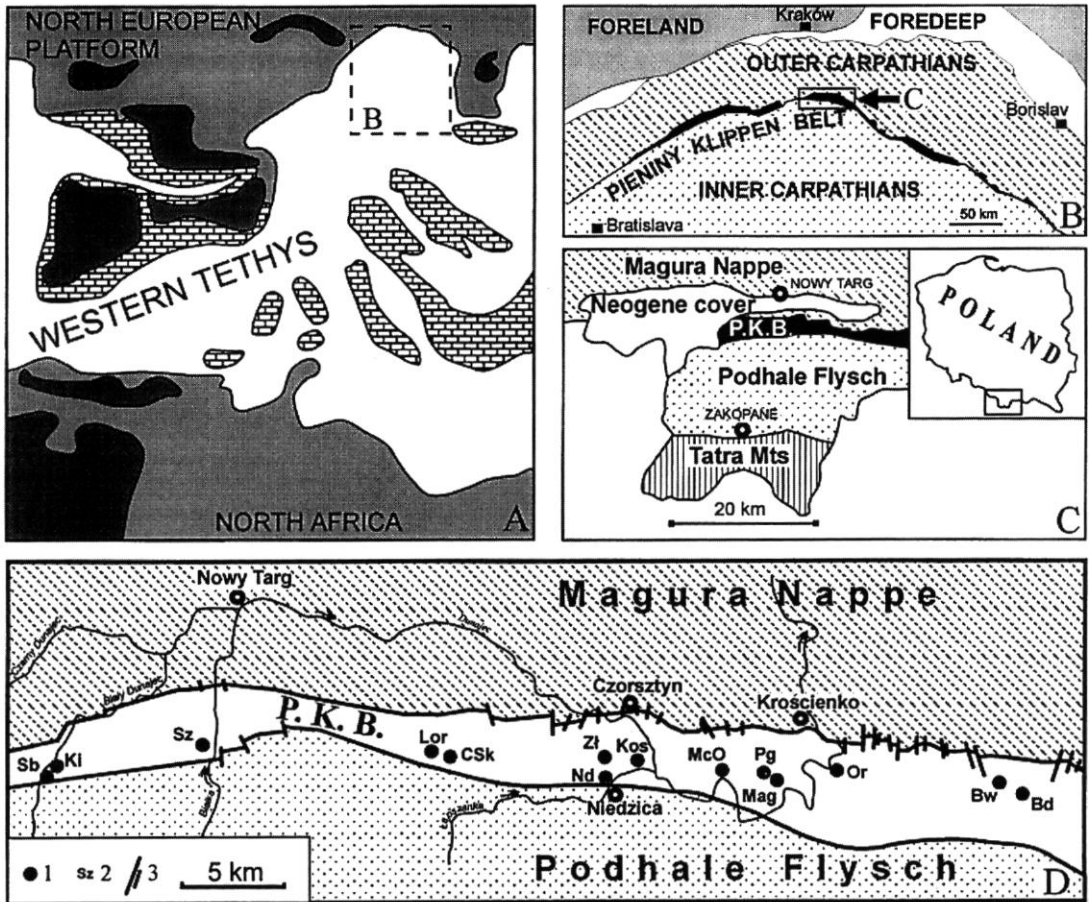
FIG. 1. — Location of the study area: A , in the Western Tethys (rectangle B) (map of late Cenomanian palaeoenvironments after Fourcade et al. 1993; simplified); B , C , in the Carpathians (Pieniny Klippen Belt in black); D , in the Pieniny Klippen Belt. Legend: 1, investigated outcrops; 2, symbols of outcrops; 3, more important dislocations. List of outcrops (from west to east): Sb , Stare Bystre; Ki , Kietowy stream; Sz , Szaflary quarry; Lor , Lorencowe Klippes; Csk , Czerwona Skala; Zi , Żłobowy Creek; Nd , Niedziczanka stream; Kos , Kosarzyska Valley; McO , Macelowa-Osice; Pg , Podskalnia Góra Mt; Mag , Magierowa Klippe; Or , Orlica Hill; Bw , Bukowiny Valley; Bd , Bukowiny Hill.
