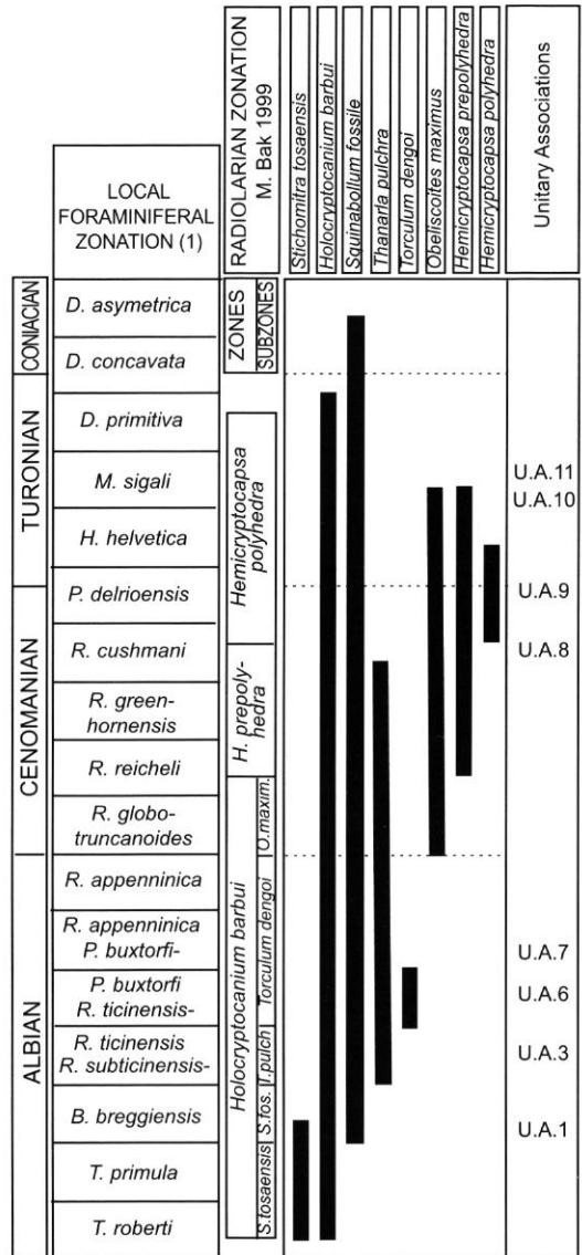
Fig. 3. — Occurrence range chart of index radiolarian species recorded in the Albian to Coniacian deposits in the Pieniny Klippen Belt successions, based on their first and the last appearances, and their co-occurrence based on the Unitary Associations. Abbreviations of zones: S. tosaensis , Stichomitra tosaensis ; S. fos. , Squinabollum fossile ; T. pulch. , Thanarla pulchra ; O. maxim. , Obeliscoites maximus . 1, local planktonic foraminiferal zonation after Robaszynski & Caron (1985) modified by K. Bąk (1992, 1998).
