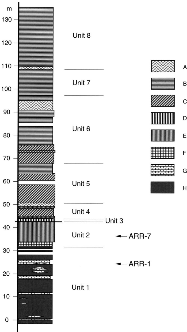
FIG. 3. — Summarized geologic column of the Arrow Rocks. A, fold zone; B, siliceous mudstone; C, bedded siliceous mudstone and chert; D, alternation of black shale and chert; E, bedded chert; F, tuff; G, limestone; H, spilitic basalt. ARR-1 and ARR-7 are the horizons where Permian radiolarians occurred (Takemura et al. 1998).
