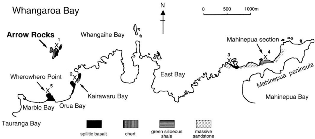
FIG. 2. — Permian and Triassic fossil localities in the Whangaroa Area. X, fossil localities, 1, Permian radiolarians from limestone and bedded chert at Arrow Rocks (Takemura et al. 1998 and this study); 2, Permian radiolarians from bedded chert at Kairawaru Bay (Caridroit & Ferrière 1988; Adachi 1988); 3, Permian radiolarians from limestone and chert at west of Mahinepua Peninsula (Takemura et al. 1998); 4, Triassic radiolarians from phosphate nodules in green argillite at the Mahinepua Section (Aita & Bragin 1999); 5, Permian fusulinids from limestones at Wherowhero Point (Hornibrook 1951; Leven & Grant-Mackie 1997).
