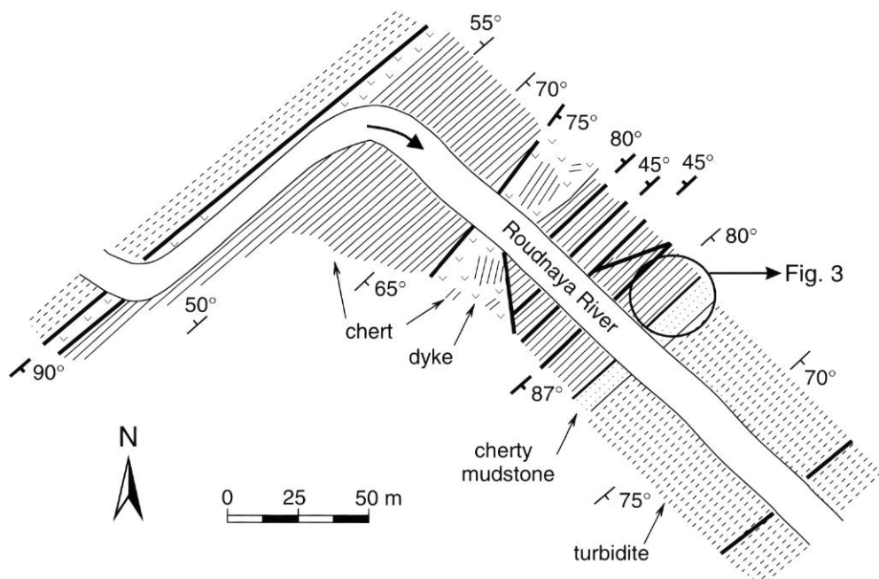
Fig. 2. — Geological scheme illustrating the structure of chert-terrigenous successions of the second tectonic plate along the Roudnaya River (Dalnagorsk Town).
