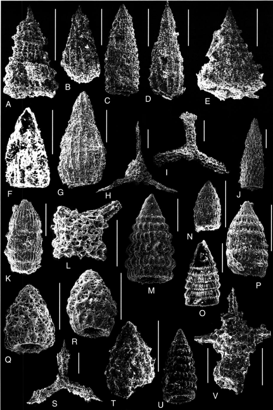
FIG. 5. — Some Jurassic and Early Cretaceous radiolarians from chert-terrigenous sequence of the Taukha Terrane. A , Parahsuum cf. longiconicum Sashida, P-17; B , Hsuum altile Hori & Otsuka, P-18; C , Parahsuum grande Hori & Yao, P-15; D , Hsuum sp. A, P-14; E , Parahsuum cf. hiconocosta Baumgartner & De Wever, P-14; F , Hsuum cf. mirabundum Pessagno & Whalen, P-13; G , Hsuum matsuokai Isozaki & Matsuda, P-8; H , Triactoma tithonianum Rust, P-7; I , Tritrabs cf. casmaliaensis (Pesagno), P-9; J , Transhsuum medium Takemura, P-8; K , Archaeodictyomitra minoensis (Mizutani), P-6; L , Haliodictya (?) cf. hojnosi Riedel & Sanfilippo, P-6; M , Pseudodictyomitra okamurai Mizutani, P-6; N , P , ? Pseudodictyomitra aff. Nuda Shaaf; N , P-6; P , P-4; O , ? Pseudodictyomitra aff. Leptoconica (Foreman), 86-14; Q , R , Xitus gifuensis Mizutani, P-3; S , Tritrabs simplex Kito & De Wever, P-10; T , Stichocapsa ex gr. altiforamina Tumanda, P-0; U , Pseudodictyomitra carpatica (Lozynyak), P-2; V , Cecrops sp., P-0. Scale bars: 100 \mu m.
