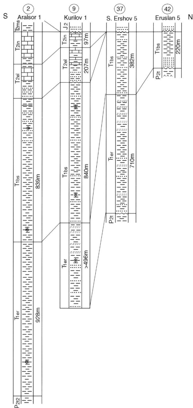
FIG. 9. — The Lower Triassic of the Precaspian Depression illustrated by some representative boreholes (Aralsor 1, 2 on Fig. 10; Kurilov 1, 9 on Fig. 10; South Ershov 5, 37 on Fig. 10; Erulsan 5, 42 on Fig. 10). Legend: see Fig. 6.
