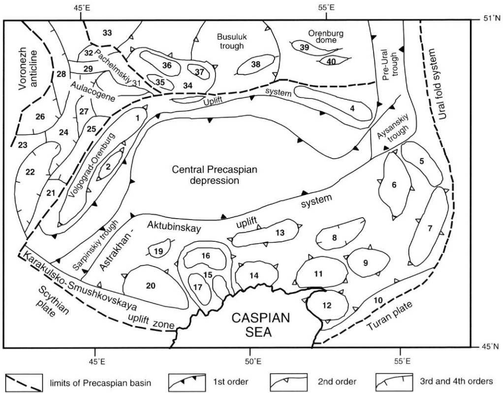
FIG. 1. — Tectonic chart of the Precaspian Depression. Tectonic features: 1, Akhtubinsk-Palassowski megamound; 2, Dzhanibekov rise; 3, Altatinsk-Nikolskiy mound; 4, Karachaganak-Koblandinskaya uplift; 5, Temirskiy dome; 6, Kyzylsharskiy dome; 7, Zharkamyskiy dome; 8, Dossorskiy trough; 9, Biikzhalskiy dome; 10, South Emba uplift; 11, Guriev dome; 12, Karaton-Tengiz uplift; 13, Zhaykyskiy dome; 14, North-Caspian dome; 15, Akkolskiy dome; 16, Myntobinskaya uplift; 17, Kobyakovskoe uplift; 18, Otyabarskoe uplift; 19, Azgirskae uplift; 20, Astrakhan dome; 21, Suvodskaya uplift; 22, Olkhovskaya depression; 23, Archedino-Don mound; 24, Zhirnovsko-Umetovskiy mound; 25, Antipovsko-Sherbakovskiy mound; 26, Tersinskaya depression; 27, Zolotovsko-Kamenskaya uplift; 28, Karamyshskaya uplift; 29, Elshano-Sergievskiy mound; 30, Stepnovskiy mound; 31, Voskresenskaya depression; 32, Saratov displacements; 33, Kazanlinskiy mound; 34, Pugachevskiy dome; 35, Marievskaya uplift; 36, Balakovskaya uplift; 37, Klintsovskaya uplift; 38, Kamelik-Chaganskiy mound; 39, Zemlyanskiy mound; 40, Syrtovskiy mound.
