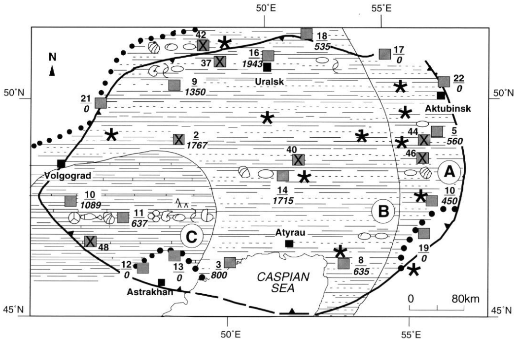
FIG. 10. — Lower Triassic lithological and palaeogeographical scheme of the Precaspian Depression. A , area of alluvial and proluvial deposits; B , alluvial plain, flooded episodically by the sea; C , epicontinental marine deposits. Legend: see Fig. 7. List of boreholes: 2, Aralsor; 3, Zhambay; 5, Karabulak; 8, Kulsary; 9, Kurilov; 10, Sadovaya; 11, Bugrin; 12, Stepnov; 13, Zavolz; 14, Ushtobe; 16, Chinarev; 17, Mertvye Soli; 18, Akzhar; 19, Tuskum; 21, Nikolaev; 22, Podgornen; 37, Ershov; 40, Inder; 42, Eruslan; 44, Kenkiyak; 46, Biaktykol; 48, Shar-Tsaryn.
