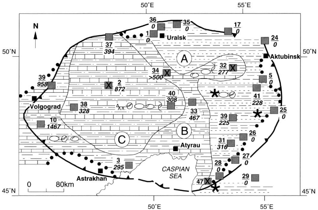
FIG. 12. — Upper Triassic lithological and palaeogeographical scheme of the Precaspian Depression. A , alluvial plain, flooded episodically by the sea; B, C , carbonate-clastic ( B ) and clastic-carbonate ( C ) deposits of shallow epicontinental sea. Legend: see Fig. 7. List of boreholes: 1, Vetekin; 2, Aralsor; 3, Zhambay; 5, Karabulak; 10, Sadovaya; 17, Mertvy Soli; 24, Jusa; 25, Zhanazhol; 26, Chikembay; 27, Mashly; 28, Suishbek; 29, Chumyshty; 31, Zhusalysay; 32, Chobda; 33, Matenkozka; 34, Kusankuduk; 35, Pavlov; 36, Teplov; 37, Ershov; 38, Shungay; 39, Novonikol; 40, Inder; 41, Shubarkuduk; 47, East Provra.
