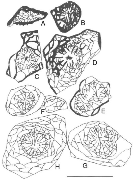
FIG. 8. — Petalaxis ( P. ) vesiculosus group: A-D , Petalaxis ( P. ) vesiculosus (Dobrolyubova), N 27/140 museum PINRAN, Moscow Basin, Ruza-Ojigova, right bank of Moscow River, down stream from Novaya Ruza, loc. XXVI, bed 3, Moscovian Stage, Myachkovian substage; E-H , Petalaxis ( P. ) gigas Kossovaya n.sp., N 32-9-3a/3 CNIGR museum, St Petersburg, Russia, Northern Timan, Sula River section, loc. 32, bed 9, Moscovian stage, Myachkovian substage. Scale bar: 1 cm.
