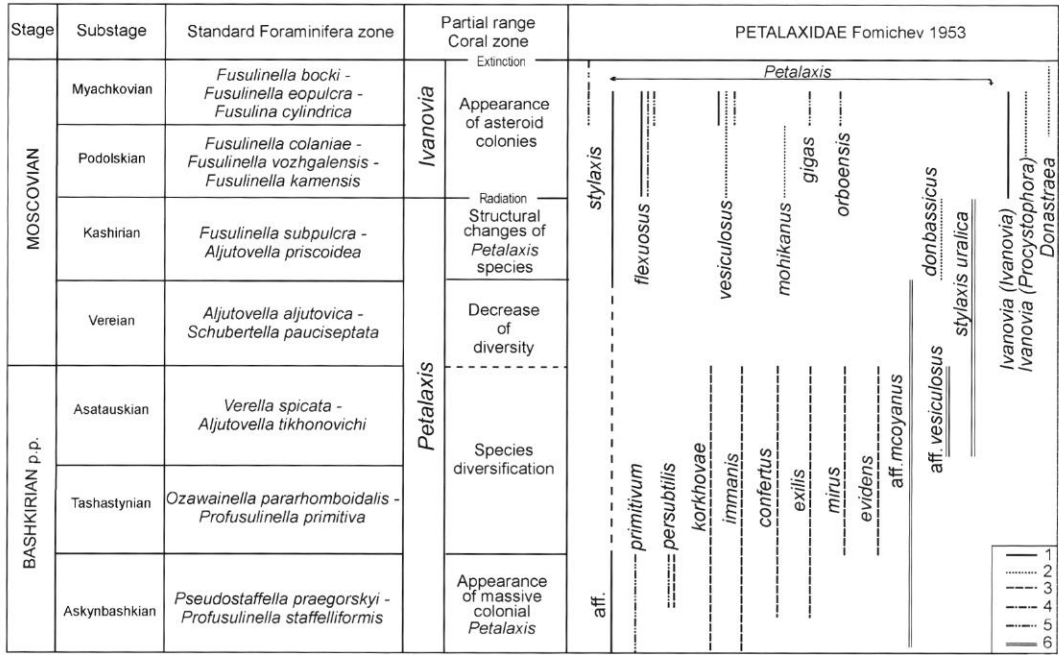
Fig. 5. — Distribution and stratigraphic range of Petalaxis and Ivanovia species in the Bashkirian and Moscovian deposits of the western part of Russia. 1, Moscow Basin; 2, Donetsk Basin; 3, Voronezh anticline; 4, Nova Zemlya; 5, Northern Timan; 6, Gornaya Bashkiria. N.B. Early Bashkirian substages omitted (see Fig. 6).
