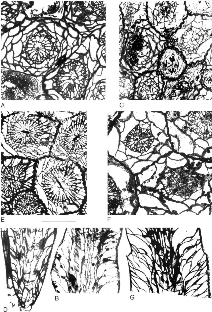
FIG. 13. — A, B , Petalaxis ( P. ) vesiculosus (Dobrolyubova), N 32-9-3a/3 CNIGR museum, Northern Timan, Sula River section. loc. 32, bed 9, Sula Formation, Myachkovian substage, (A) transverse section, (B) longitudinal section; C, D , Petalaxis ( P. ) stylaxis (Trautschold), N 32-9-4a/1 CNIGR museum, Northern Timan, Sula River section. loc. 32, bed 9, Sula Formation, Myachkovian substage, (C) transverse section, (D) longitudinal section; E , Petalaxis ( P. ) flexuosus (Trautschold), N 5-6-1 CNIGR museum, Northern Timan, Belaya River section, loc. 5, bed 9, Sula Formation, Myachkovian substage; F, G , Petalaxis ( P. ) gigas Kossovaya n.sp., N 32-9-4a/2, Northern Timan, Sula River section. loc. 32, bed 9, Sula Formation, Myachkovian substage, (F) transverse section, (G) longitudinal section. Scale bar: 0.5 cm.
