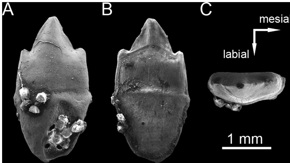
Fig. 4. Specimen KM-?-1, tooth of cf. Cynodontia gen. et sp. indet., in (A) labial, (B) lingual and (C) occlusal views. SEM views.
