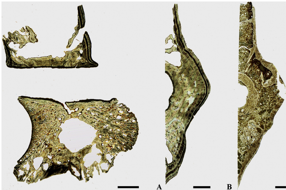
Fig. 11. Pterosphenus schucherti . Georgia, USA. Late Eocene. MNHN Unnumb. A. Longitudinal section in NL. The scale bar equals 3 mm. B–C. Half transverse sections in NL. B, MNHN Unnumb. A ; C, MNHN Unnumb. B. The scale bars equal 2 mm.
