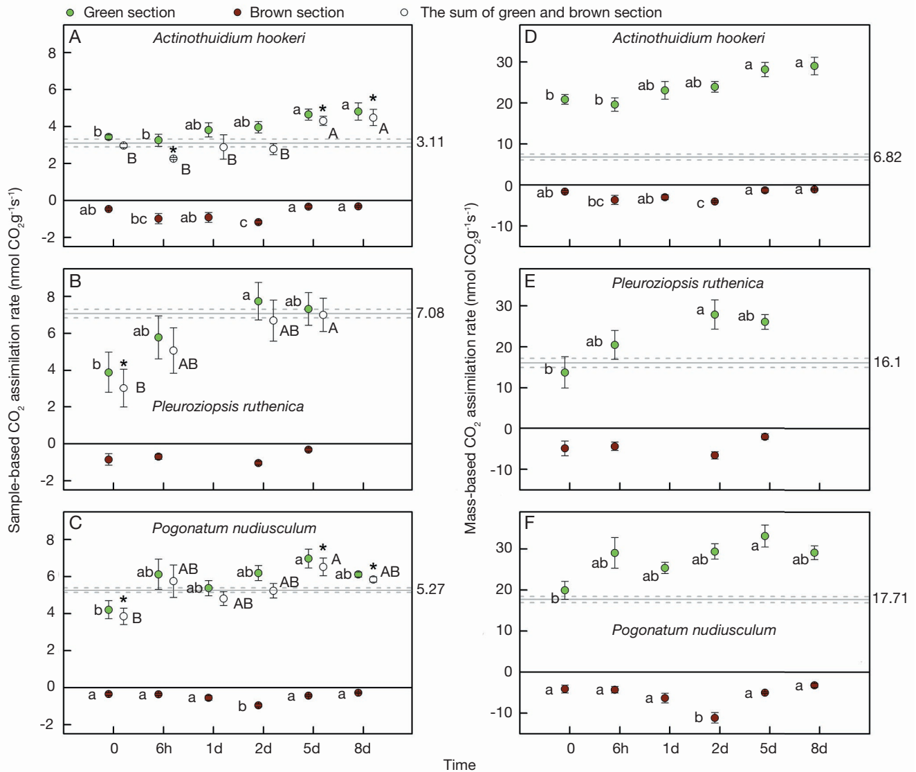
FIG. 2. — Comparisons of the sample- (A–C) and mass- (D–F) based CO 2 assimilation rates of green and brown moss sections, and the sum of these two sections (sample-based plots) and the changes through time for three moss species. Shown are the mean values \pm standard errors (smaller than the symbol in some cases) of different sections determined at different time points, starting at a few minutes after separation. Sample-based plots are expressed as the CO 2 exchange per sample to allow a direct comparison of intact and separated sections. Gray solid and dashed lines show the mean values of intact shoots (values shown to the right), \pm standard errors. Asterisks indicate significant differences in assimilation rates between intact shoots and the sum of the separated sections (paired t-test, p < 0.05 , n = 4 ). And the capital and lowercase letters indicate significant differences among time points ( p < 0.05 ).
