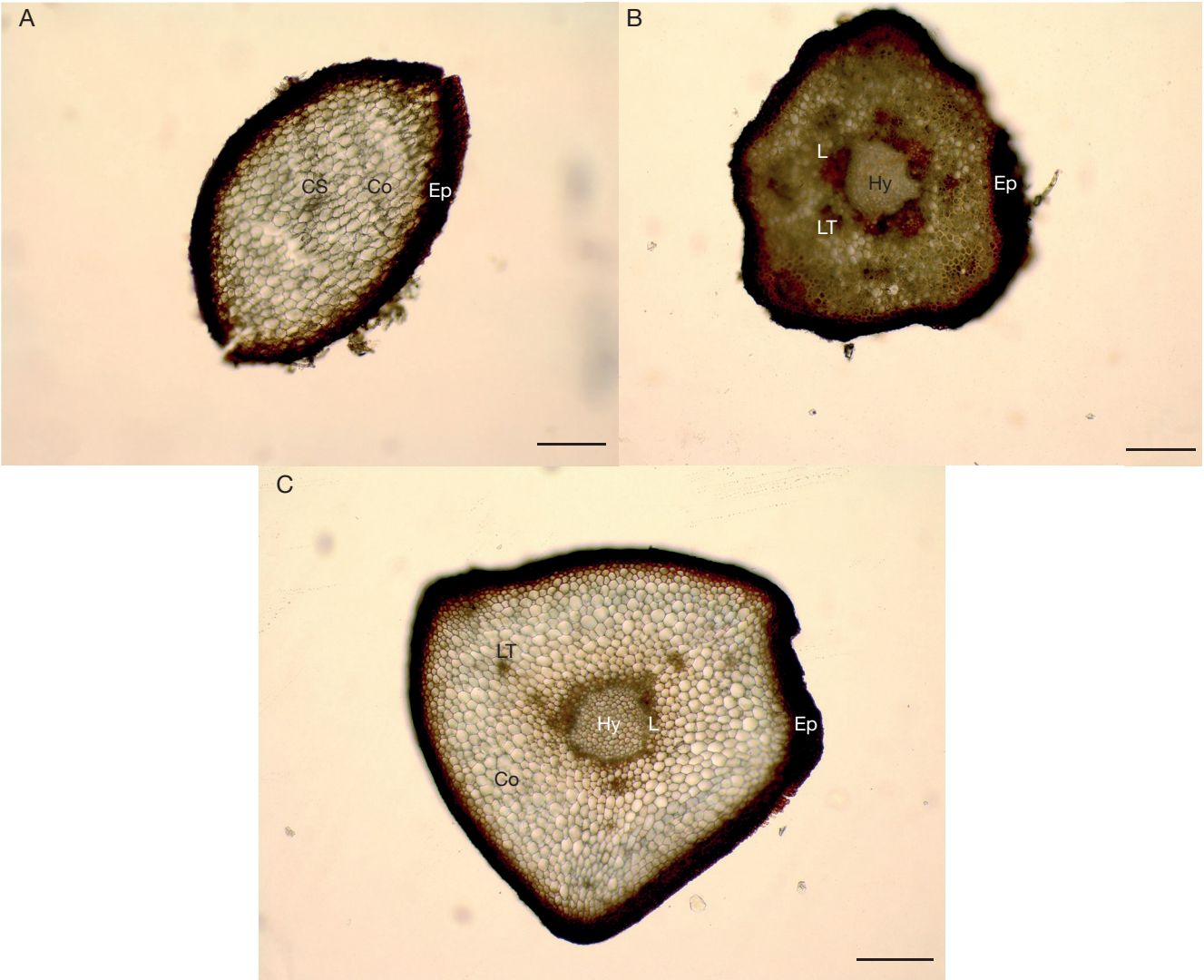
APPENDIX 2. — A , Actinohuidium hookeri (Mitt.) Broth.; B , Pleuroziopsis ruthenica (Weinm.) Kindb. ex E. Britton; C , Pogonatum nudiusculum Mitt. The stem cross-sections of the three mosses collected on the eastern slope of Gongga Mountain, Sichuan province, China. One medium-sized individual from each replicate was selected to observe the stem cross-section. The samples were submerged in a petri dish for 30 minutes and the excess water was removed using a paper towel. The stem cross-section was made at the point where the brown and green sections were separated (Fig. 1) using a dissecting microscope and was photographed using an optical microscope. The cross-section anatomical structures following Maslova et al. (2015). Abbreviations: Co , cortex; CS , central strands; Ep , epidermis; Hy , hydroids; L , leptoids; LT , leaf trace.
