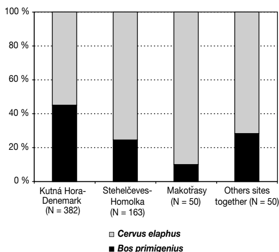
FIG. 4. – Comparison of aurochs representation with stag in Kutná Hora-Denemark and on other Tzech Eneolithic sites. Finds of uncertain morphological determination of form ( Bos sp.) not included. Y axis = % NISP.
