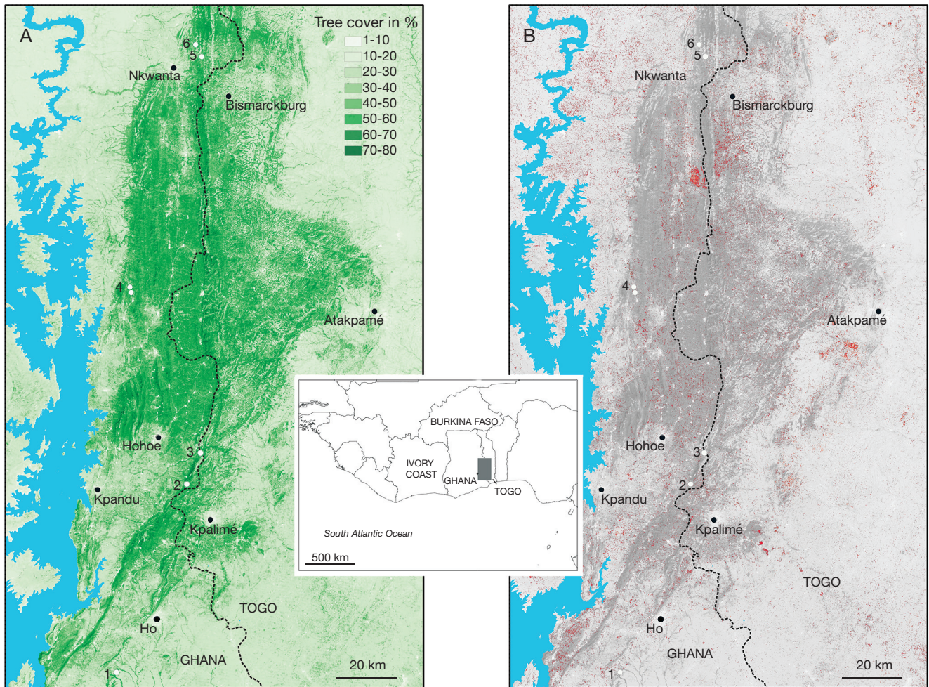
FIG. 1. — Maps of Volta Region, Ghana with the Togo Highlands: A , forest cover > 30% in 2010 and study sites: 1, Kalakpa Resource Reserve; 2, Tagbo Falls (Liatí Wote); 3, Wli Waterfall (Agumatsa Valley); 4, Apesokubi (Bedibem Forest); 5, Shiare village; 6, Kyabobo Range National Park (KRNP); B , elevation (shading), Forest cover loss 2000–2018 (red pixels) based on online data (Hansen et al. 2013).
