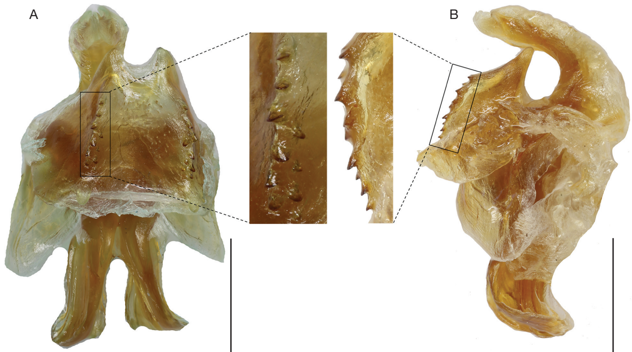
FIG. 97. — Phallic complex of Paracinipe saharae (Pictet & Saussure, 1891), dorsal view (A), lateral view (B). Scale bars: 1 mm. Photos: H. Tlili.
