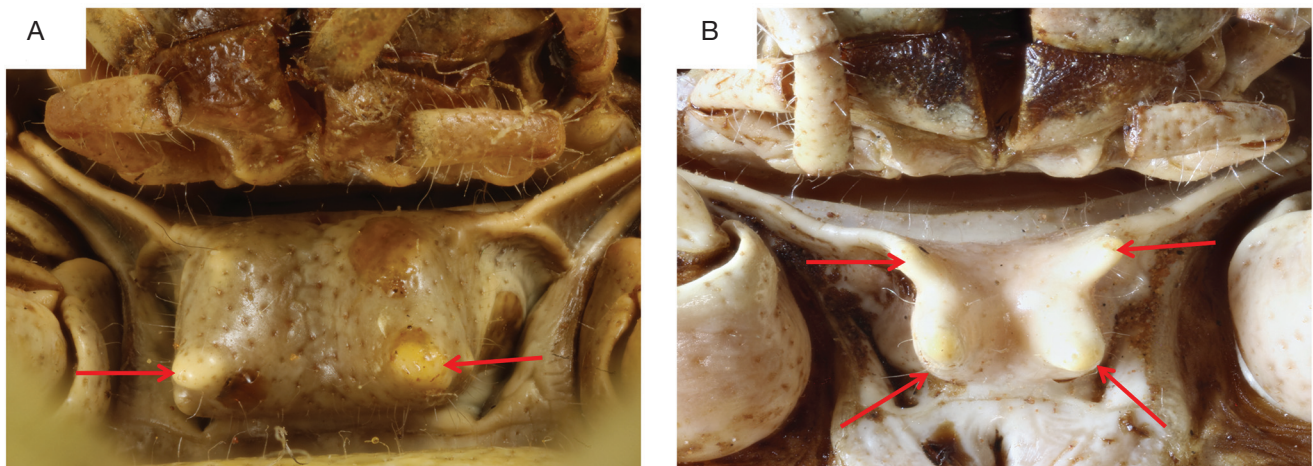
FIG. 83. — Shape of prosternal process: A , prosternal process of Euryparyphes sitifensis (Brisout de Barneville, 1854) (female) with two pointed tubercles; B , Paraeuryparyphes quadridentatus (Brisout de Barneville, 1852) (female) with four pointed tubercles. Scale bars: 2 mm. Photos: H. Tlili.
