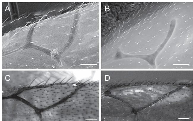
FIG. 9. — Types of radial cells: A , A. trapezoidea (Hartig, 1841); B , D. subclavata Förster, 1869; C , P. villosa (Hartig, 1841); D , P. americana Baker, 1896. Scale bar: 50 µm.
