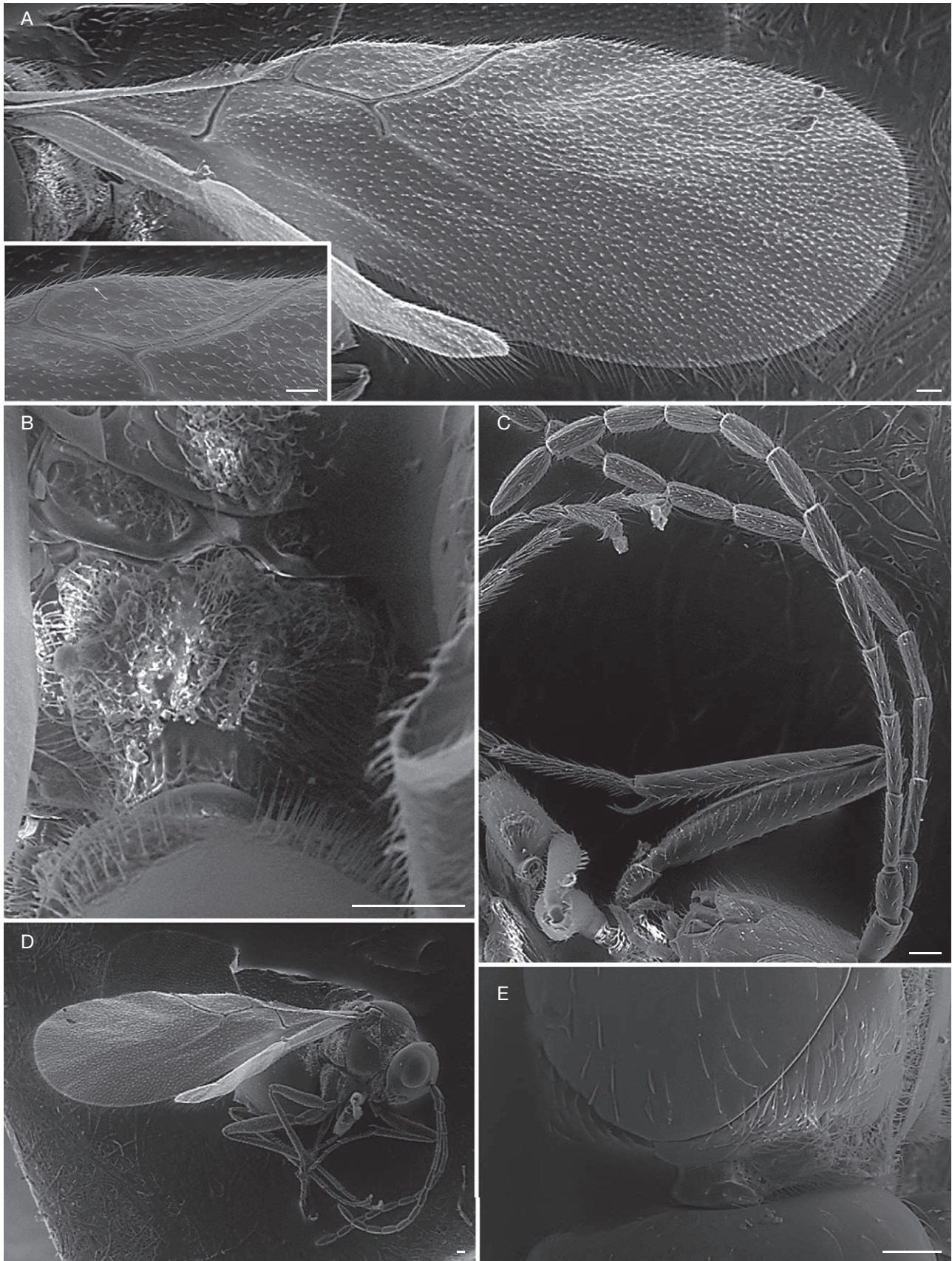
FIG. 4. — Alloxysta alpina Ferrer-Suay & Pujade-Villar, n. sp.: A , Forewing; B , propodeum; C , antennae; D , body; E , pronotum. Scale bars: 50 µm.
