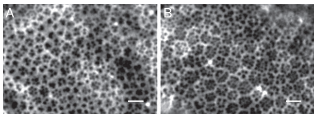
FIG. 3. — Echiniscus pardalis n. sp., details of subsurface structure of plates, holotype, PhC: A, scapular plate; B, caudal plate. Scale bars: 2 µm.
