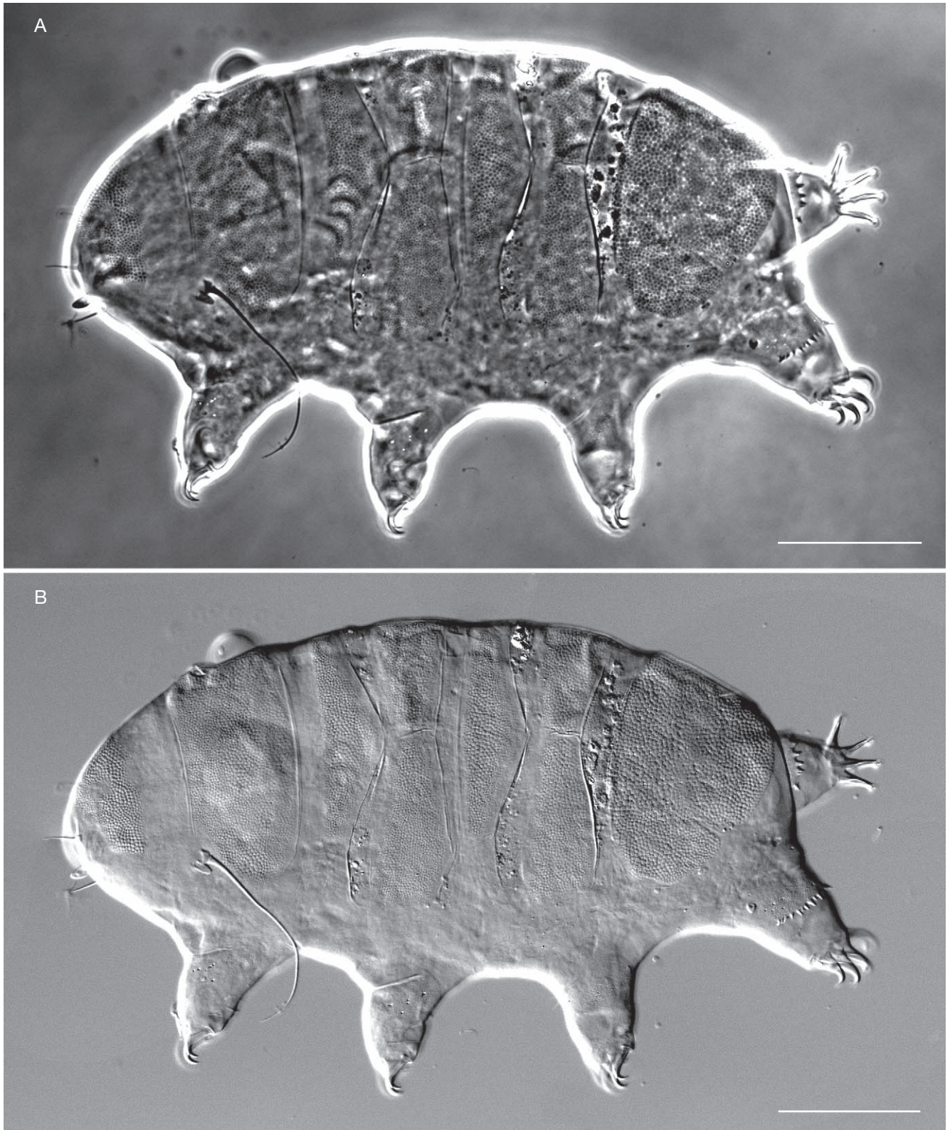
FIG. 1. — Echiniscus pardalis n. sp., habitus of holotype: A , PhC; B , DIC. Scale bars: 50 µm.
