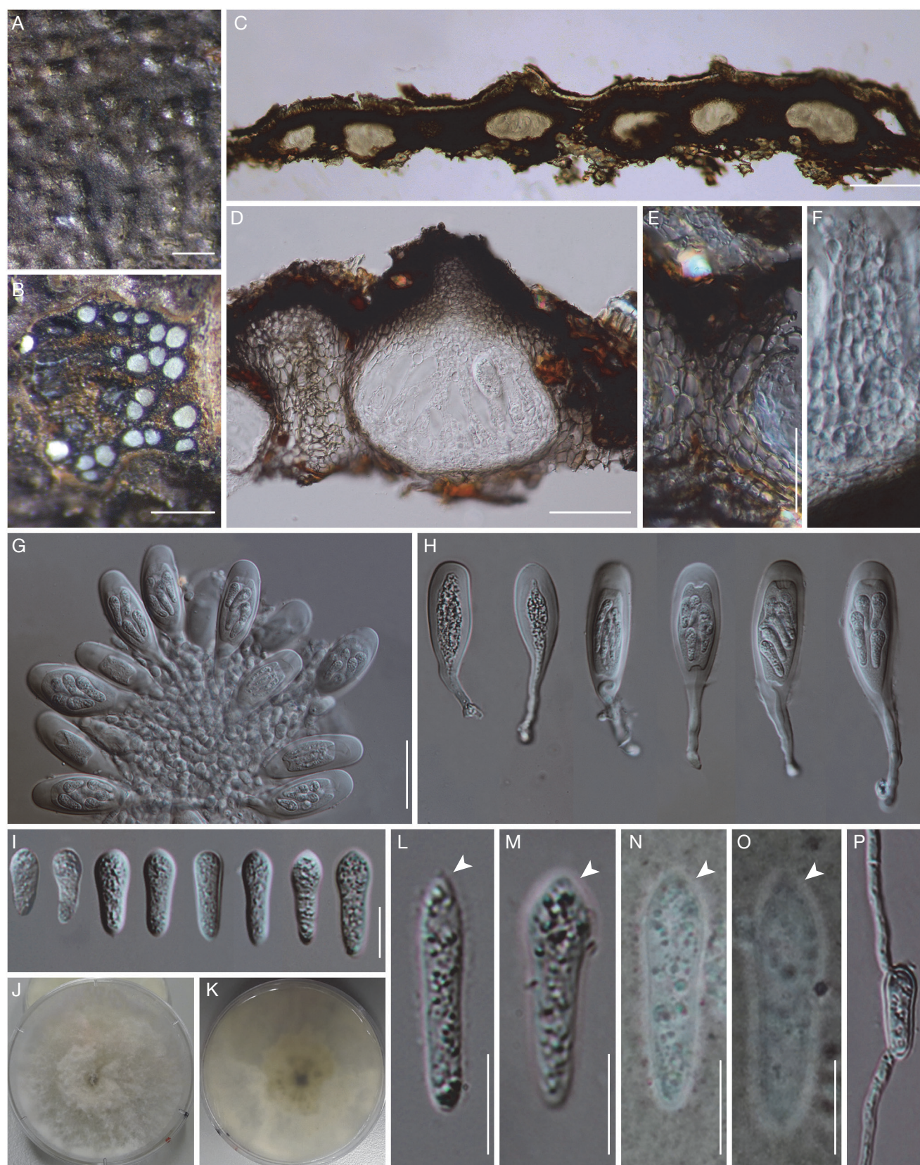
FIG. 3. — Pseudofusicoccum adansoniae Pavlic, T.I.Burgess & M.J.Wingf. (MFLU 19-0239): A , habit of ascoma in bark; B , transverse sections through ascomata; C , D , section through the ascoma; E , peridium; F , pseudoparaphyses; G , H , asci; I , ascospores (mounted in double-distilled water); J , K , upper and reverse view of the culture after ten days; L – O , ascospores with mucilaginous sheath (arrows) (stained in Indian ink); P , germinated spores. Scale bars: A , B , 500 µm; C , 200 µm; D , 50 µm; E – H , 30 µm; I , L – P , 10 µm.
