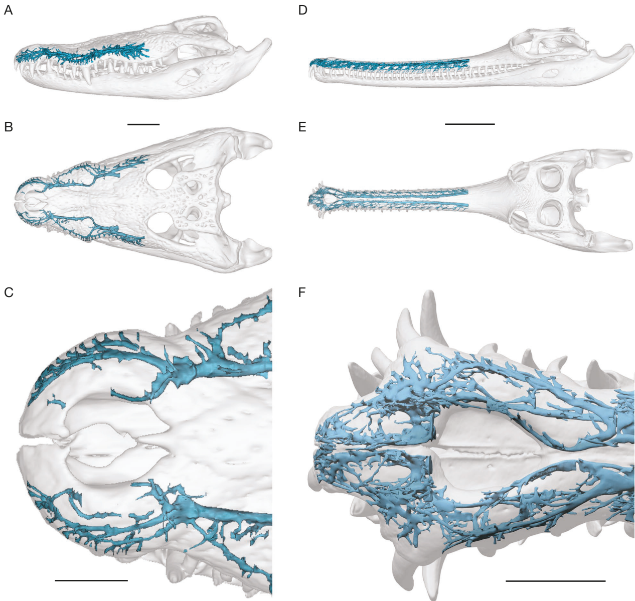
FIG. 19. — CT scans views of two crocodylians rostra in transparency with configuration of the neurovascular network: A-C , Crocodylus moreletii Duméril & Bibron, 1851 (TMM M-4980) in lateral left ( A ) and top ( B ) views with network highlighted in the rosette ( C ); D-F , Gavialis gangeticus Gmelin, 1789 (MHNG S14.25) in lateral left ( D ) and top ( E ) views with network highlighted in the rosette ( F ). Models by Frédéric Pittet and Florent Goussard. Scale bars: A, B, D, E, 10 cm; C, 5 cm; F, 2.5 cm.
