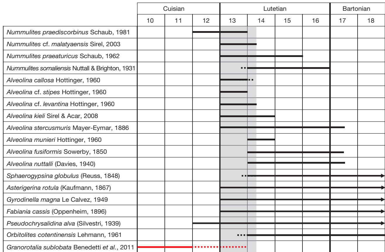
Fig. 5. — General biostratigraphic distribution of the studied species in Karyağı Hill and Gölbayırı section from Memlik Village. The grey area represents the stratigraphic position of the studied samples according to the assemblage biozone. Dotted lines show the suggested distribution of the species in the studied area.
