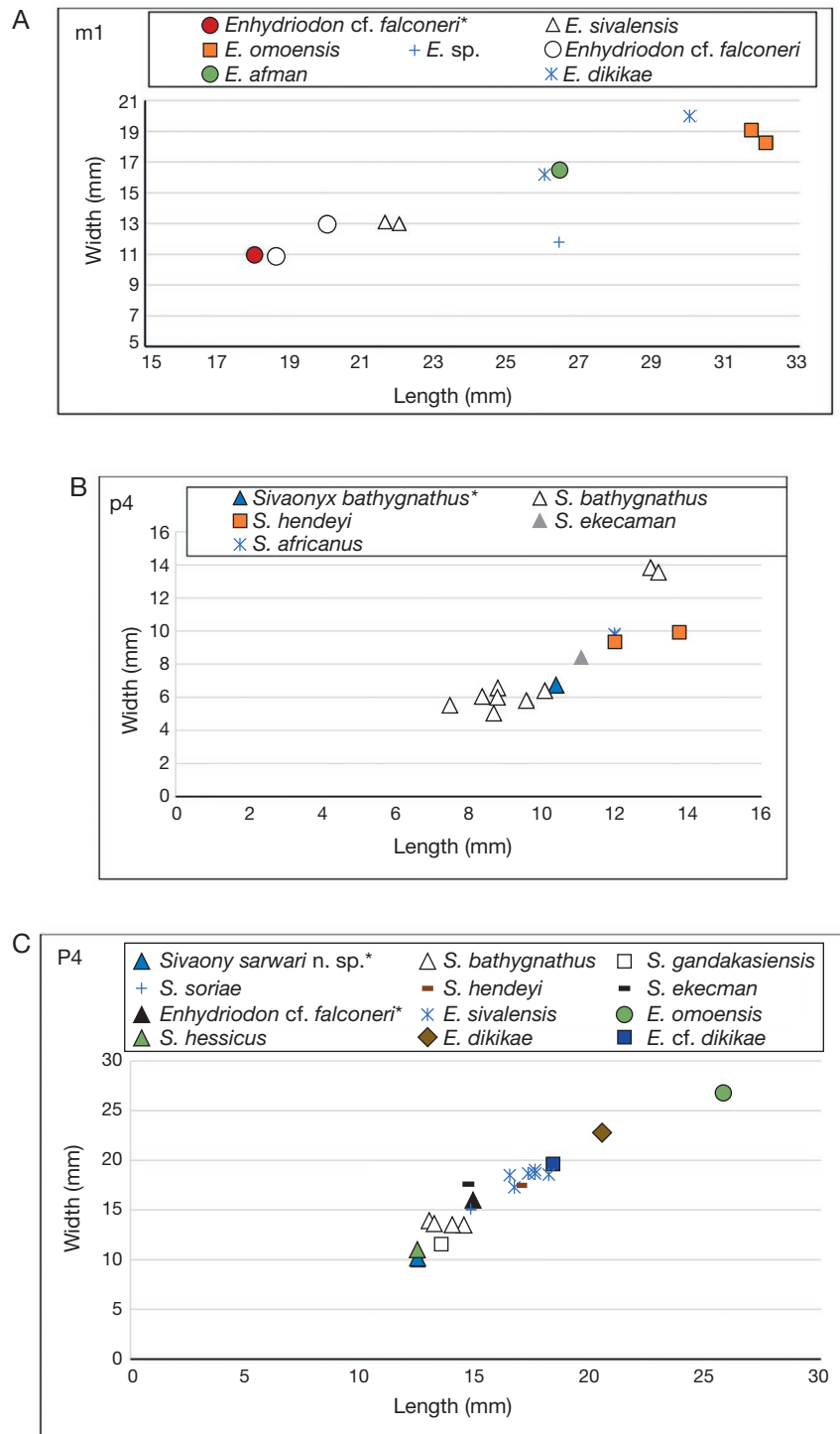
FIG. 3. — Comparative measurements of described taxa represented in scatter plots: A , Enhydriodon cf. falconeri ; B , Sivaonyx bathygnathus ; C , Sivaonyx sarwari n. sp.
