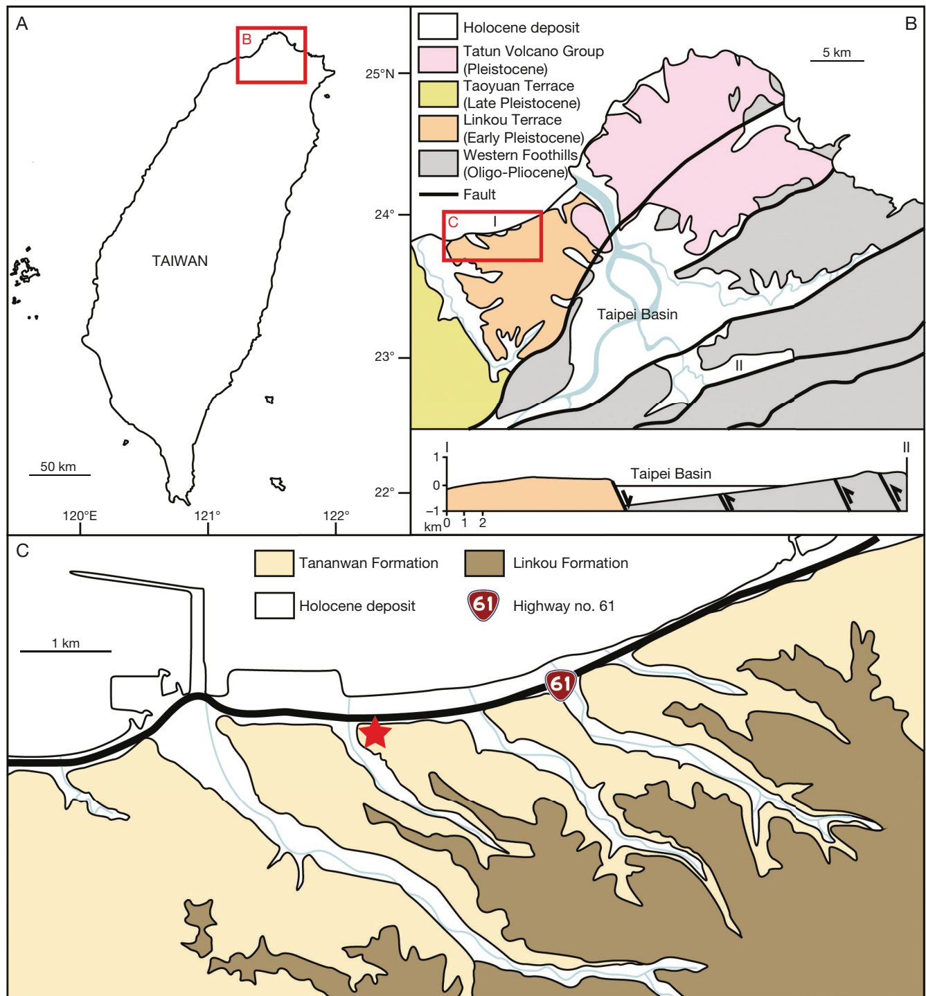
FIG. 1. — Locality and geological background of sampling site: A , study area; B , general geological background and sections of Taipei Basin (modified from Teng 2007); C , geological map of sampling site (modified from Lin 1981). Red star represents the sampling site. Map: Chia-Hsin Hsu.
