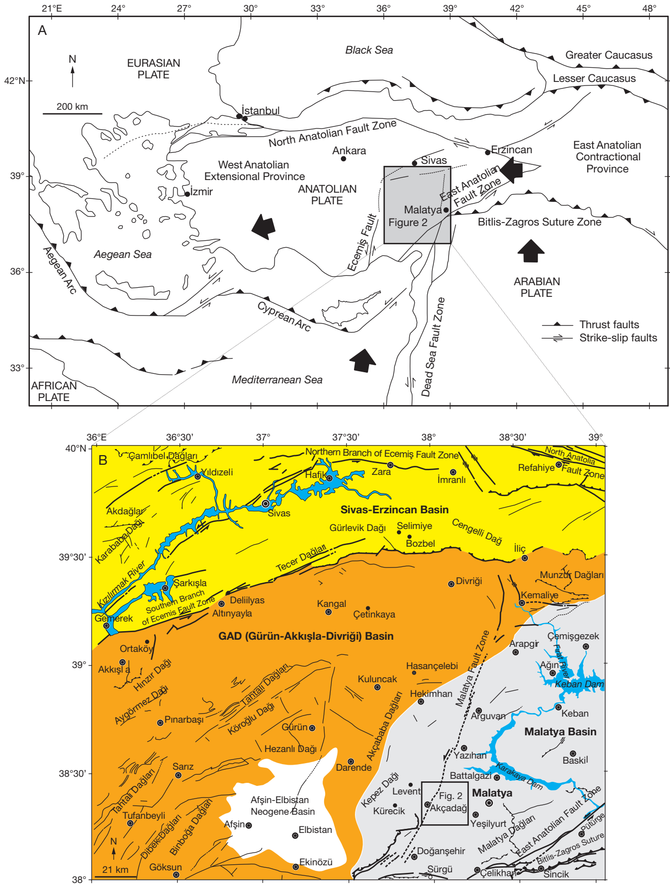
FIG. 1. — A , Tectonic map of Turkey showing the major tectonic structures (modified from Bozkurt 2001); B , limits of the Sivas-Erzincan, GAD (Gürün-Akışla-Divriği) and Malatya basins.
