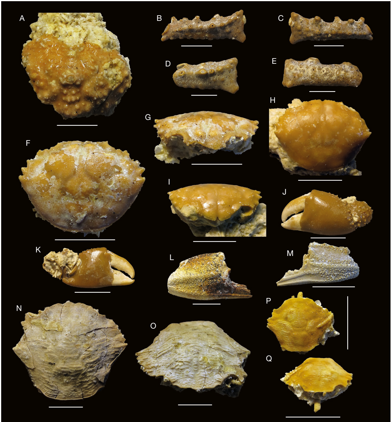
FIG. 5. — Decapods from the 'Savignean facies' (Langhian) of the 'Blandinerie' quarry, Breil (Maine-et-Loire): A , indeterminate majoid, ULB-IV-A (26): dorsal view; B-E , Derilambrus cf. szabo (Müller, 1974): B , ULB-IV-A (33), right propodus, outer margin; C , inner margin; D , ULB-IV-A (35), right propodus, outer margin; E , right propodus, inner margin; F-K , Pilumnus mediterraneus (Lorenthey, 1897): F , ULB-IV-A (14), dorsal view; G , frontal view; H , ULB-IV-A (18), dorsal view; I , frontal view; J , ULB-IV-A (20), left chela, outer margin; K , inner margin; L-M , undetermined Carcinidae: L , ULB-IV-A (52), right chela; M , ULB-IV-A (50) left chela; N-Q , Liocarcinus kuehni (Bachmayer, 1953a): N , ULB-IV-A (10), dorsal view; O , frontal view; P , ULB-IV-A (13), dorsal view; Q , frontal view. Scale bars: A-I, N-Q, 5 mm; J-M, 10 mm. Photographs by Á. Ossó.
