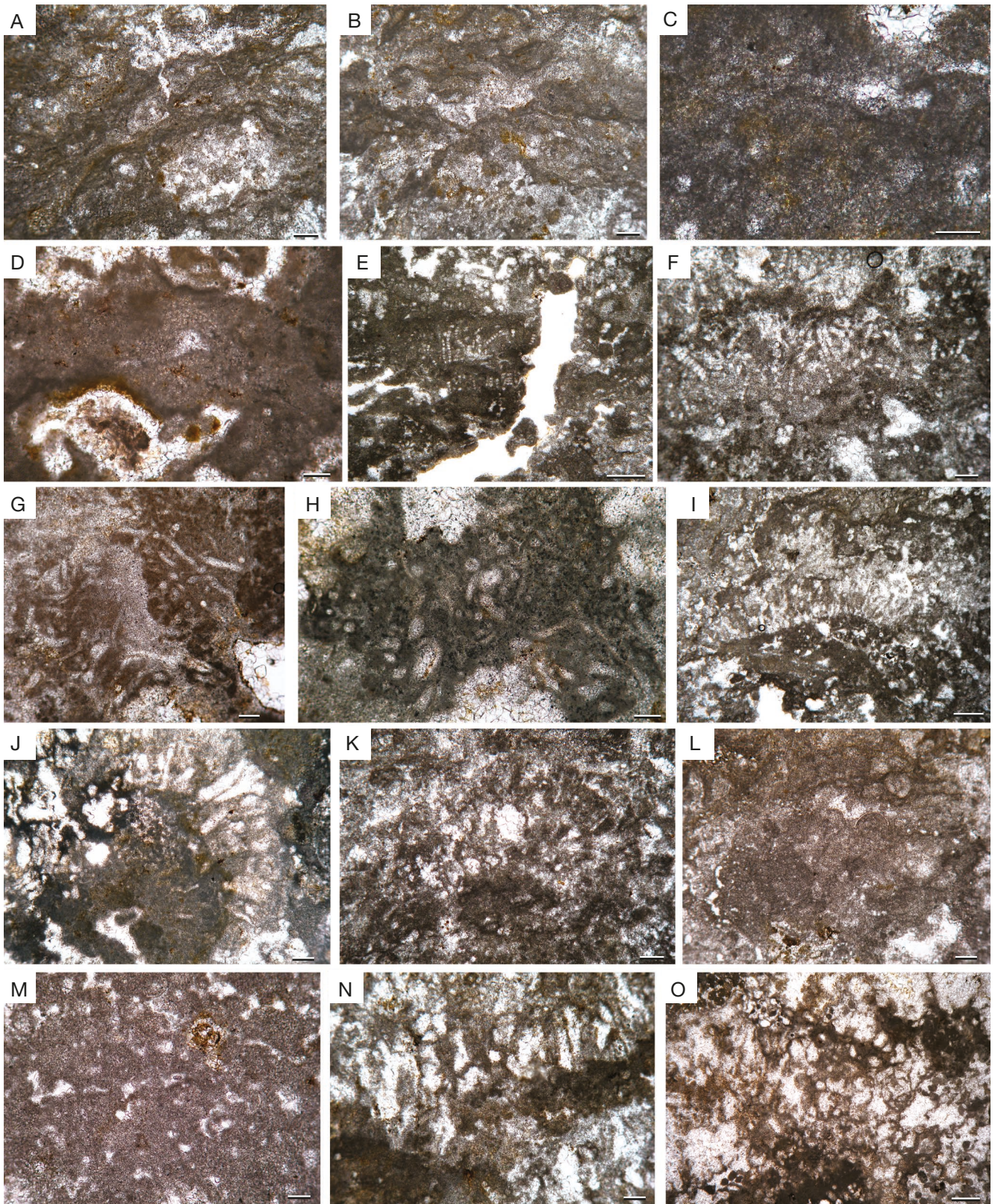
FIG. 9. — Main components of crusts: A, B , type 1, thin crust attributable to corallines; C, D , type 2, micritic masses attributable to corallines showing a preserved cellular structure; E, F , type 3, cell alignments within a micritic crust with an indistinctly fine structure, possibly attributable to Corallinaceae; G, H , type 4, networks of filaments with micritic outlines within micritic masses, recalling a cyanobacterial structure of the Girvanella type; I, J , type 5, elongated cell structures, sometimes branched; K , type 6, rounded micritic masses with fine fan-shaped filaments recalling small cyanobacterial constructions; L, M , type 7, lumpy micritic clumps of probable microbial origin; N, O , type 8, cellular structures of variable size exhibiting a Bacinella -like character. Scale bars: A, F, J–L, 200 \mu\text{m} ; B–D, G, H, M, N, 100 \mu\text{m} ; E, I, O, 500 \mu\text{m} .
