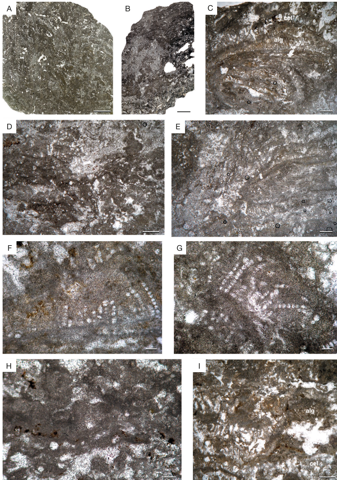
FIG. 11. — GR3 microfacies: A, B , general views showing dense micritic crusts, often forming small columns; C , detail of a multi-component crust: probable algae (type 3) with alignments of large cells ( alg ) and type 5 cell structures ( cel ) erected on the previous algal crust; D, E , mass formed by successive fine crusts (type 1) and rows of cells (type 3); F, G , detail of the rows of algal cells (type 3); H , lumpy micritic masses of microbial origin (type 7); I , composite crust with fine algal crusts (type 1), rows of cells (type 3, alg ), cellular structures (type 5, cel ). Scale bars: A, B, 5 mm; C, D, I, 500 \mu m; E, 400 \mu m; F-H, 100 \mu m.
