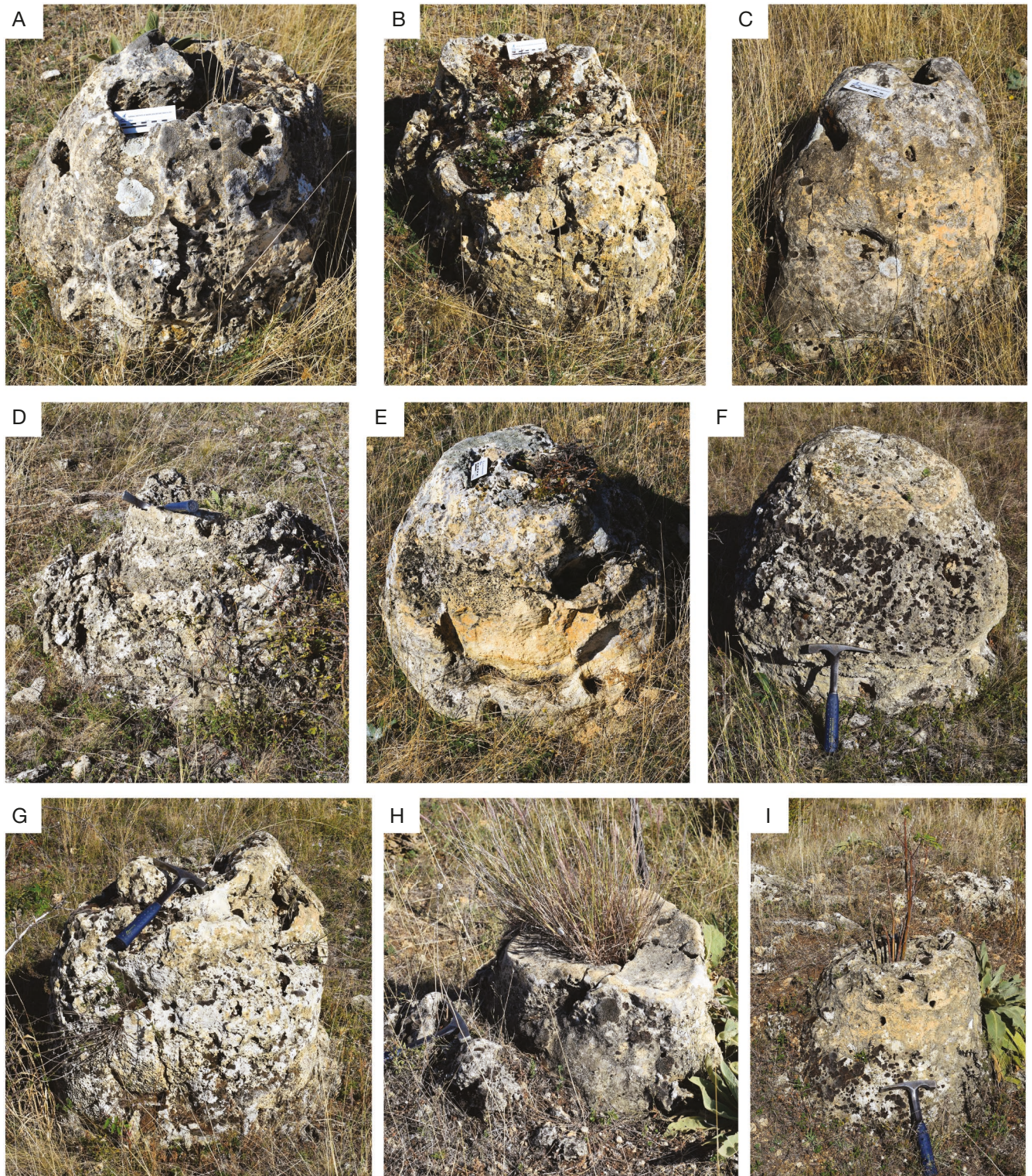
Fig. 6. — A-I , Vertically arranged cylinders in natural position; F , preserved dome shaped in form of “hat”; note the position of the central cavity; Scale bars: A-C, E: 10 cm; D, F-I: the hammer gives the scale.
