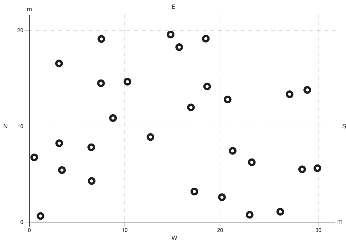
Fig. 16. — Spatial distribution of cylinders remaining in situ from zone 1, giving an idea of their density on the field.
