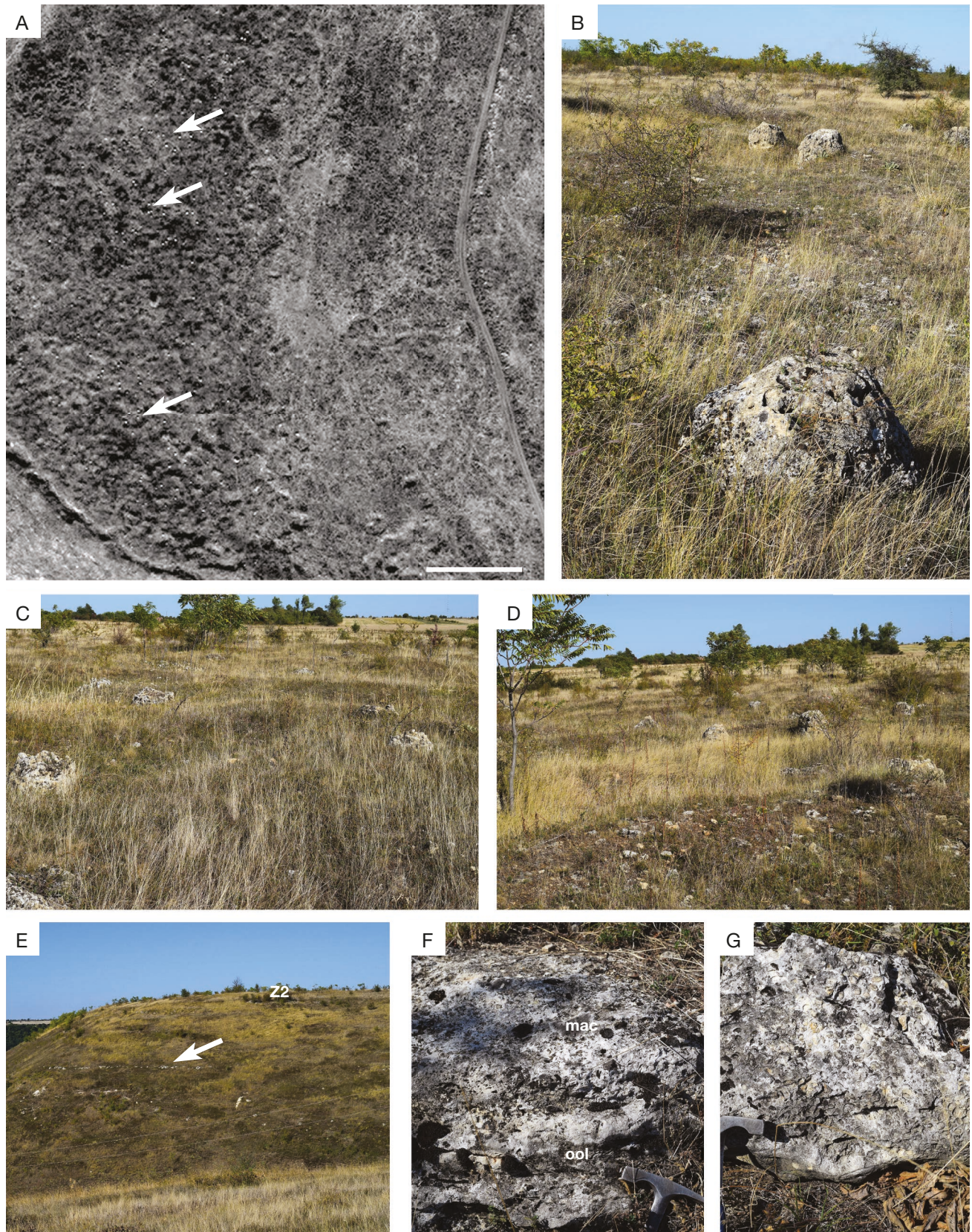
FIG. 4. — A , Satellite view of zone 2; the white dots represents the cylinders (the white arrows indicate the place of some cylinders); B-D , Cylinders in natural vertical position; B , Example of cylinder exhibiting a preserved dome shaped in form of "hat"; E , View of the outcrop under the zone 2 (Z2) with horizontal limestone beds indicated by the white arrow; F , Detail of the outcrops directly below the cylinder zone; it displays the oolitic limestone ( ool ) topped with Mactra limestone ( mac ); G , Detail of the limestone with accumulations of Mactra . Scale bar: A, 50 m; F, G, the hammer (length: 28 cm) gives the scale.
