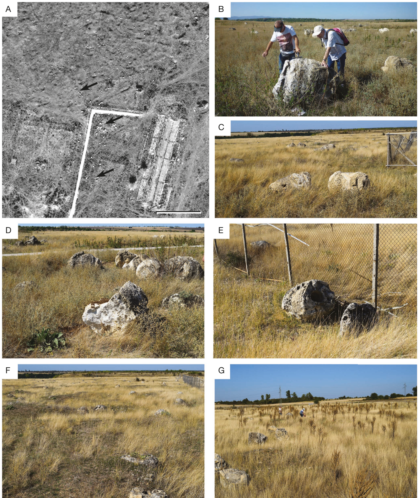
FIG. 3. — A , Satellite view of zone 1; the white dots represent the cylinders; B-E , Cylinders artificially displaced and horizontally arranged; F, G , Cylinders in vertical position, probably in their natural place. Scale bar: A, 50 m.
