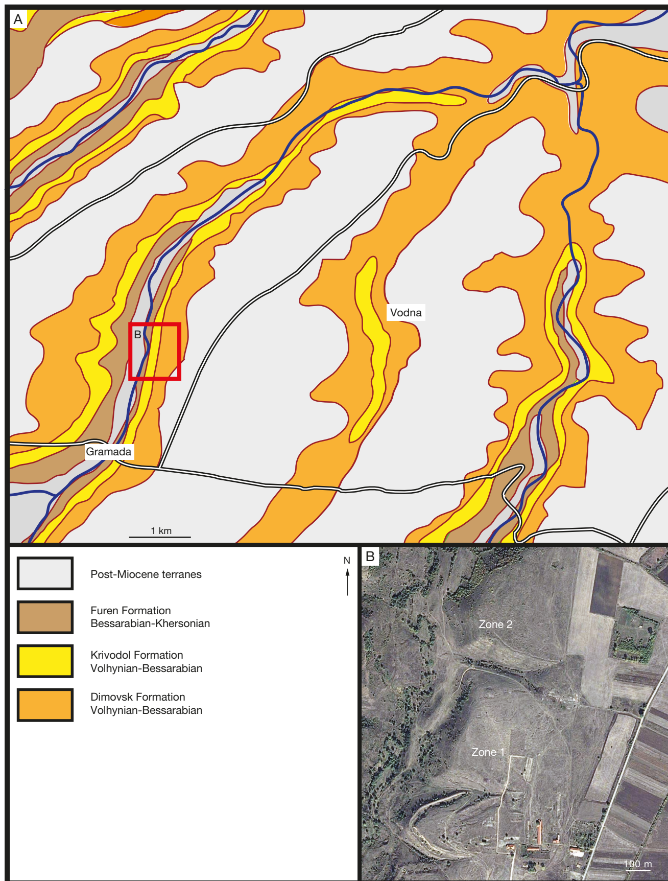
FIG. 2. — A , Geological map of the studied area; B , Satellite view of the outcrops to the north of the locality of Gramada and location of the two main zones exhibiting the calcareous cylinders.
