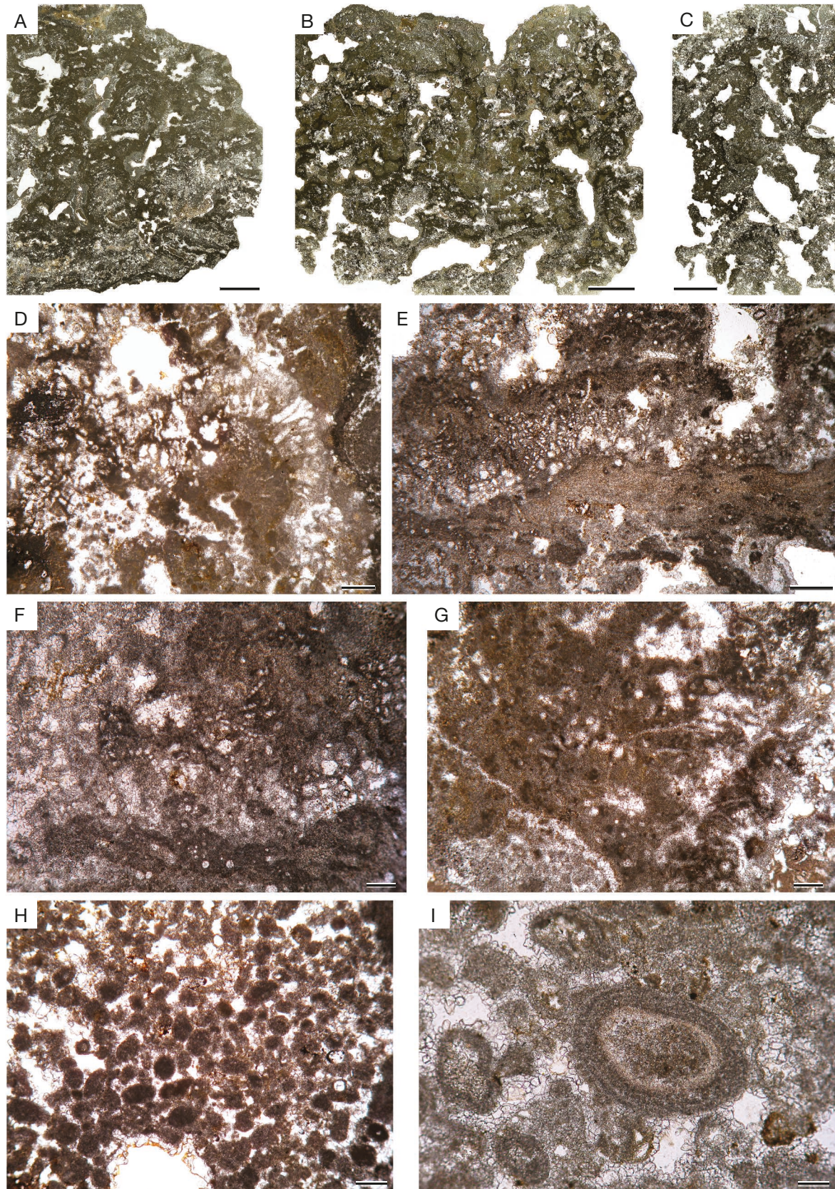
FIG. 14. — GR4 outer layer microfacies; A-C , general views showing the appearance in micritic columns making spaces partially filled by peloidal and oolitic accumulations; D , filamentous crusts surrounded by elongated branched cellular structures (type 5); E , composite corallineous crusts (types 2 and 3); F , cellular crusts (type 3); G , crust with Girvanella -like filament; H , accumulations of peloids resembling faecal pellets; I , details of grains with an oolitic cortex. Scale bars: A-C, 5 mm; D, E, 500 \mu m; F-H, 200 \mu m; I, 100 \mu m.
