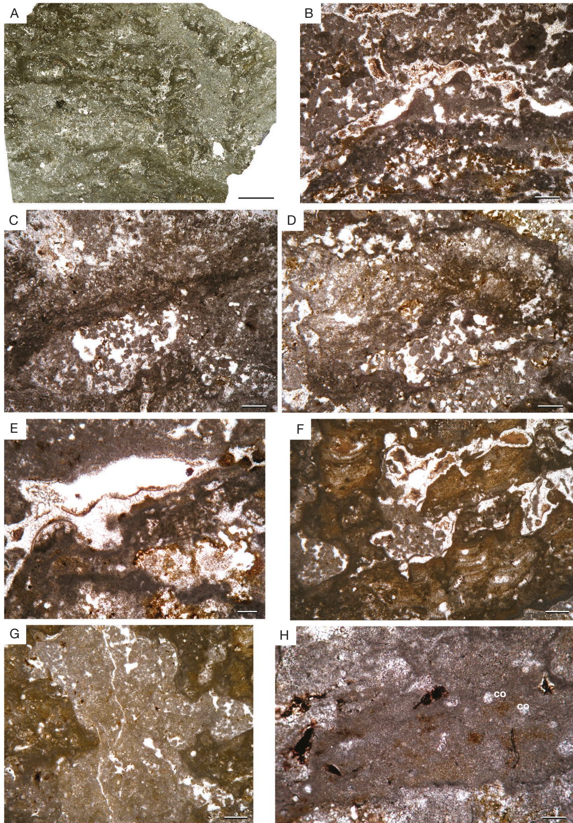
FIG. 13. — GR4 middle part microfacies; A , general view showing crusts forming more or less wide columns, the spaces between the columns being filled by peloidal accumulations; B , details of micritic and peloid crusts; C , thin crusts (type 1) and peloids; D , composite crusts with algae and vacuolar structures (type 8); E , detail of cell-lined crusts (type 3) and presence of ostracod shells; F , finely rolled columns (microstromatolites?) with filling of voids by peloids; G , filling of a void between two micritic crusts by peloidal accumulations; H , crust (type 2) of Corallinaceae whose cell structure is degraded by an intense micritization, but with distinguishable conceptacles (co). Scale bars: A, 5 mm ; B-D, F, G, 500 \mu m; E, 200 \mu m; H, 100 \mu m.
