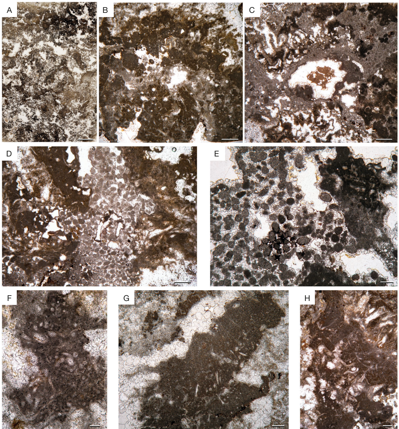
FIG. 12. — GR4 internal part microfacies; A , overview showing the porosity determined by the voids, partially filled by peloidal accumulations between the micritic columns; B , detail of peloids showing features of faecal pellets; C , cellular structures (type 5); D , E , spaces between columns filled by peloidal accumulations; F , G , micritic clusters containing intertwined filaments (type 4); H , composite crust with elongated filamentous and cellular structures. Scale bars: A, 5 mm; B-D, 500 µm; E, H, 200 µm; F, G, 100 µm.
