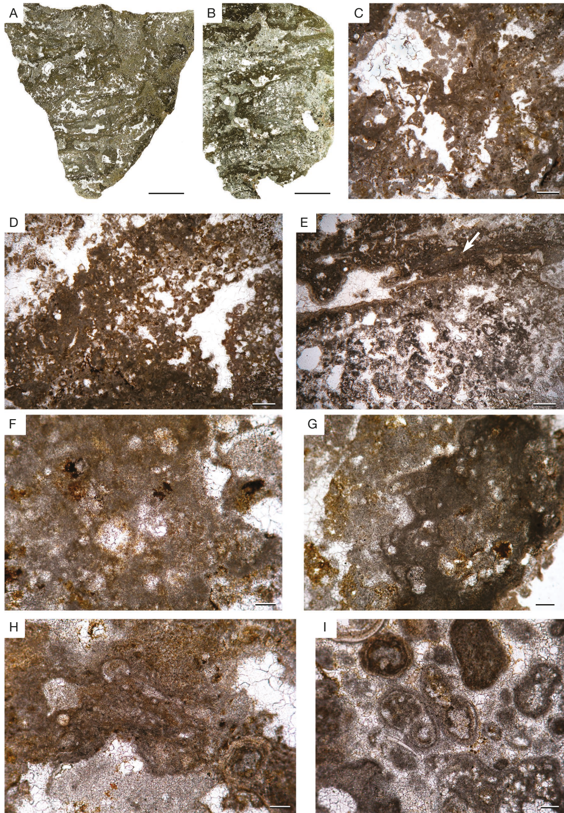
FIG. 15. — GR5 dome-shaped top microfacies; A, B , general views showing dense micritic crusts; C , detail of micritic columns; D , partially peloidal micritic crust with poorly expressed filamentous structures; E , composite micritic crust with very degraded coralline crusts and fine filamentous structures (arrow); F, G , coralline crusts (type 2) showing fairly well-preserved cell structures; H , probable coralline crust; I , accumulations of peloids often oolitized and bioclasts with undetermined honeycomb structures (see Fig. 10G). Scale bars: A, B, 5 mm; C, D, 500 \mu m; E, 200 \mu m; F-I, 100 \mu m.
