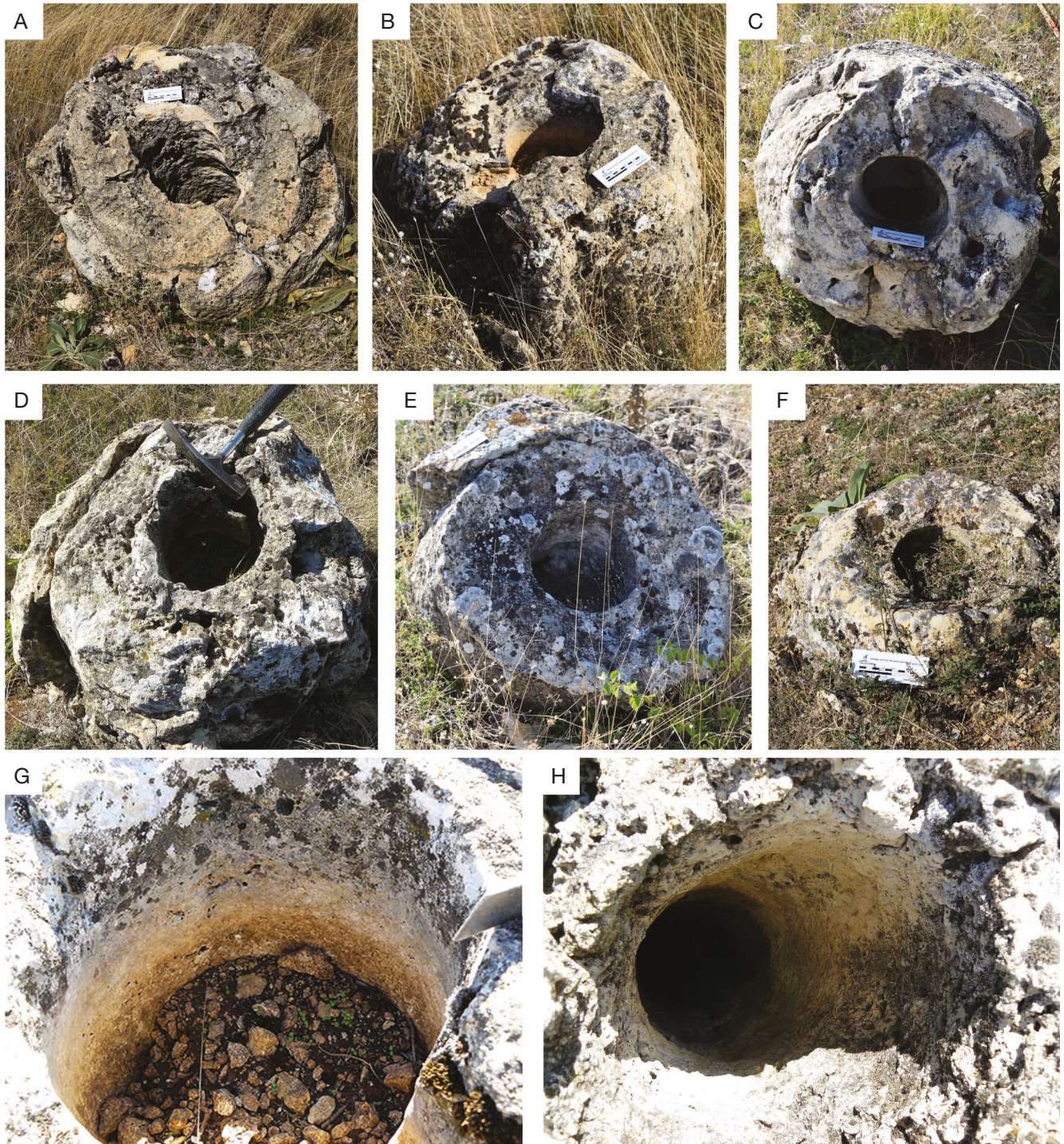
FIG. 7. — A–F , Different views of the cylinders showing the central cavity with usually smooth edges; G, H , detailed views showing the smooth internal structures. Scale bars: A–C, F, G, 10 cm; D, E, the hammer gives the scale.
