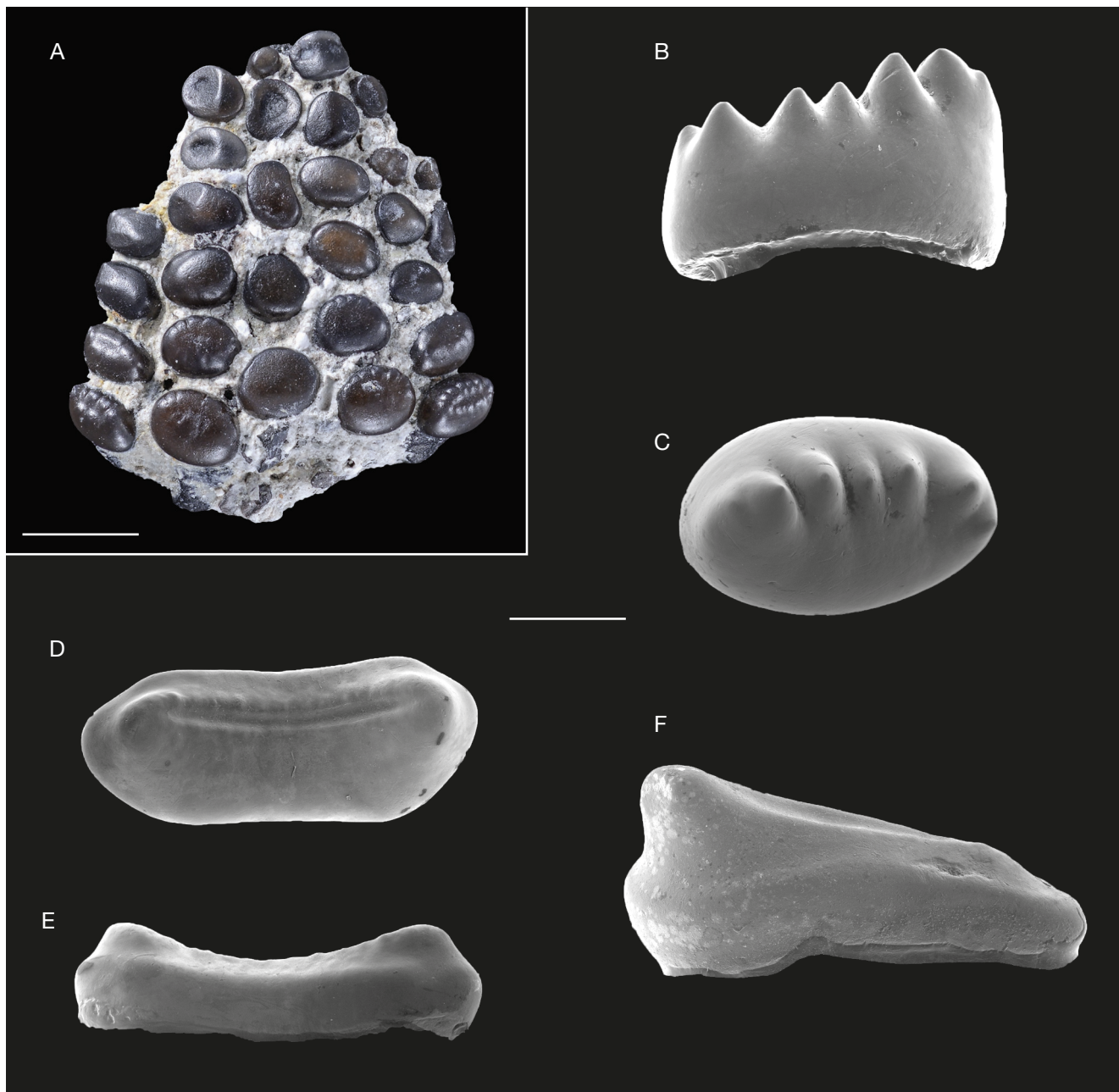
FIG. 6. — Actinopterygian remains from Angeac-Charente: A , vomerine dentition of cf. Micropycnodon sp. (ANG M-69) in occlusal view; B , C , detailed view of an isolated vomerine tooth of cf. Micropycnodon sp. (ANG M-28) in (B) anterior and (C) occlusal views; D , E , isolated tooth of Pycnodontidae indet. (ANG M-50) in occlusal (D) and lateral (E) views; F , isolated tooth of Pycnodontidae indet. (ANG M-59) in lateral view. Scale bars: A, 2.5 mm; B, C, F, 500 µm; D, E, 1 mm.
