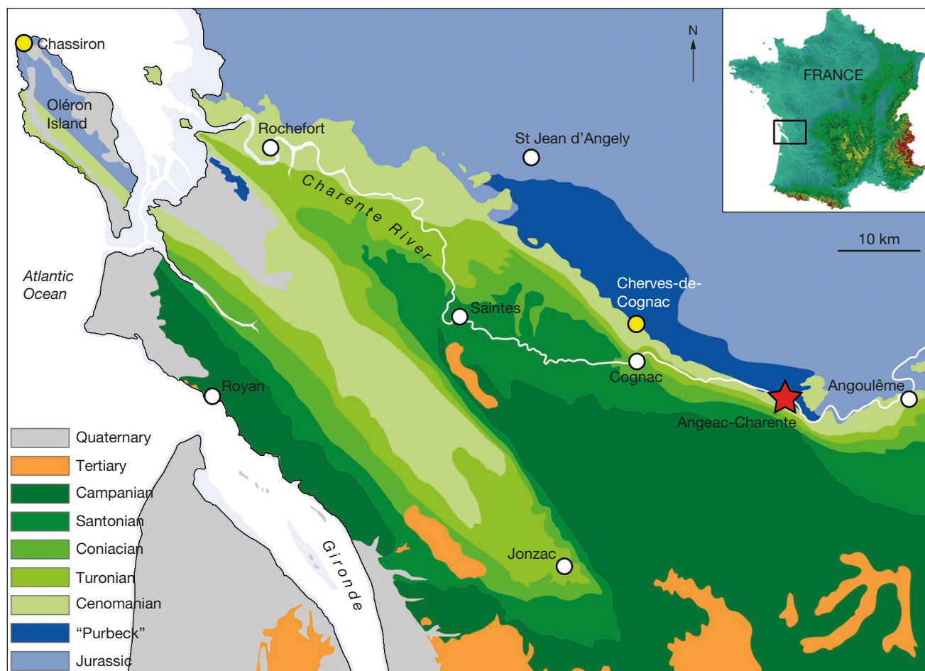
FIG. 1. — Geographical distribution of the three continental fossil localities documenting the Late Jurassic to Early Cretaceous transition in Western France: Chassiron (Tithonian, Department of Charente-Maritime), Cherves-de-Cognac (Berriasian, Department of Charente) and Angeac-Charente (Berriasian, Department of Charente).
