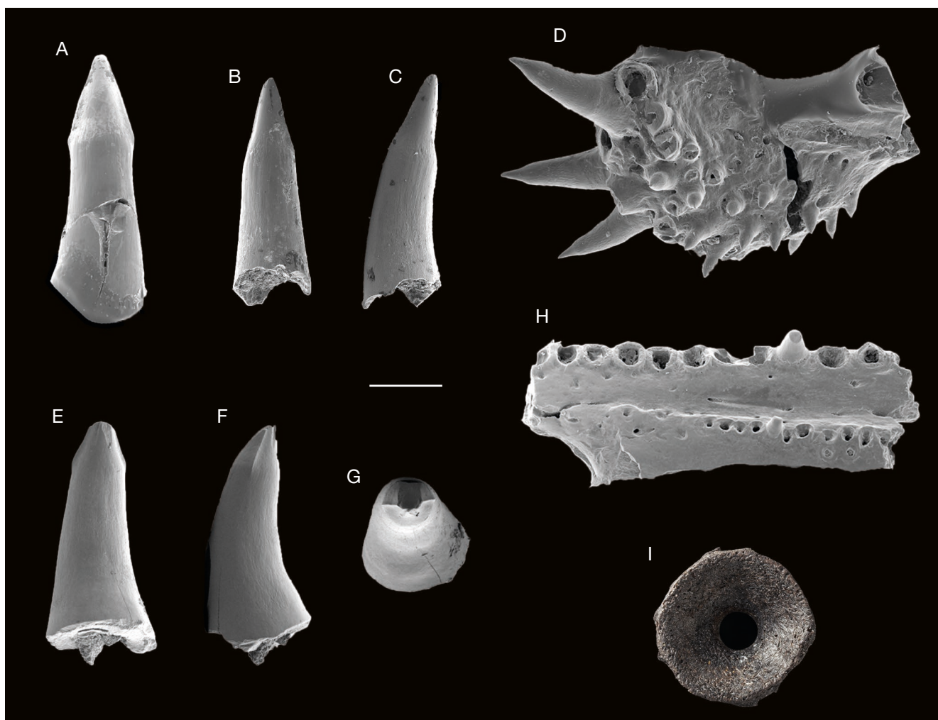
FIG. 8. — Actinopterygian remains from the Berriasian of Angeac-Charente: A , isolated tooth of Amiiformes indet. (ANG M-39); B , C , isolated tooth of Amiiformes indet. (ANG M-110); D , dentulous vomerine element of Amiiformes indet. (ANG M-56); E – G , isolated tooth of Ionoscopiformes indet. (ANG M-111); H , jaw fragment of Actinopterygii indet. (ANG M-38) in lingual view; I , vertebra of Actinopterygii indet. (ANG M-069). Scale bar: A–C, E–H, 500 µm; D, 250 µm; I, 2 mm.
