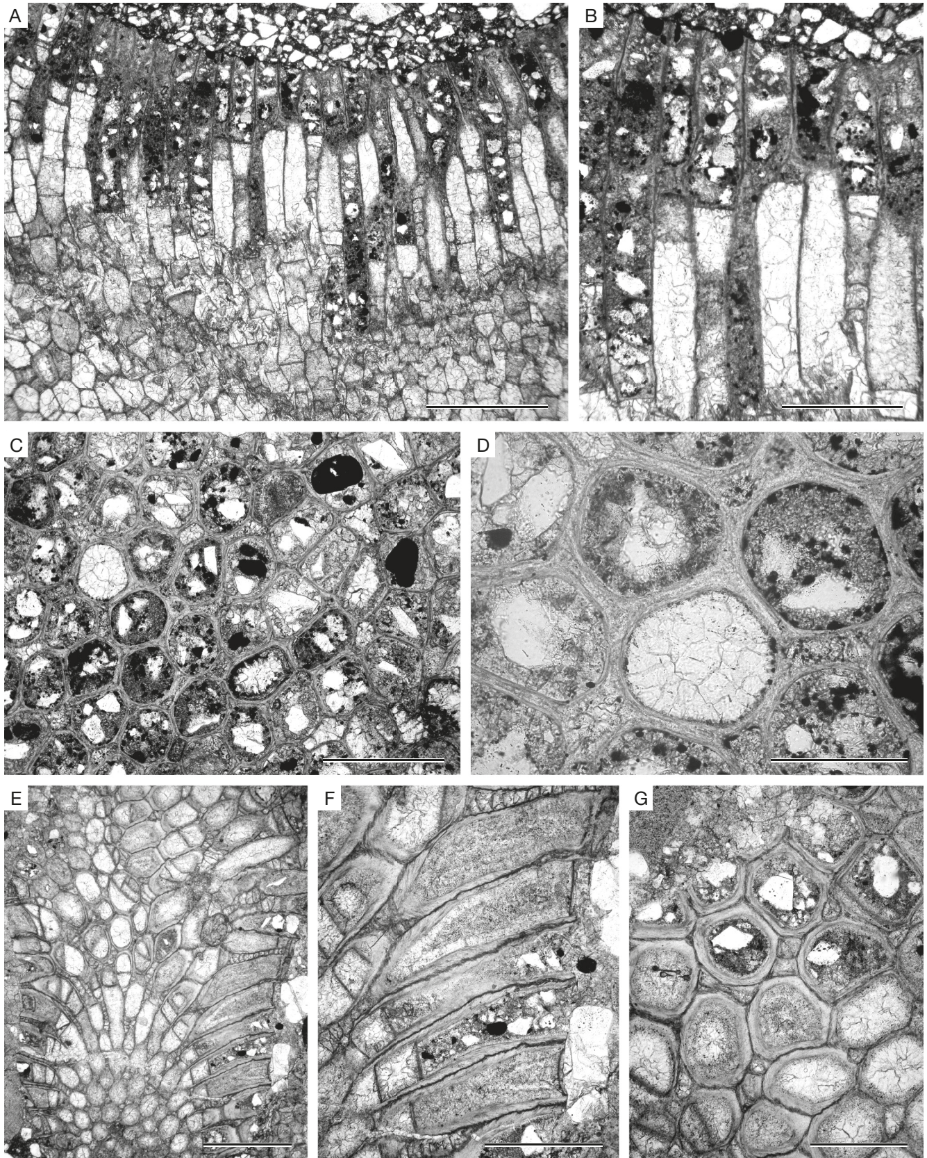
FIG. 10. — A-D , Diplotrypa sp. A , CEGH-UNC 27543 a: A , B , longitudinal section showing autozooeal chambers with diaphragms and mesozooeia; C , D , tangential thin section showing autozooeal apertures and mesozooeia; E-G , Tarphophragma macrostoma (Loeblich, 1942), CEGH-UNC 27520 d: E , oblique section through the colony; F , longitudinal section showing autozooeal chambers and mesozooeia; G , tangential thin section showing autozooeal apertures and mesozooeia. Scale bars: A , E , 1 mm; B , C , F , G , 0.5 mm; D , 0.2 mm.
