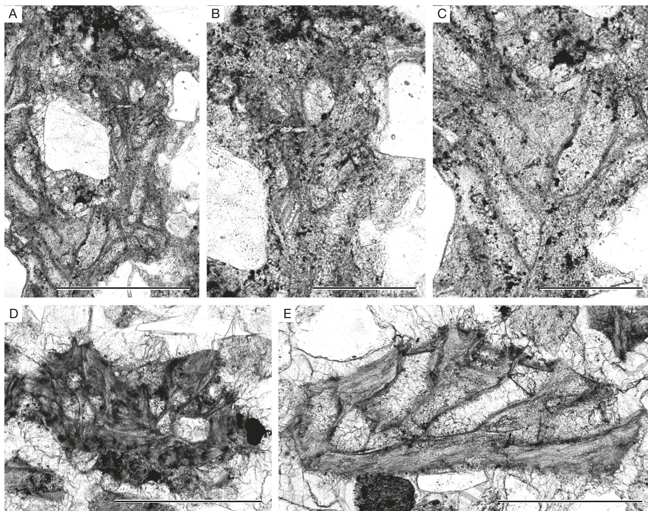
FIG. 17. — A-E , Parachasmatopora sp. A: A-C , tangential section showing branches with autozooeal apertures and chambers, CEGH-UNC 27526 a; D , branch transverse section showing autozooeal chambers and laminated skeleton, CEGH-UNC 27545 a; E , branch longitudinal section showing autozooeal chambers with diaphragms and laminated skeleton, CEGH-UNC 27545 b. Scale bars: A, D, E, 0.5 mm; B, C, 0.2 mm.
