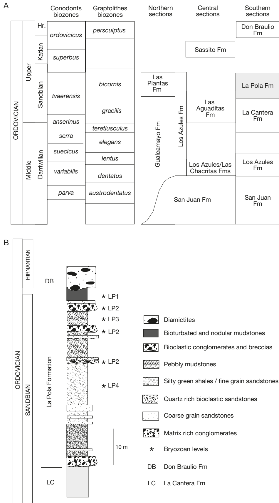
FIG. 2. — A , stratigraphic chart showing main Ordovician units (including La Pola Formation) of the Argentinean Precordillera disposed according north-south distribution; B , lithological column of the La Pola section in the Villicum range.
