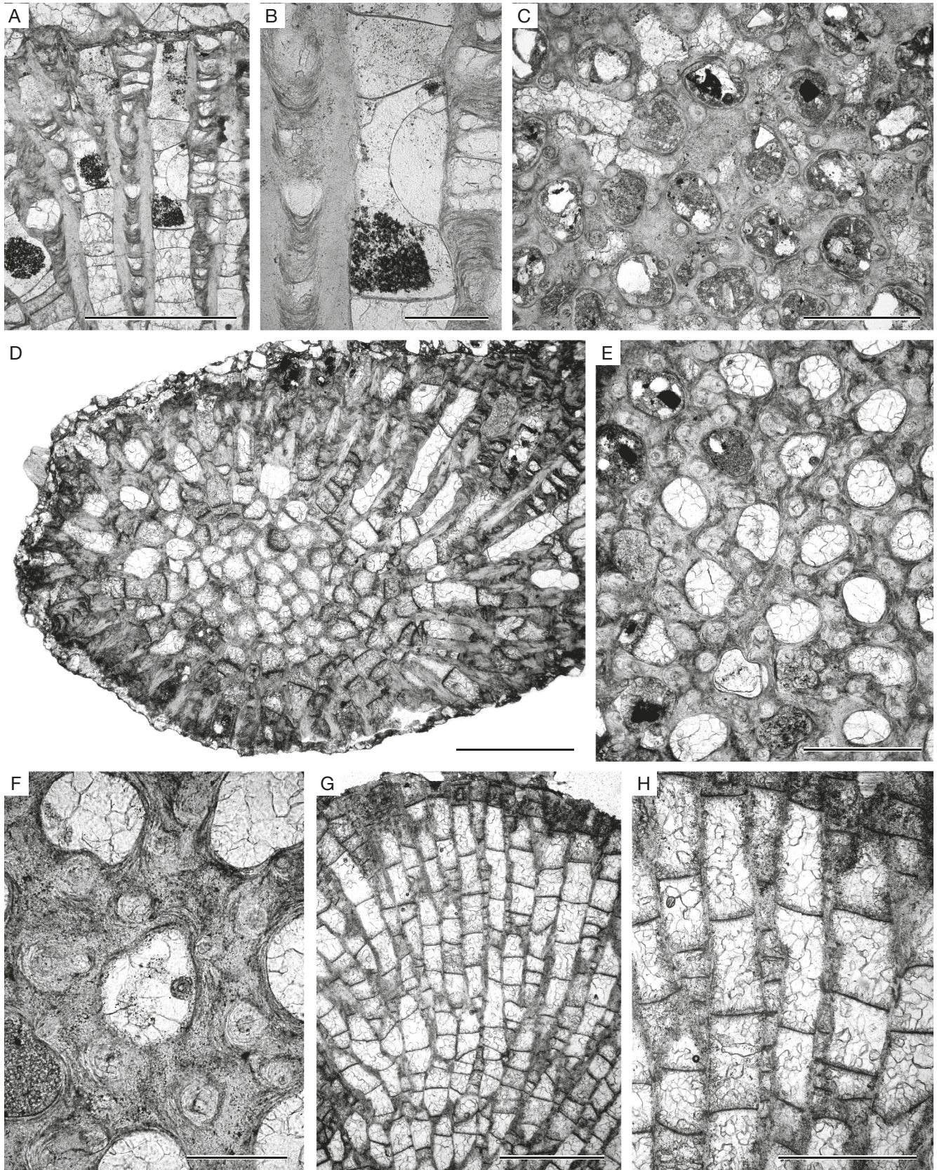
FIG. 12. — A–F. Argentinopora robusta n. gen., n. sp.: A, B , longitudinal thin section showing autozooeceal chambers with a cystiphragm, mesozooecia, acanthostyles, holotype CEGH-UNC 27511 a; C , tangential thin section showing autozooeceal apertures, mesozooecia, and acanthostyles, holotype CEGH-UNC 27511 d; D , branch transverse section, paratype CEGH-UNC 27514 b; E, F , tangential thin section showing autozooeceal apertures, mesozooecia, and acanthostyles, paratype CEGH-UNC 27514 c; G, H. Nicholsonella spinigera n. sp., branch longitudinal section showing autozooeceal chambers with diaphragms, holotype CEGH-UNC 27528 c. Scale bars: A, D, G, 1 mm; B, F, 0.2 mm; C, E, H, 0.5 mm.
