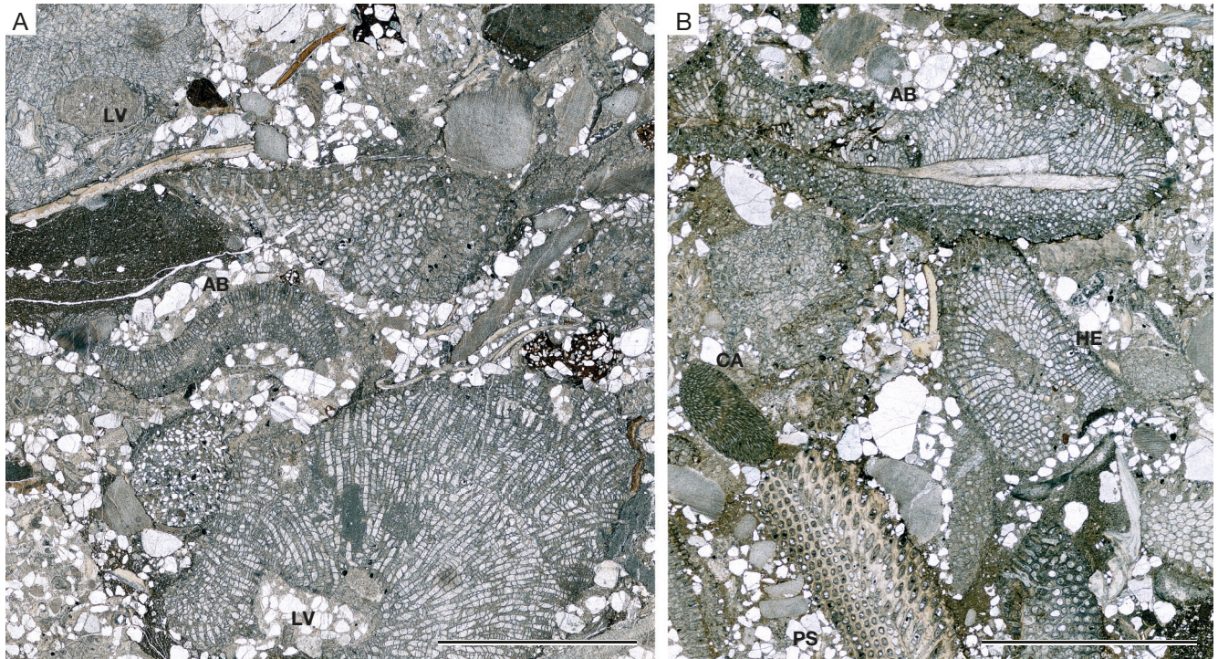
FIG. 3. — Microfacies of the main bryozoan-bearing rocks (lenticular quartz-bioclastic-rich sandstones) containing fragmented bryozoans (PS, Pseudostictoporella simplex n. sp.; AB, Albardonia bifoliata n. gen., n. sp.; LV, Lunaferamita virginiensis Utgaard, 1981; HE, Heterotrypa enodis n. sp.), brachiopod shells, crinoids, calcareous algae (CA), as well as lithoclasts in the siliciclastic matrix; A, CEGH-UNC 27520 b; B, CEGH-UNC 27530 e. Scale bars: 5 mm.
