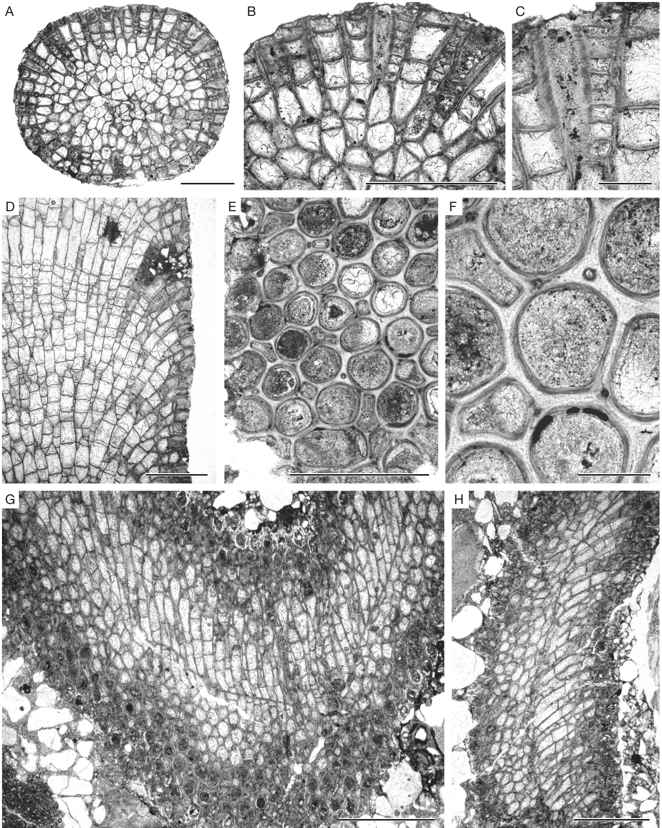
FIG. 8. — A-F , Heterotrypa enodis n. sp.: A-C , branch transverse section showing autozooeal chambers and mesozooeia, holotype CEGH-UNC 27504 b; D , branch longitudinal section showing autozooeal chambers with diaphragms and mesozooeia, CEGH-UNC 27504 a; E, F , tangential thin section showing autozooeal apertures, mesozooeia, and acanthostyles, CEGH-UNC 27504 c; G, H , Albardonía bifoliata n. gen., n. sp., oblique thin section through the bifoliate colony, holotype CEGH-UNC 27538 c. Scale bars: A, B, D, E, G, H, 1 mm; C, F, 0.2 mm.
