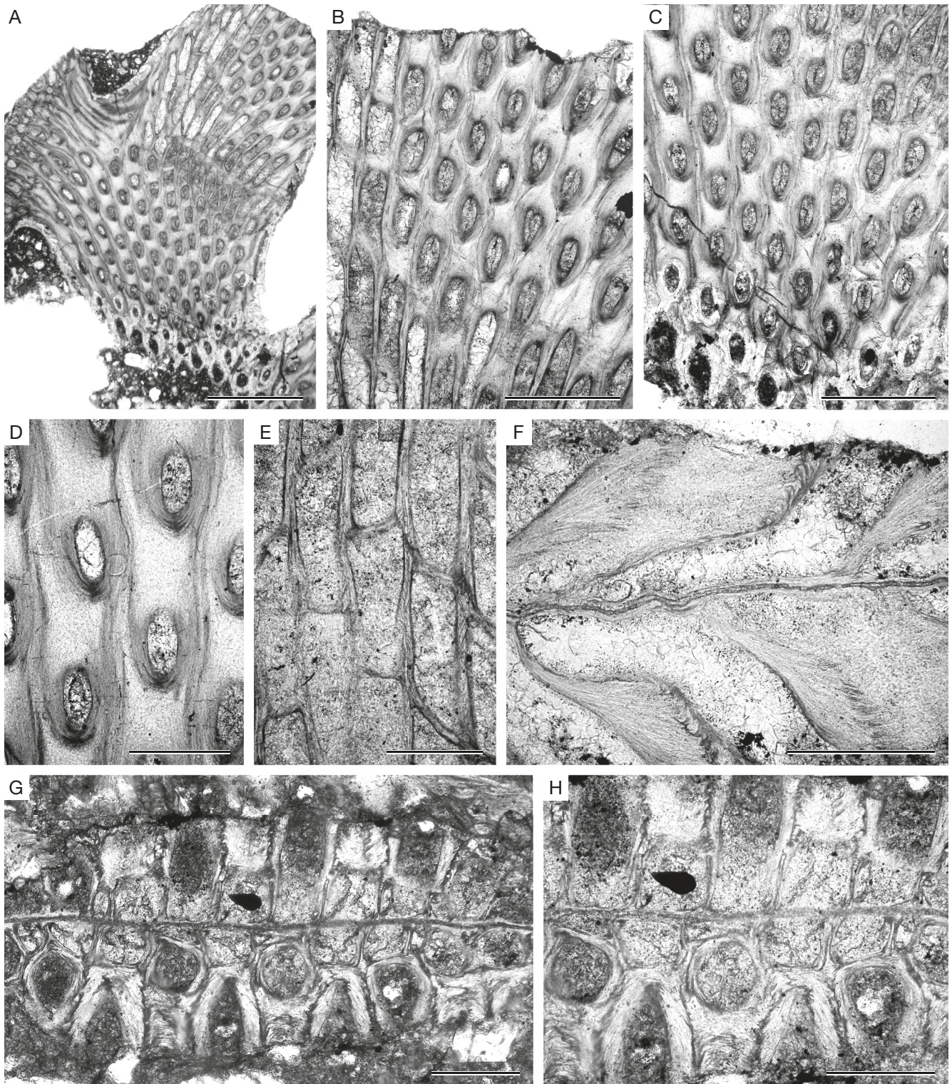
FIG. 15. — A-H , Pseudostictoporella simplex n. sp.: A-E , branch tangential section showing autozooeal chambers and apertures, holotype CEGH-UNC 27508 a; F , branch longitudinal thin section autozooeal chambers, paratype CEGH-UNC 27533 a; G, H , branch transverse thin section showing autozooeal chambers and mesotheca without rods, paratype CEGH-UNC 27533 d. Scale bars: A, 1 mm; B, C, 0.5 mm; D-H, 0.2 mm.
