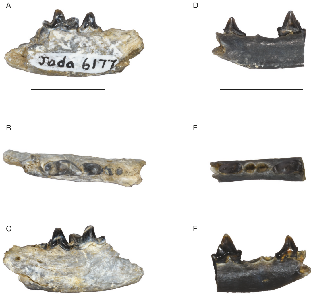
FIG. 3. — Dentaries of Palaeogale doroithiae MacDonald, 1963: A , lingual view (JODA 6177); B , occlusal view (JODA 6177); C , buccal view (JODA 6177); D , lingual view (JODA 5893); E , occlusal view (JODA 5893); F , buccal view (JODA 5893). Scale bars: 1 cm.
