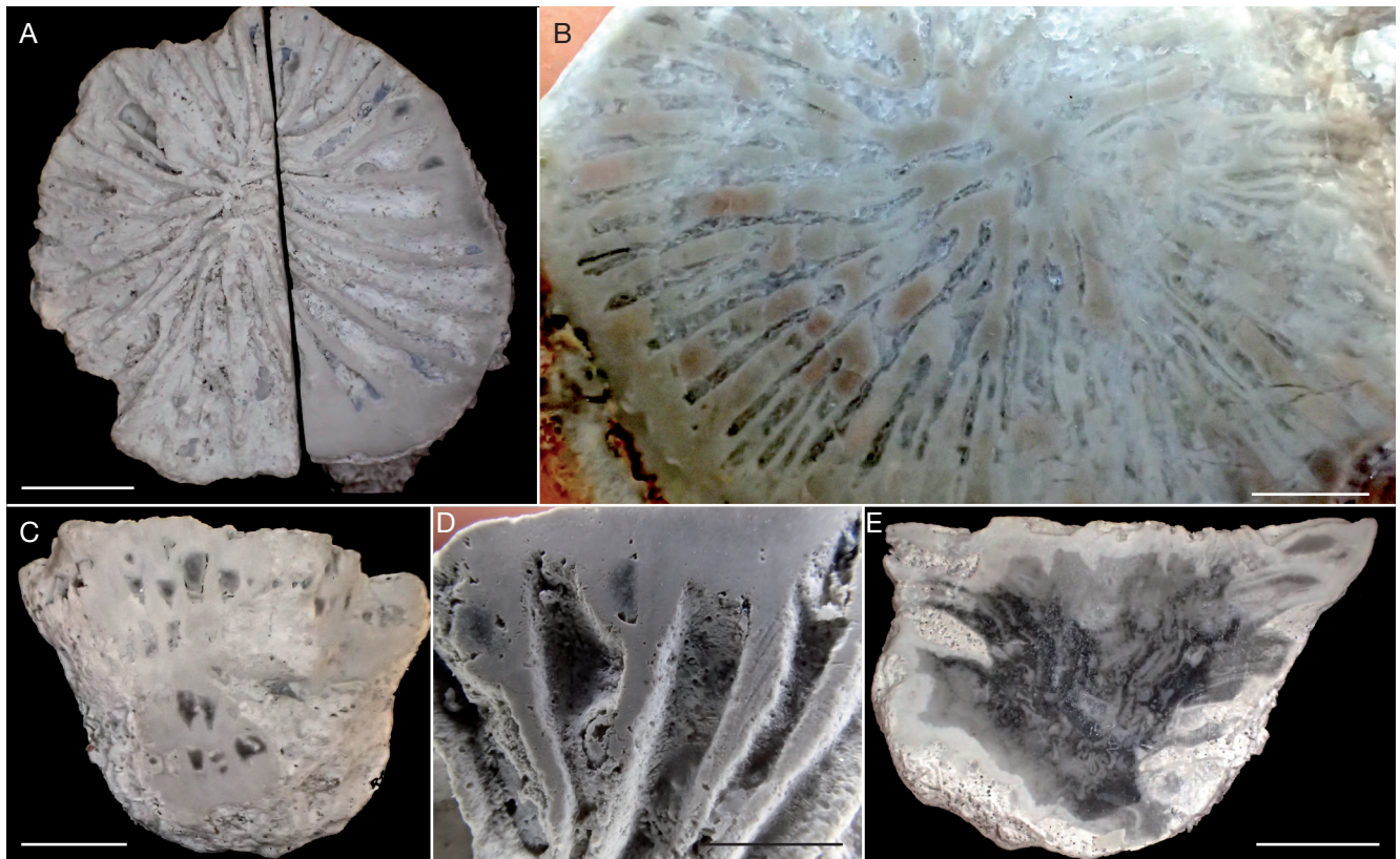
FIG. 3. — Alloiteausmilium boudaharensis Beauvais, 1986: A , distal view of the holotype MNHN.F.R11603; B , transverse section in the specimen CPUN DA2905E1'-1; C , partially polished lateral view of holotype MNHN.F.R11603; D , detail in distal view of the holotype MNHN.F.R11603 showing the link between endotheca and septa; E , longitudinal section of the holotype MNHN.F.R11603. Scale bars: A, C, E, 1 cm; B, D, 5 mm.
