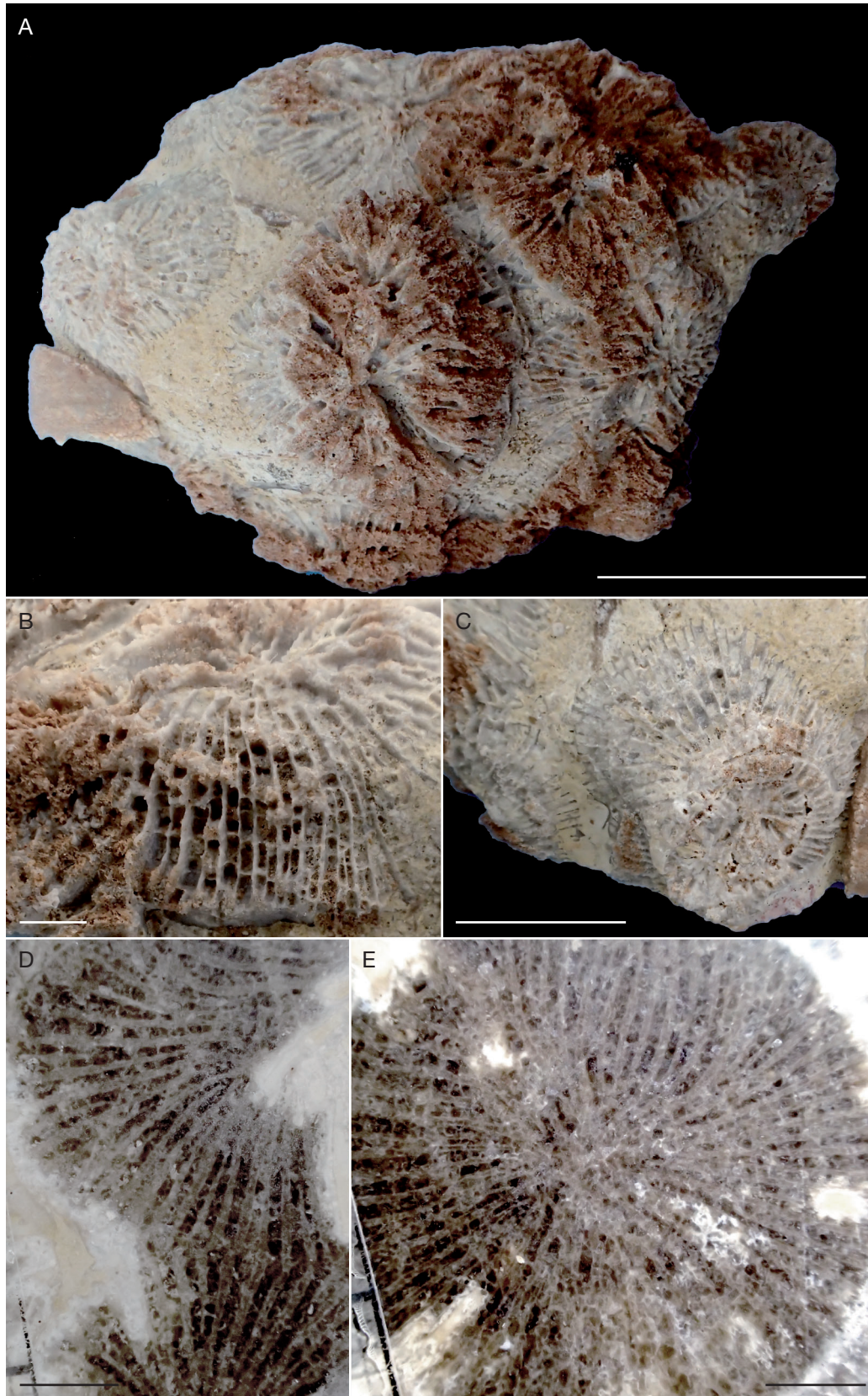
FIG. 61. — Complexastrea cf. gregaria (M'Coy, 1848): A , distal view of the specimen CPUN MA0504E2-3; B , lateral view of one corallite of the specimen CPUN MA0504E2-3; C , distal view of one calice of the specimen CPUN MA0504E2-3; D , transverse polished section of the specimen CPUN MA0504E2-4; E , transverse polished section of the specimen CPUN MA0504E2-4. Scale bars: A, 2 cm; B, 2 mm; C, 1 cm; D, E, 4 mm.
