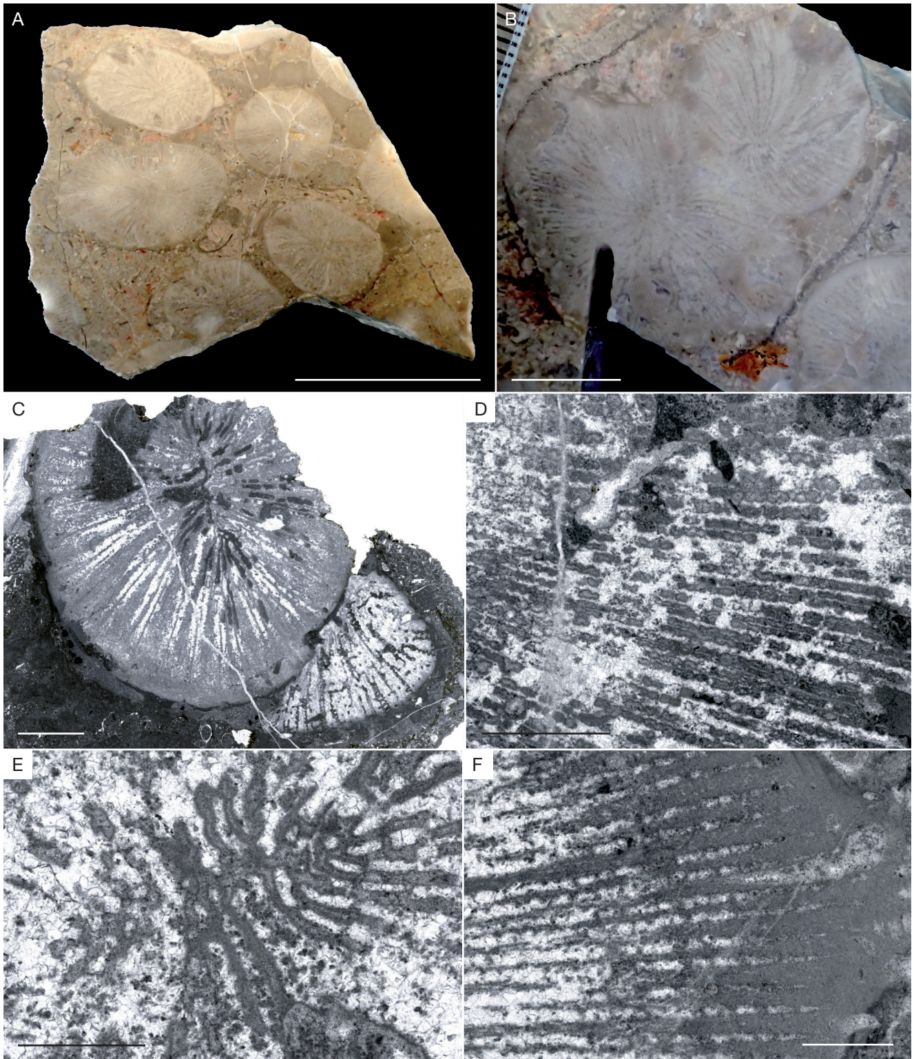
FIG. 37. — Margarosmilia ? sp.: A , lateral view of the specimen MNHN.F.R11617; B , distal view of the specimen MNHN.F.R11617; C , lateral view of the major calice, corallum specimen MNHN.F.R11617; D , distal view of the major calice of the specimen MNHN.F.R11617; E , detail of the septal ornamentation of the major calice of the specimen MNHN.F.R11617. Scale bars: A, B, 1 cm; C, 2 mm; D, 4 mm; E, 1 mm.
