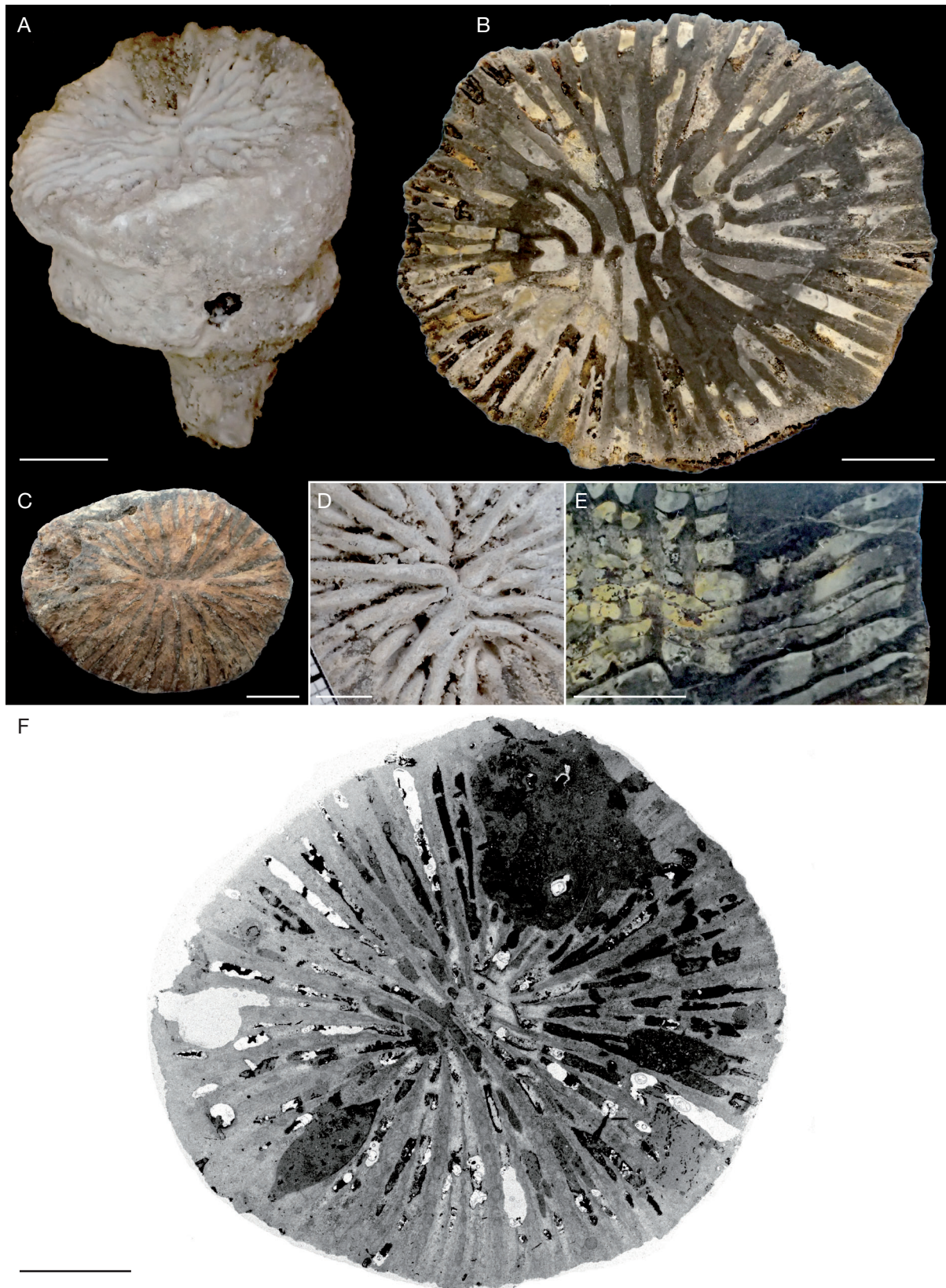
FIG. 47. — Epismiliopsis paraeudesi n. sp.: A , slightly oblique lateral view of the specimen MNHN.F.R11596; B , transverse polished section of the specimen CPUN 2703A3-5; C , distal view of the specimen CPUN 2303A6-2; D , detail in distal view of the axial fossa of the specimen MNHN.F.R11596; E , polished longitudinal axial section (following the elongated fossa) of the specimen CPUN 2703A3-5; F , transverse polished section of the specimen CPUN AM16188-11. Scale bars: A, C, 1 cm; B, E, 5 mm; D, F, 4 mm.
