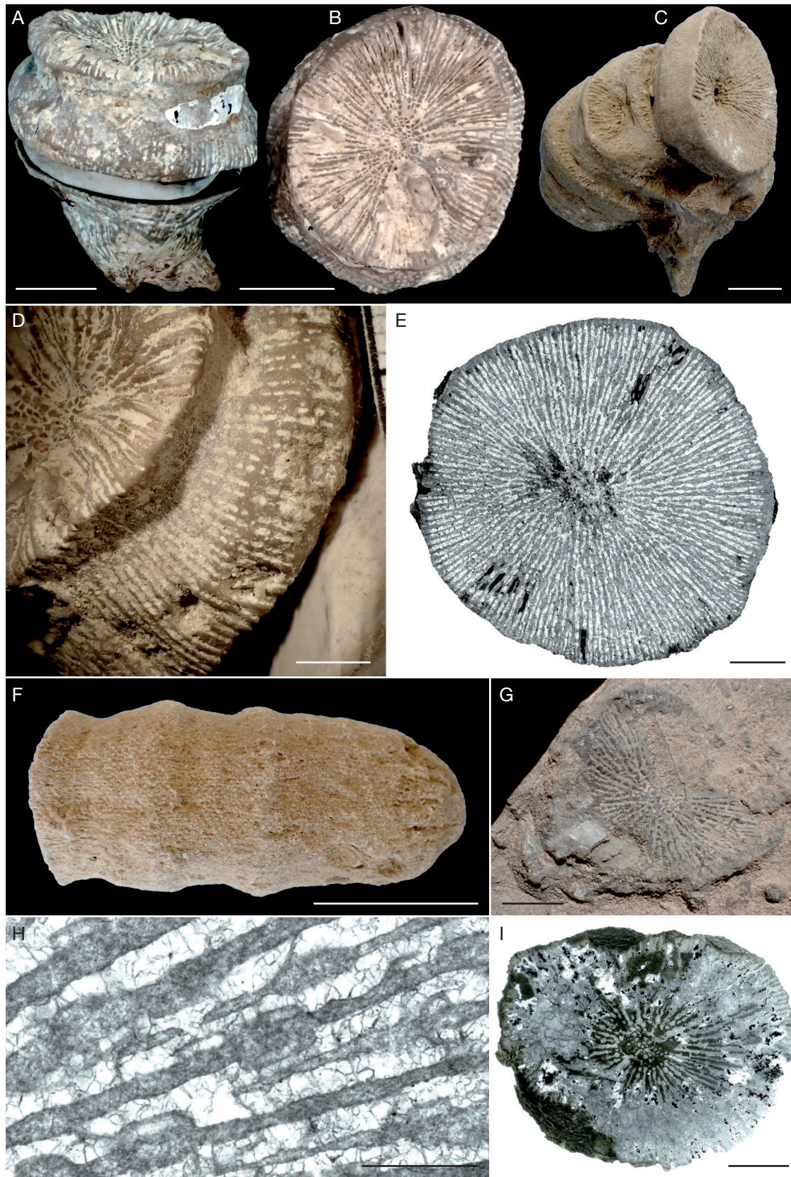
FIG. 23. — Proleptophyllia granulum (Fromentel & Ferry, 1866): A , lectotype MNHN.F.M03533; B , distal view of the lectotype MNHN.F.M03533; C , rejuvenescent specimen from the batch CPUN MA1004E1-G; D , detail of costoseptal structure in the lectotype MNHN.F.M03533; E , transverse thin section of the specimen CPUN CDAm5; F , subcylindrical specimen that lost his epitheca from the batch CPUN MA1004E1-G; G , specimen pictured in the field (Dades Valley, Morocco); H , detail of the pennular septal ornamentation in the specimen CPUN G'3; I , transverse thin section of the specimen CPUN AM16182-7. Scale bars: A, B, C, 1 cm; D, E, 4 mm; F, 2 mm; G, I, 5 mm; H, 1 mm.
