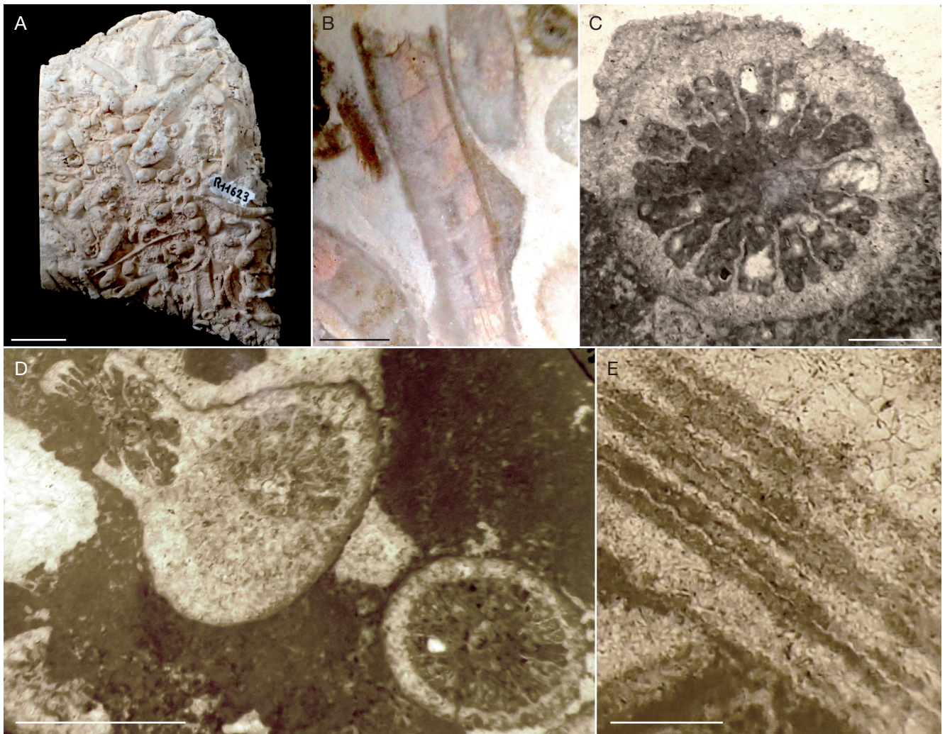
FIG. 45. — “ Stylosmilia ” dresnayi Beauvais, 1986: A , distal view of the holotype MNHN.F.R11623; B , polished longitudinal section in one corallum of the holotype MNHN.F.R11623; C , transverse thin section in one corallum of the holotype MNHN.F.R11623; D , transverse thin section in the holotype MNHN.F.R11623; E , oblique thin section of septa in a corallum of the holotype MNHN.F.R11623. Scale bars: A, 1 mm; B, D, 2 mm; C, E, 0.5 mm.
