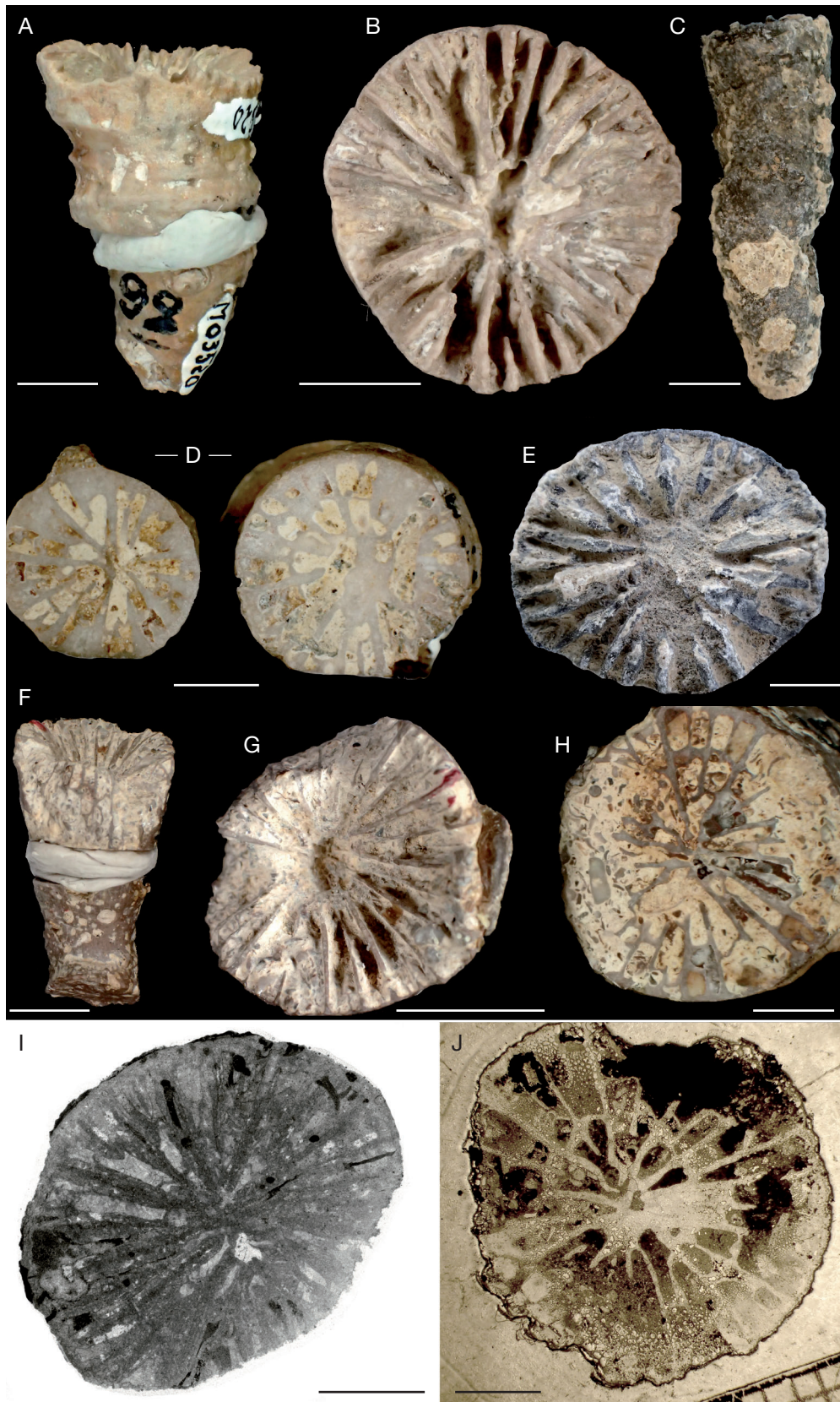
FIG. 55. — Stylophyllopsis fritillus (Fromental & Ferry, 1866): A , lateral view of the specimen MNHN.F.M03520; B , distal view of the specimen MNHN.F.M03520; C , lateral view of the specimen CPUN AM16179-6; D , polished sections of the specimen MNHN.F.M03520; E , distal view of the specimen CPUN AM16179-6; F , lateral view of the holotype MNHN.F.M03502; G , distal view of the holotype MNHN.F.M03502; H , polished transverse section of the holotype MNHN.F.M03502; I , transverse thin section of the specimen CPUN AM16179-6; J , printing of the holotype MNHN.F.M03502 (transverse section). Scale bars: A, B, 5 mm; C, F, G, 1 cm; D, E, H, I, 4 mm; J, 3 mm.
