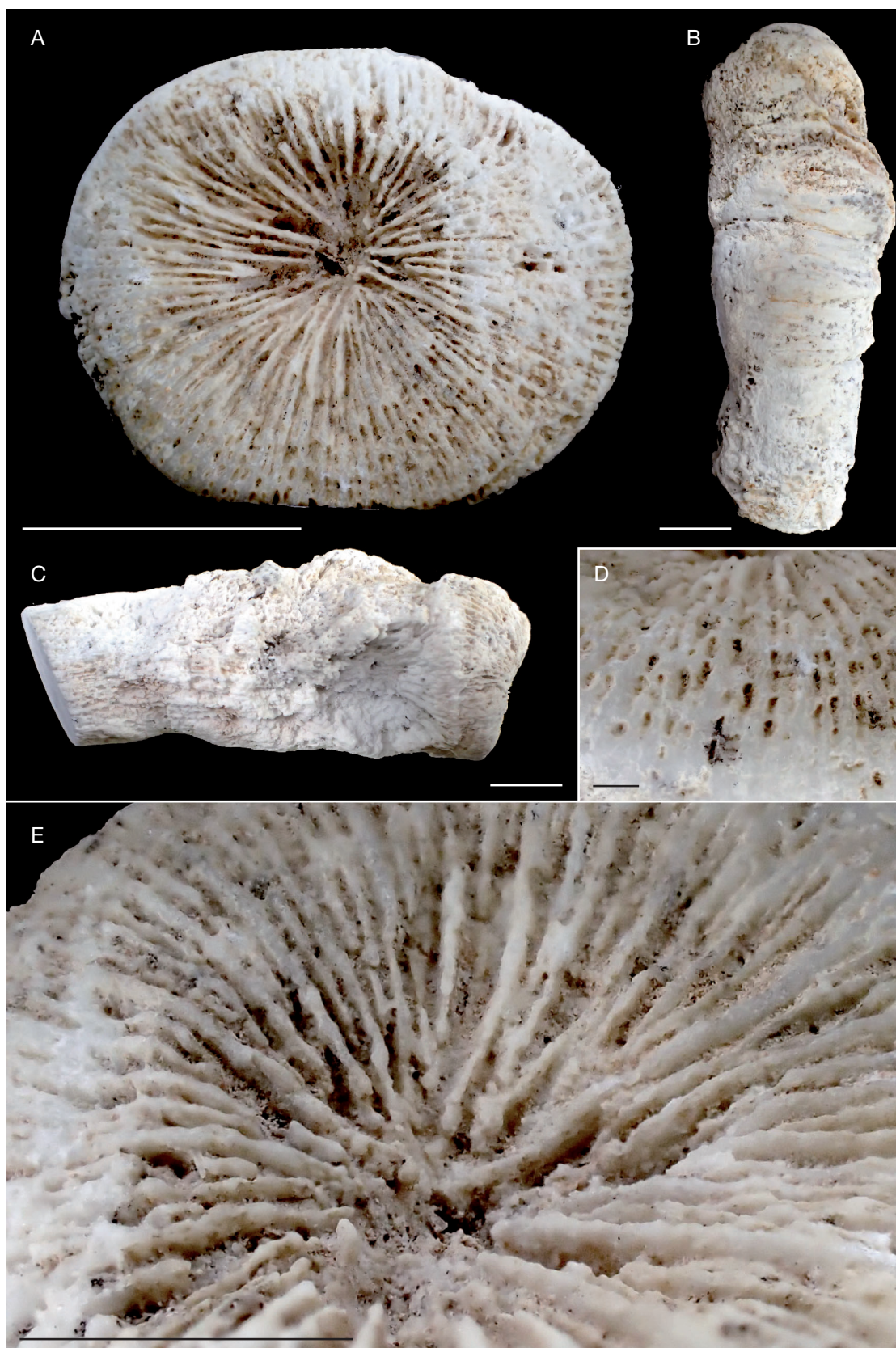
FIG. 57. — Stylophyllopsis vetusum (Beauvais, 1986): A , distal view of the holotype MNHN.F.R11648; B , lateral view of the holotype MNHN.F.R11648; C , lateral view of the holotype MNHN.F.R1164; D , distal peripheral view of the holotype MNHN.F.R11648; E , detail in distal view of the holotype MNHN.F.R11648. Scale bars: A, C, 1 cm; B, E, 5 mm; D, 1 mm.
