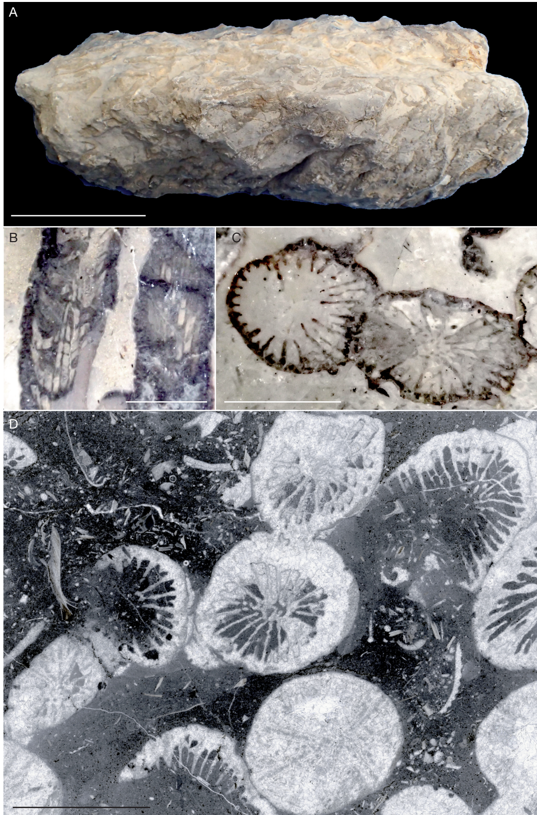
FIG. 49. — Phacelostylophyllum mg. arbustum n. sp.: A , distal view of specimen CPUN PFPyr13; B , longitudinal oblique section of two corallites of the specimen CPUN PFPyr13; C , transverse section of two corallites of the specimen CPUN PFPyr13; D , transverse thin section in specimen CPUN PFPyr13. Scale bars: A, 5 cm; B, C, D, 5 mm.
