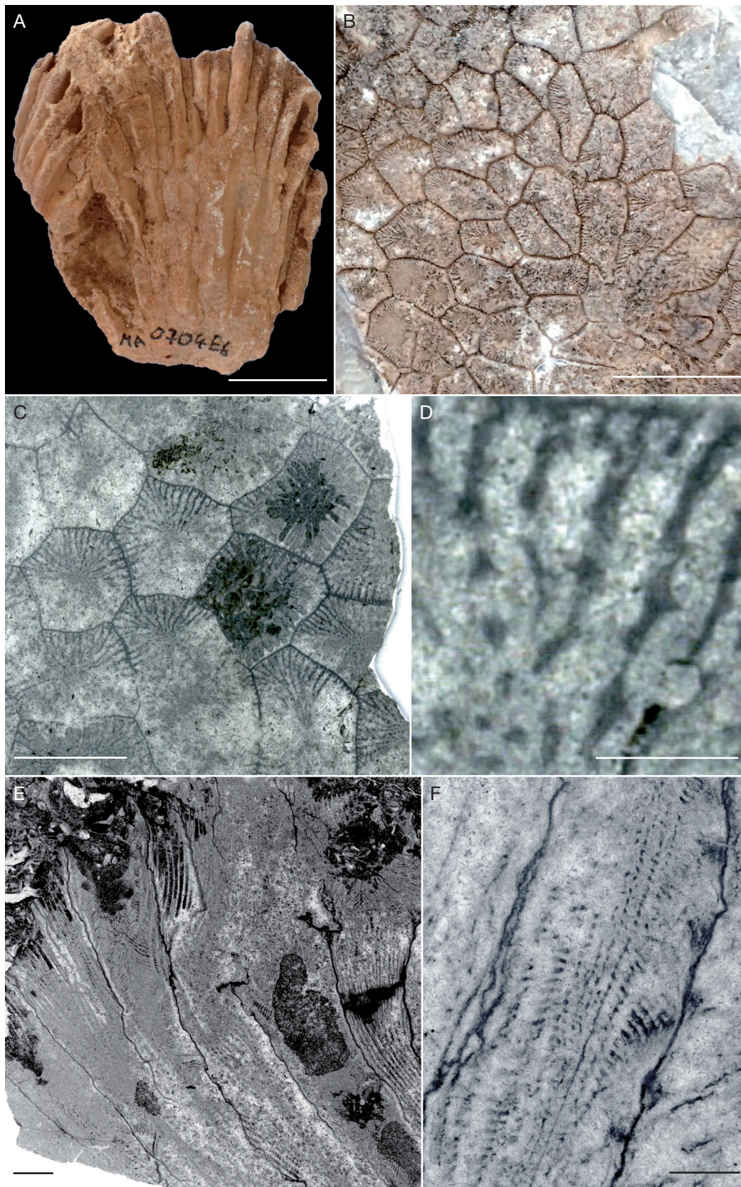
FIG. 65. — Prismaestrea organum n. gen., n. sp.: A , lateral view of specimen CPUN MA0704E6-2; B , distal view of specimen CPUN MA0704E6-1; C , transverse thin section in specimen CPUN MA0704E6-1; D , detail in transverse section of montlivatid septal microarchitecture in specimen CPUN MA0704E6-1; E , longitudinal thin section in the specimen CPUN MA0704E6-1; F , longitudinal thin section in the specimen CPUN MA0704E6-3. Scale bars: A, 2 cm; B, 1 cm; C, 4 mm; D, 0.5 mm; E, 2 mm; F, 1 mm.
