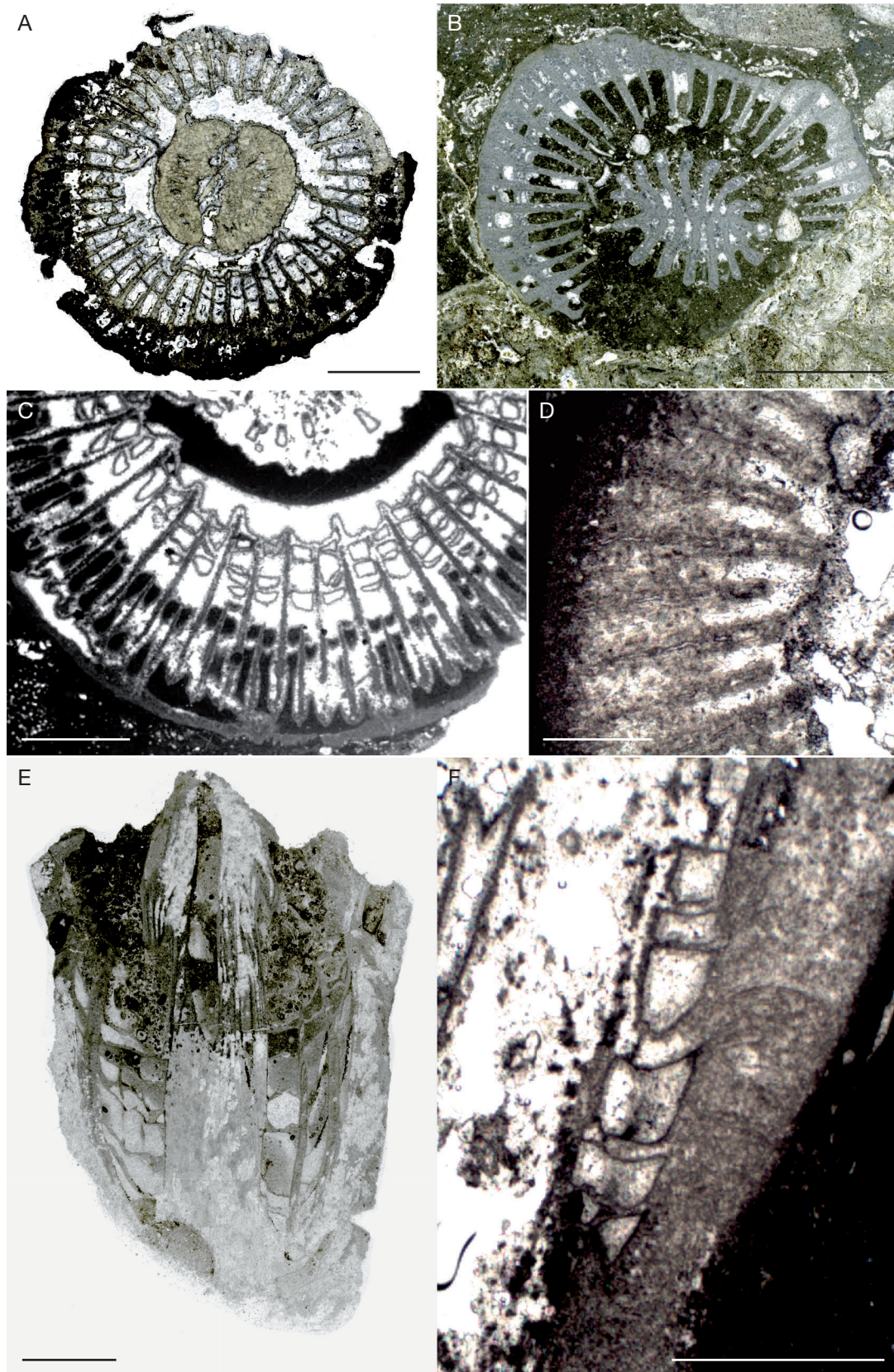
FIG. 32. — Neorylstonia pseudocolumellata (Beauvais, 1986): A : transverse section of the specimen CPUN AM16164, showing a type 2 pseudocolumella with visible pseudocolumellar septa; B : transverse section of the specimen CPUN AM175 showing a type 1 pseudocolumella; C : transverse section in the specimen CPUN DA2905E1.1 showing the true epitheca surrounding the septal apparatus and the stereome deposits on septa; D : detail of the ghosts of septal structure in transverse section (specimen CPUN 2110A2) and the stereome deposits in “ogives” or “glove fingers”; E : longitudinal section of the specimen MNHN.F.A57331-2 showing the endotheal organization in tabular dissepiments and the axial porosity of the pseudocolumella; F : detail of the parathecal wall in continuity with the tabular dissepiments (longitudinal section of the specimen CPUN 2110A2). Scale bars: A, B, E, F, 5 mm; C, 4 mm; D, 2 mm.
