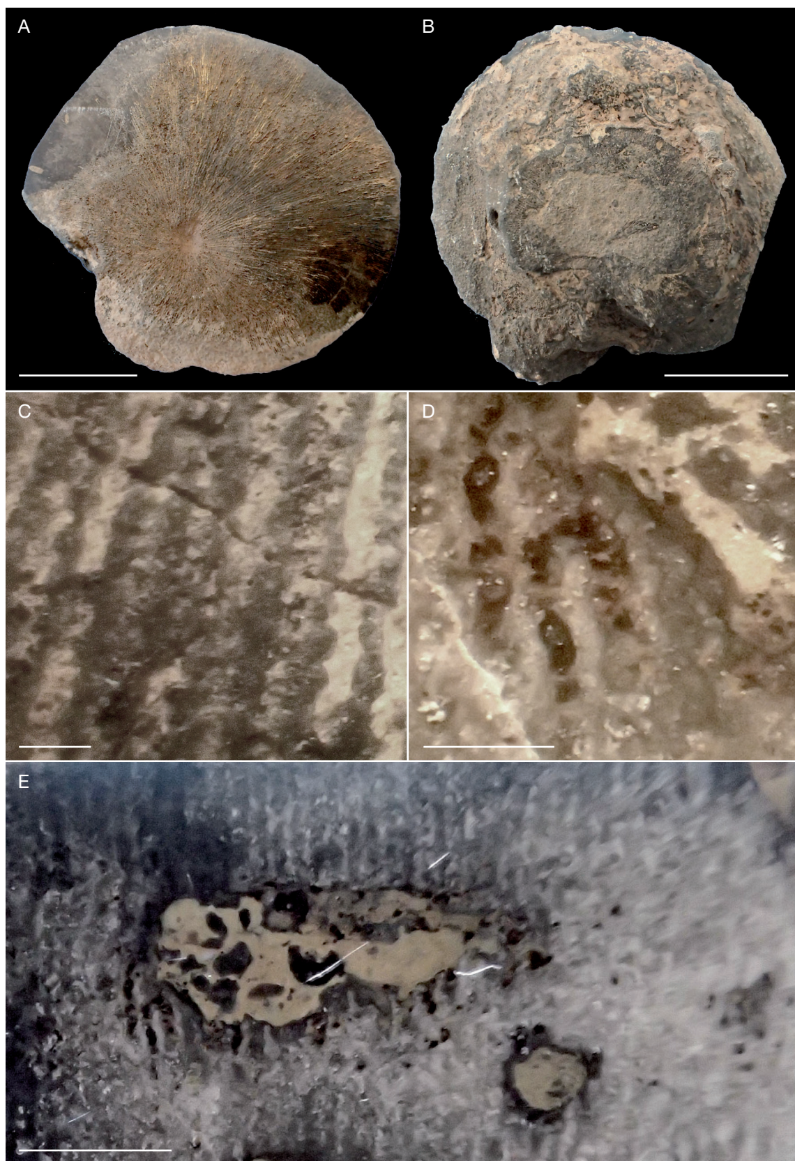
FIG. 24. — Proleptophyllia magna n. sp.: A , distal view of the specimen CPUN AM16160-1; B , proximal view of the specimen CPUN AM16160-1; C , pennular septal structure of the specimen CPUN AM16160-1 in distal view (skeleton in dark); D , pennular septal structure of the specimen CPUN AM16160-1 in polished longitudinal section; E , longitudinal polished section of the specimen CPUN AM16160-1. Scale bars: A, B, 2 cm; C, D, 0.5 mm; E, 2 mm.
