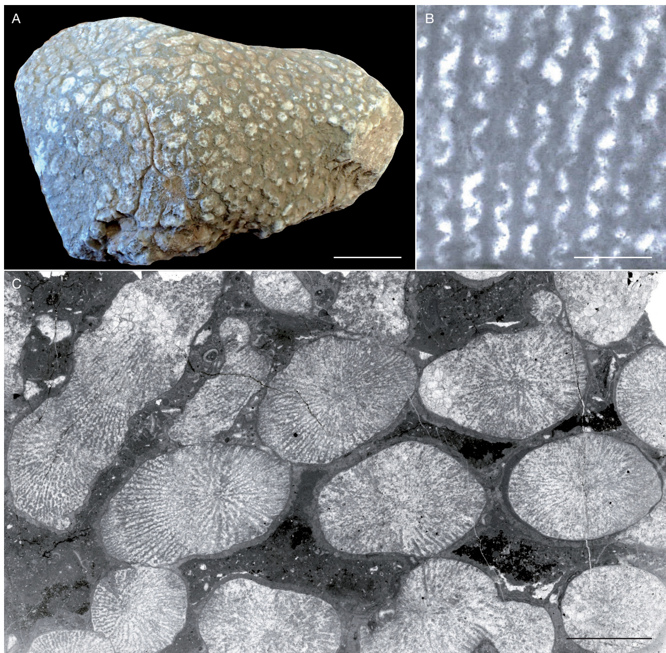
FIG. 31. — Gen. et sp. indet.: A , distal view of the specimen CPUN DA3105E1; B , detail in longitudinal thin section of pennular structures of septa in the specimen CPUN DA3105E1; C , transverse thin section in the specimen CPUN DA3105E1. Scale bars: A, 3 cm; B, 0.5 mm; C, 4 mm.
