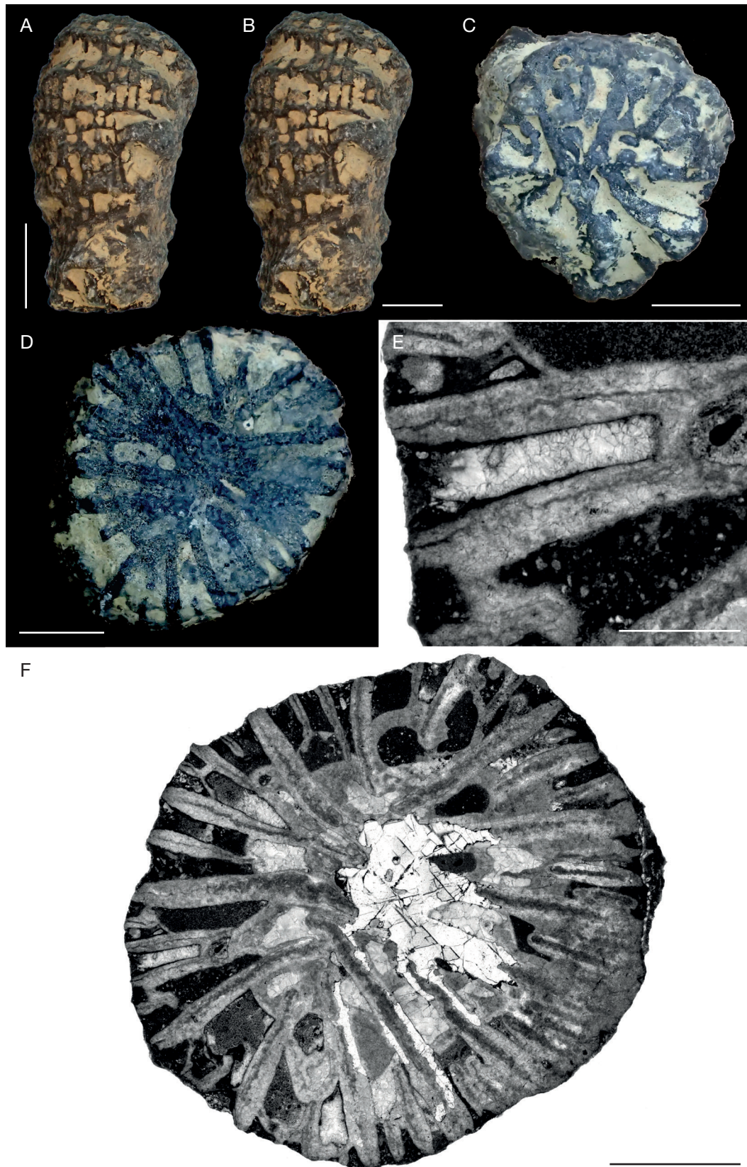
FIG. 58. — Stylophyllopsis zitteli Frech, 1890: A , lateral view of the specimen CPUN 2703A3-3; B , lateral view of the specimen CPUN AM16179-8; C , distal view of the specimen CPUN 2703A3-3; D , distal view of the specimen CPUN 2703A3-3; E , transverse thin section showing wavy mid-septal line in the specimen CPUN 2703A3-3; F , transverse thin section of the specimen CPUN 2703A3-3. Scale bars: A, B, 1 cm; C, D, 5 mm; E, 1 mm; F, 4 mm.
