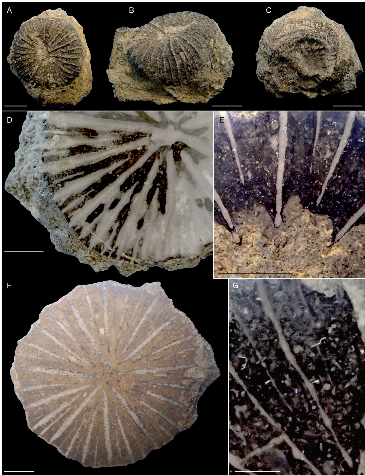
FIG. 54. — Stylophyllopsis bovista n. sp.: A , distal view of the specimen CPUN PFPyr6-7; B , lateral view of the specimen CPUN PFPyr6-7; C , proximal view of the specimen CPUN PFPyr6-7; D , transverse proximal polished section of the specimen CPUN PFPyr6-8; E , transverse distal polished section of the specimen CPUN PFPyr6-8 (detail of septal structure); F , transverse polished section of the specimen CPUN PFPyr6-10; G , transverse polished section of the specimen CPUN PFPyr6-11 (detail of septal structure). Scale bars: A, B, C, 1 cm; D, E, F, 5 mm; G, 2 mm.
