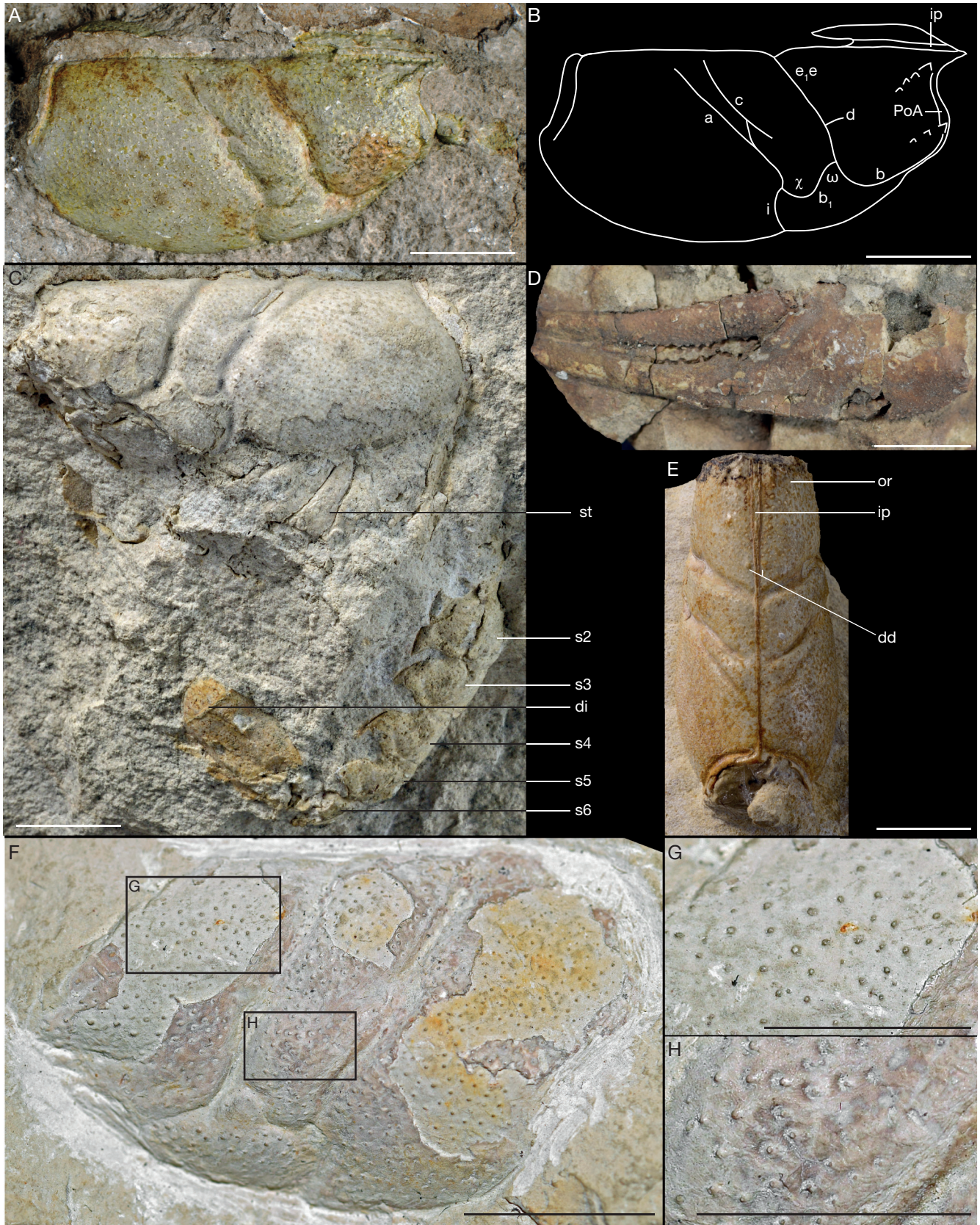
FIG. 3. — Eryma ventrosus (Meyer, 1835) from France: A, B , cast of the holotype MNHN.F.B12484 (Oxfordian, Frétille); general view (A), schema (B); C , specimen MNHN.F.A29468 (Oxfordian, Mailley); D , specimen MNHN.F.A29470 (Oxfordian, Mailley); E , specimen MNHN.F.A29479 (Oxfordian, Montcey); F-H , specimen BSPG 1961 VIII 148 (Kimmeridgian, Chablais): general view (F), detailed view of an entirely decorticated area (G), detailed view of an area non entirely decorticated (H). Abbreviations: a , branchiocardiac groove; b , antennal groove; b 1 , hepatic groove; c , postcervical groove; d , gastro-orbital groove; dd , dorsal domes; di , diaeresis; e, e , cervical groove; i , inferior groove; ip , intercalated plate; or , orbital row; PoA , post-orbital area; s2-s6 , pleonal somites; st , sternum; \chi , attachment site of adductor testis muscle; \omega , attachment site of mandibular muscle. Photographs: A, D, F-G, J. Devillez; C, L. Cazes; E, P. Loubry. Line drawing: J. Devillez. Scale bars: 1 cm.
