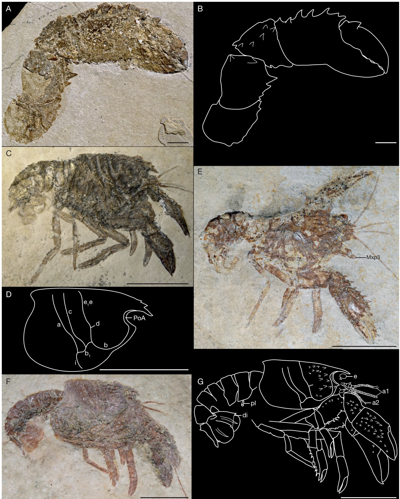
FIG. 12. — Palaeastacus rothgaengerae Schweigert & Röper, 2001 and Palaeastacus fuciformis (Schlotheim, 1822) from Germany: A, B , holotype BSPG 1993 XXVIII 200 of P. rothgaengerae from the Kimmeridgian of Brunn quarry: general view ( A ), schema ( B ); C, D , holotype MFN 2236 P1383/8 MB.A.0251 of P. fuciformis from the Tithonian of Solnhofen: general view ( C ), schema of the carapace ( D ); E , specimen MFN 2236 P1383/7 MB.A.2985 from the Tithonian of Eichstätt; F–G , specimen MFN 2236 P1383/7 MB.A.2992 from the Tithonian of Solnhofen: general view ( F ), schema ( G ). Abbreviations: a , branchiocardiac groove; a1 , antennulae; a2 , antenna; b , antennal groove; b1 , hepatic groove; c , postcervical groove; d , gastro-orbital groove; di , diaeresis; e , eye; e1e , cervical groove; i , inferior groove; ip , intercalated plate; Mxp3 , third maxilliped; pl , pleopod; PoA , postorbital area. Photographs: C, E, F, J. Devillez; A, G. Schweigert. Line drawings: J. Devillez. Scale bars: 1 cm.
