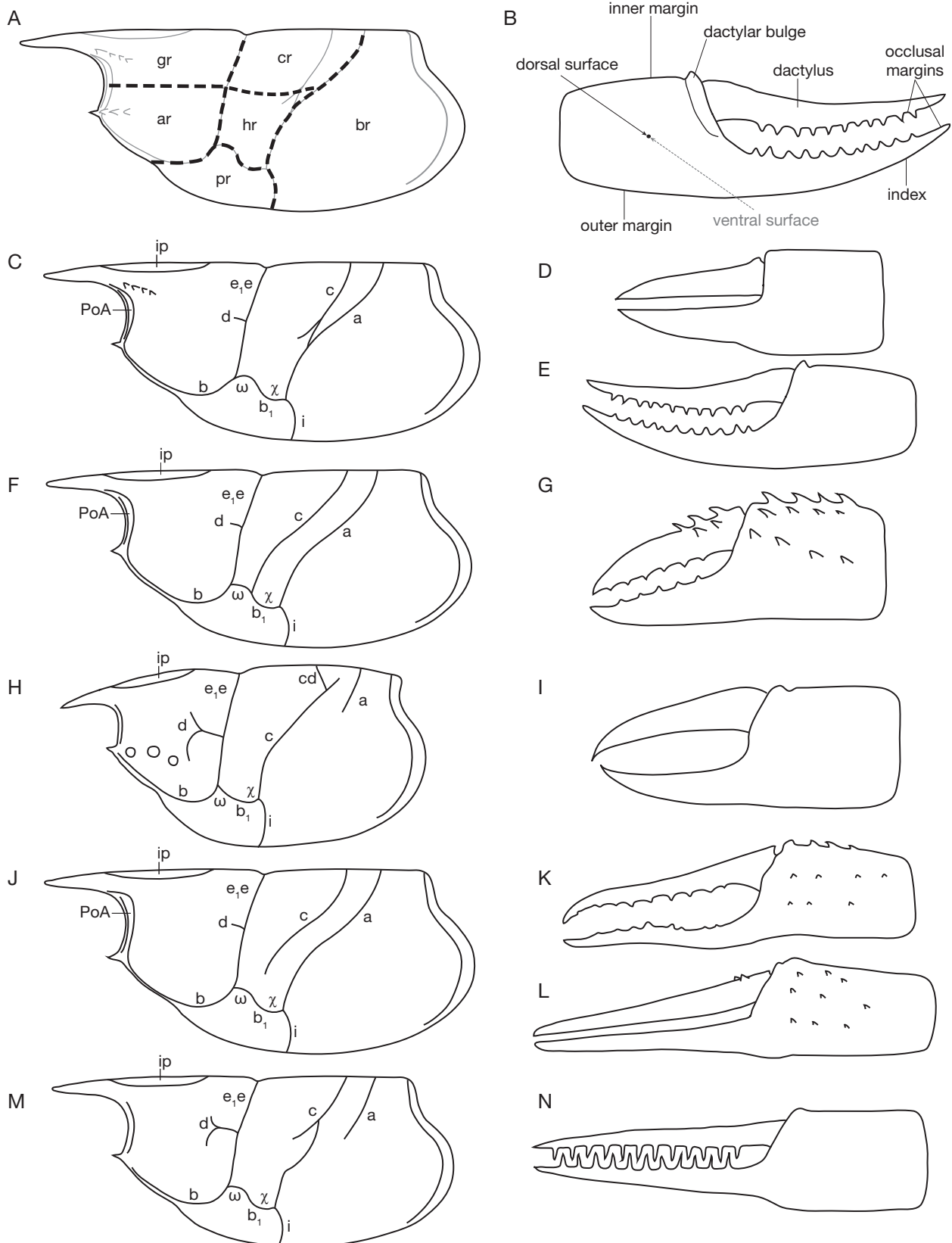
of pereiopods of Stenodactylina ; L , form II of chela of the first pair of pereiopods of Stenodactylina ; F , typical carapace groove pattern of Enoploclytia ; G , typical chela of the first pair of pereiopods of Enoploclytia . Abbreviations: a , branchiocardiac groove; ar , antennal region; b , antennal groove; b 1 , hepatic groove; br , branchial region; c , postcervical groove; cr , cardiac region; d , gastro-orbital groove; e 1 e , cervical groove; gr , gastric region; hr , hepatic region; i , inferior groove; ip , intercalated plate; PoA , post-orbital area; pr , pterygostomial region; χ , attachment site of adductor testis muscle; ω , attachment site of mandibular muscle. Line drawings: J. Devillez.
