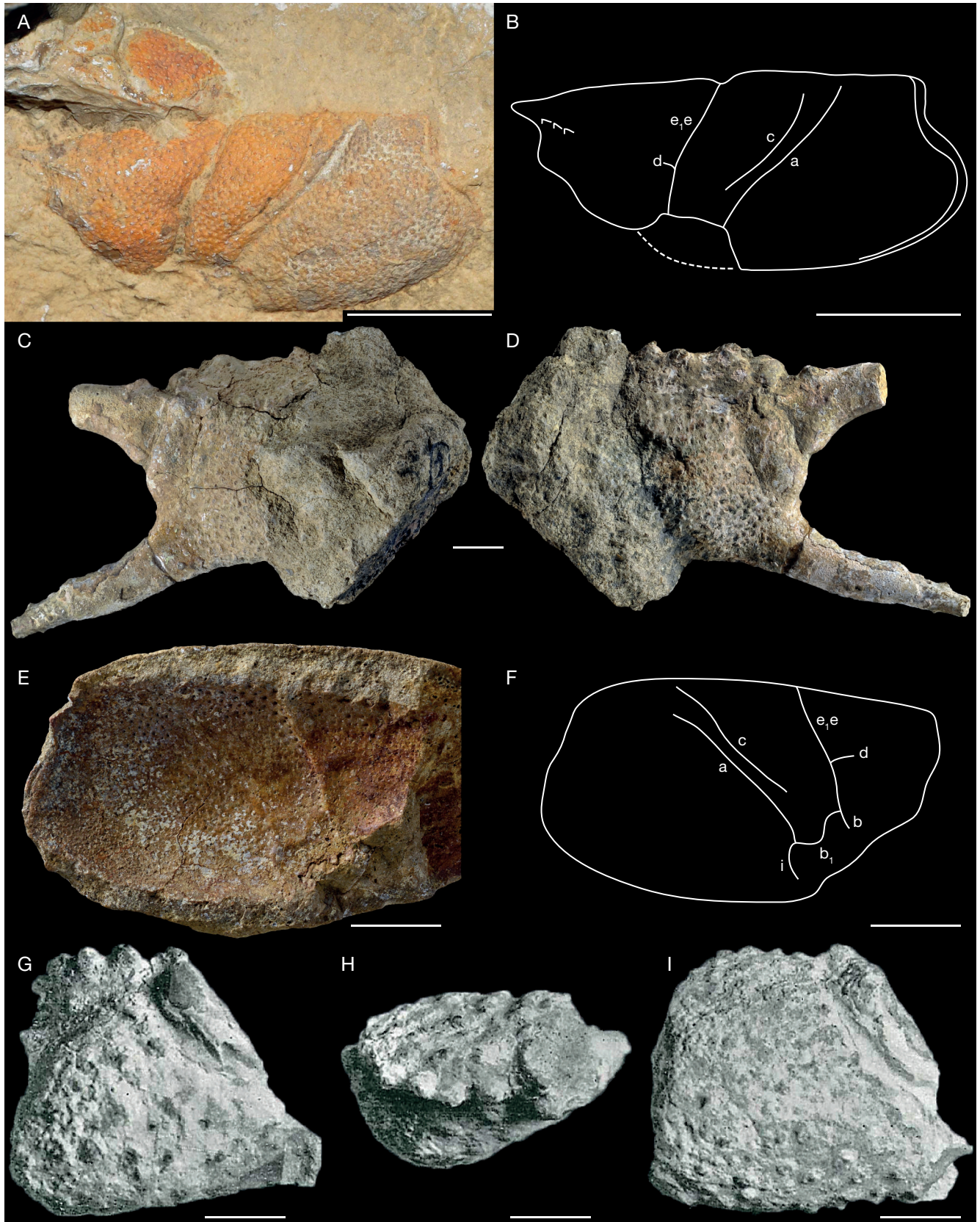
Marolalitra, Madagascar: general view ( E ), schema ( F ); G , H , original figures of Bachmayer (1959: pl. 2, fig. 2b, c) of the holotype of S. strambergensis (Tithonian, Stramberg, Czech Republic); I , original figure of Bachmayer (1959: pl. 2, fig. 2a) of the paratype of S. strambergensis (Tithonian, Stramberg, Czech Republic). Abbreviations: a , branchiocardiac groove; b , antennal groove; b 1 , hepatic groove; c , postcervical groove; d , gastro-orbital groove; e, e , cervical groove; i , inferior groove. Photographs: A, J. Devillez; C, D, C. Lemzaouda; E, L. Cazes. Line drawings: J. Devillez. Scale bars: 1 cm.
