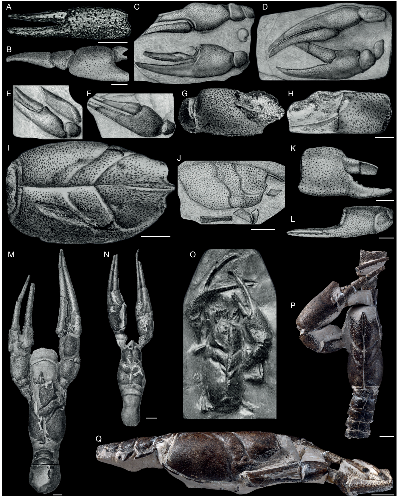
fig. 6) of Eryma fossata (Oxfordian, Galgenberg near Hildesheim, Germany); J , original figure of Sauvage (1891: pl. 4, fig. 6) of Eryma leblanci (Kimmeridgian, Boulogne-sur-Mer, France); K , original figure of Sauvage (1891: pl. 3, fig. 5) of Eryma boloniensis (Kimmeridgian, Boulogne-sur-Mer, France); L , original figure of Sauvage (1891: pl. 4, fig. 3) of Eryma beaugrandi (Kimmeridgian, Boulogne-sur-Mer, France); M , N , original figures of Morière (1883: pl. 1, figs 1-2) of the syntypes of Eryma villersi (Oxfordian, Villers-sur-Mer, France); O , original figure of Van Straelen (1925: pl. 9, fig. 1) of the holotype of Eryma morieri Hée, 1924 (Oxfordian, Villers-sur-Mer, France); P , Q , specimen from the Callovian of Villers-sur-Mer (France, private collection of J.-P. Pezy). Photographs: L. Cazes. Scale bars: 1 cm.
