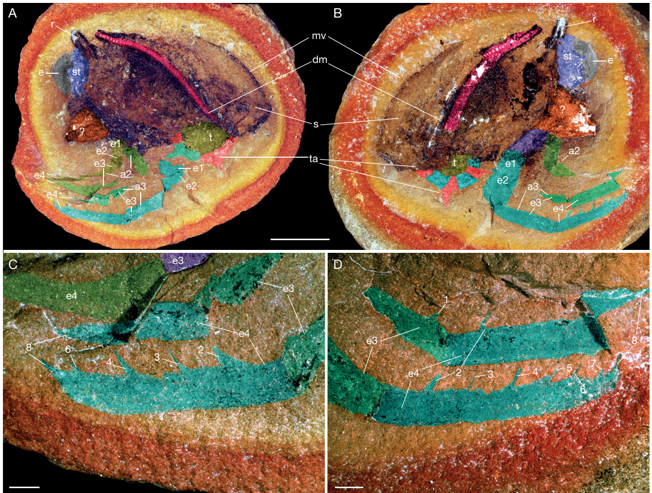
FIG. 7. — Eodollocaris keithflinti Laville, J.T. Haug & C. Haug, n. gen., n. sp., ROMIP61586: A, B , general view of part and counter-part (color-marked); C , close-up of appendages of A (color-marked); D , close-up of appendages of B (color-marked). Abbreviations: a2, a3 , second, third raptorial appendages; e , eyes; e1-e4 , element 1-4; dm , dorsal midline; mv , ventral margin; r , rostrum; s , shield; st , stalk; t , trunk; ta , trunk appendage; ? , indeterminate oval plate; 1-8 , spines 1-8. Photographs: C. Haug and J. T. Haug.. Scale bars: A, B, 5 mm; C, D, 1 mm.
