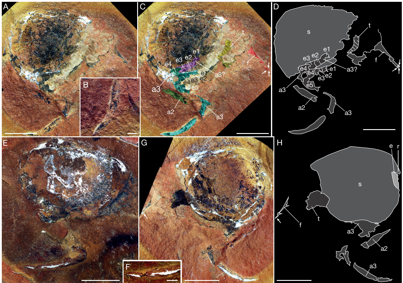
FIG. 4. — Concavicularis georgeorum Schram, 1990: A–D , ROMIP61591, part; A , general view; B , close-up of the third raptorial appendage; C , general view (color-marked); D , line drawing; E, F , ROMIP61588; E , general view; F , close-up of the third raptorial appendage; G, H , ROMIP61591, counter-part; G , general view; H , line drawing. Abbreviations: a2, a3 , second, third raptorial appendages; e , eyes; e1–e5 , element 1–5; f , furca?; r , rostrum; s , shield; t , trunk. Arrows indicate the spines of the possible furca. Photographs: C. Haug and J. T. Haug. Line drawings: T. Laville. Scale bars: A, C–E, G–H, 5 mm; B, F, 1 mm.
