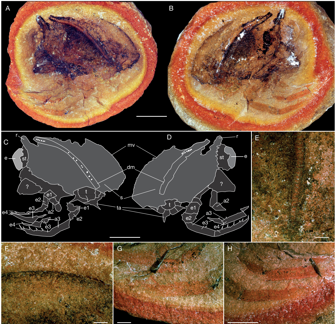
FIG. 6. — Eodollocaris keithflinti Laville, J.T. Haug & C. Haug, n. gen., n. sp., ROMIP61586: A, B , general view of part and counter-part; C , line drawing of A ; D , line drawing of B ; E , close-up of the dorsal midline of A ; F , close-up of ventral margin of A ; G , close-up of prominent appendages of A ; H , close-up of prominent appendages of B . Abbreviations: a2 , a3 , second, third raptorial appendages; e , eyes; e1-e4 , element 1-4; dm , dorsal midline; mv , ventral margin; r , rostrum; s , shield; st , stalk; t , trunk; ta , trunk appendage; ? , indeterminate oval plate. Photographs: C. Haug and J. T. Haug. Line drawings: Thomas Laville. Scale bars: A-D , 5 mm; E-H , 1 mm.
