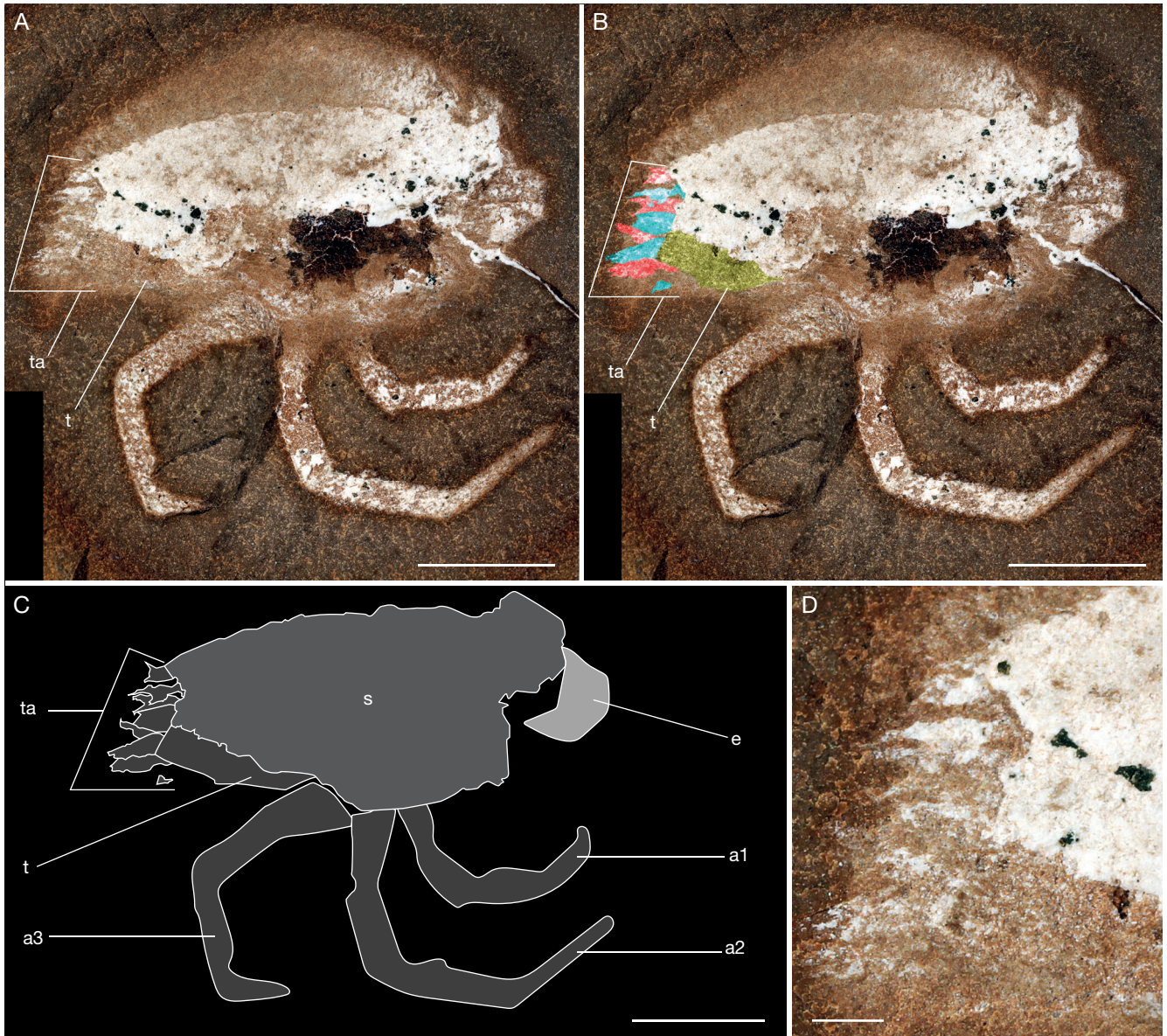
FIG. 5. — Convexicaris mazonensis Schram, 1990, ROMIP47987: A , general view; B , general view (color-marked); C , line drawing; D , close-up on trunk appendages. Abbreviations: a1-a3 , first, second, third raptorial appendages; e , eyes; s , shield; t , trunk; ta , trunk appendages. Photographs: C. Haug and J. T. Haug. Line drawings: T. Laville. Scale bars: A-C, 5 mm; D, 1 mm.
