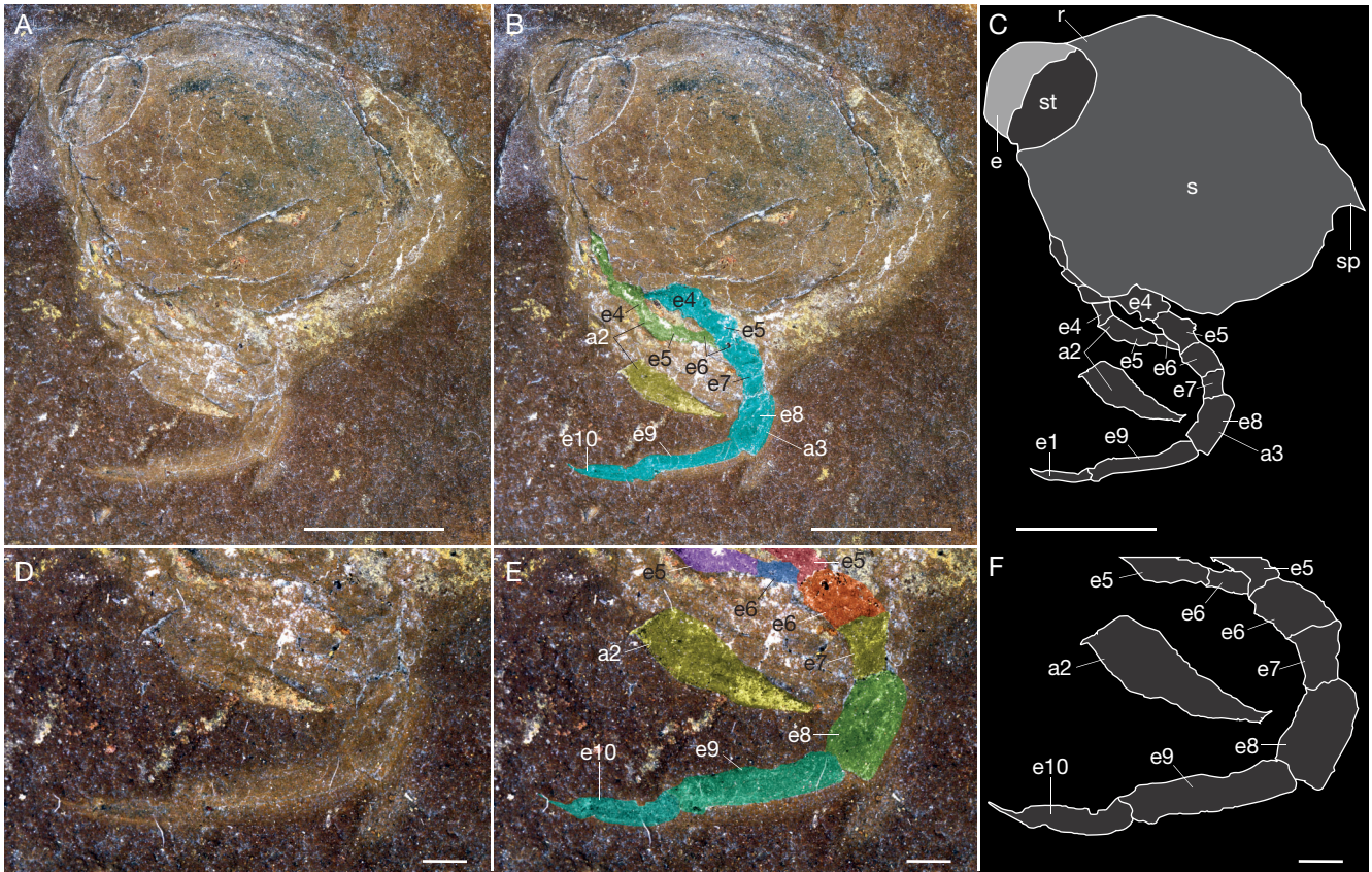
FIG. 3. — Concavicularis georgeorum Schram, 1990, ROMIP61587: A , general view; B , general view (color-marked); C , line drawing of general view; D , close-up of the third raptorial appendage; E , close-up of the third raptorial appendage (color-marked); F , line drawing of the third raptorial appendage. Abbreviations: a2 , a3 , second, third raptorial appendages; e , eyes; e4-e10 , element 4-10; r , rostrum; s , shield; sp , posterior spine; st , stalk. Photographs: C. Haug and J. T. Haug. Line drawings: T. Laville. Scale bars: A-C, 5 mm; D-F, 1 mm.
