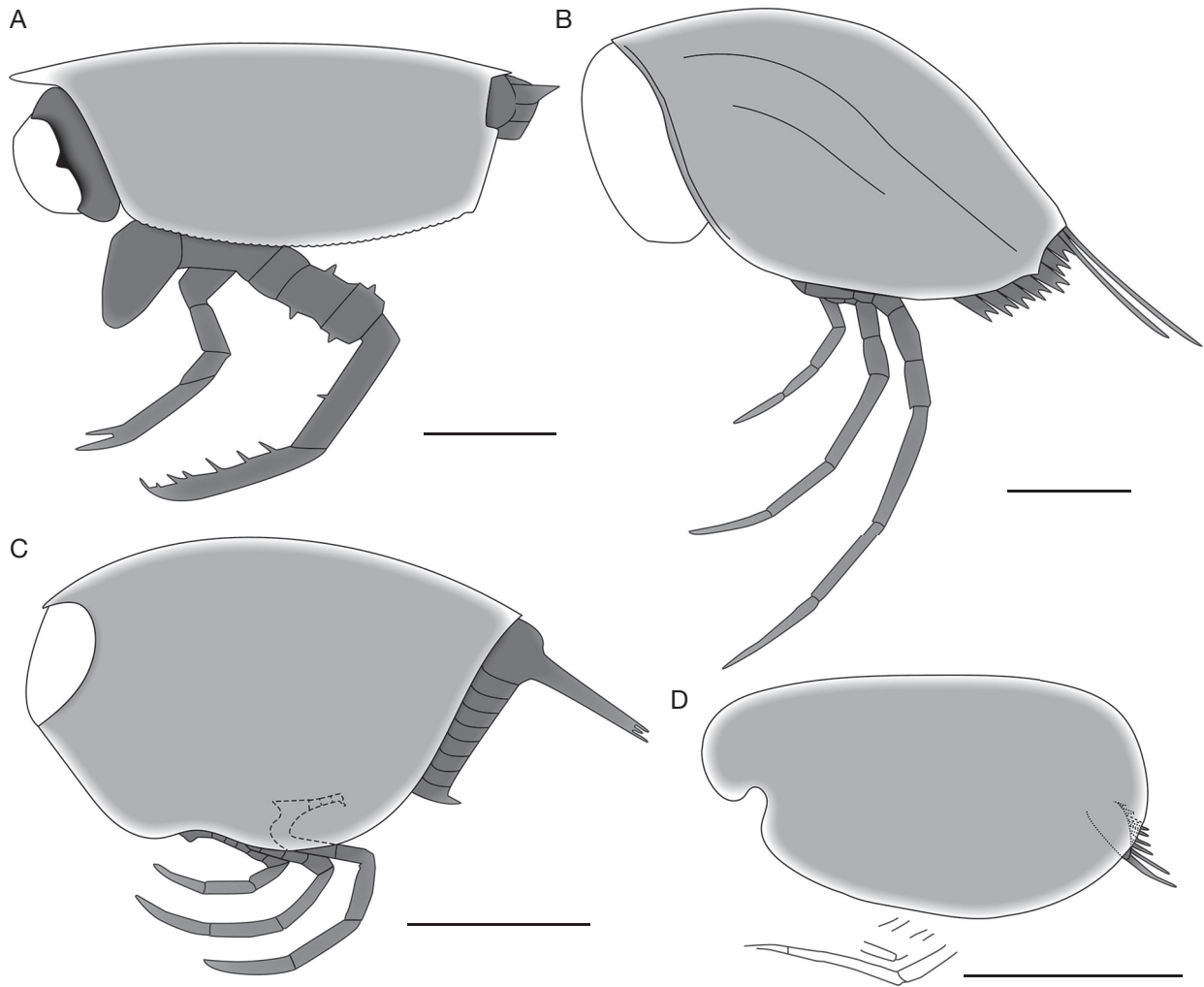
FIG. 9. — Mazon Creek thylacocephalans and possible representative of Myodocopida: A , reconstruction of Eodollocaris keithflinti n. gen., n. sp.; B , reconstruction of Convexicaris mazonensis Schram, 1990; C , reconstruction of Concavicularis georgeorum Schram, 1990; D , reconstruction of Concavicularis remipes Schram, 1990. B-D , adapted from Schram (1990). Scale bars: A-D, 5 mm.
