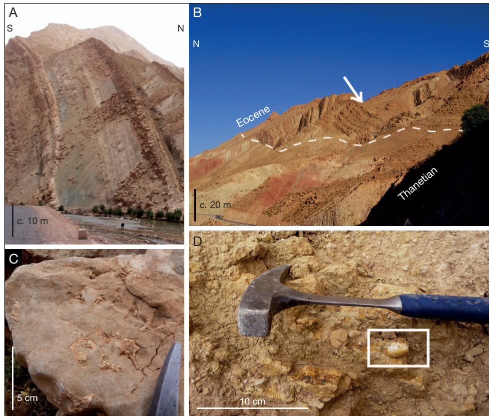
FIG. 2. — Field photographs from the Jbel Talout area: A , tilted strata of the Jbel Talout outcropping in the Tourbict gorges. This shows the high degree of tectonic deformation within the sub-Atlas thrust belt; B , view of the Tamalout section on the northern face of the Jbel Talout. The dot line corresponds to the limit between the Thanetian and Eocene sedimentary units. The white arrow shows the location of the Carpiliidae site; C , vertebrate bone fragments coming from the beds that overlies the Carpiliidae marls. Those beds are the lateral equivalent of those of the Aznag vertebrate site; D , in the white box is Maurocarpilus binodosus n. gen., n. sp. holotype, in situ , that is outcropping within the Eocene marls of the Ait Ouarhitane Formation.
