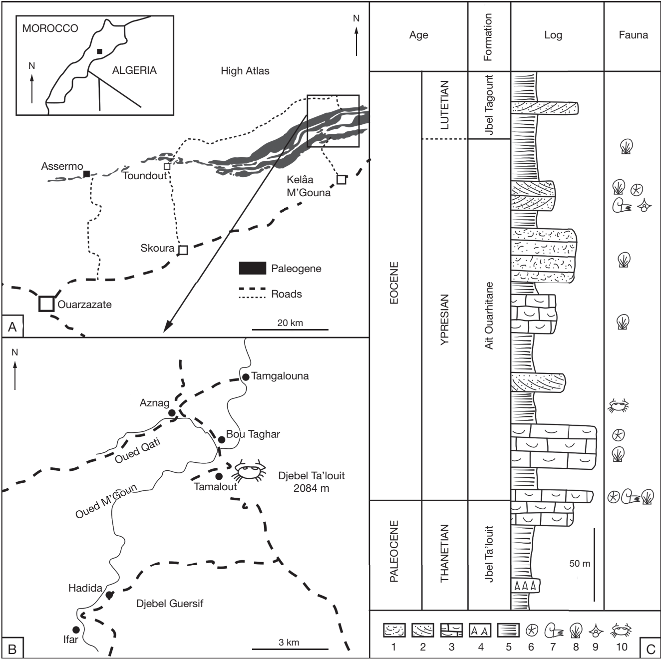
FIG. 1. — The geographical and geological contexts: A , location map of the Paleogene formations between Ouarzazate and Kelâa M'Gouna (Tabuce et al. 2005, modified); B , location of Tamalout paleontological site (Tabuce et al. 2005, modified); C , sedimentological section of the Tamalout site. 1, calcarenite; 2, sandstone; 3, bioclastic limestone; 4, gypsum; 5, marls; 6, urchins; 7, cephalopod nautiloids; 8, others molluscs; 9, vertebrates; 10, Maurocarpilus binodosus n. gen., n. sp.
