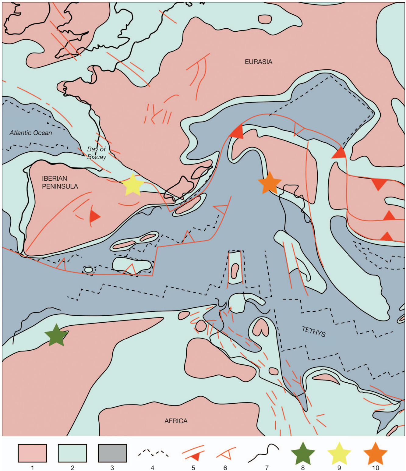
FIG. 5. — The paleogeographic map of the Tethys sea during the Ypresian (lower Eocene): 1, continental domain; 2, shallow marine domain; 3, deep marine domain, 4, oceanic crust boundary; 5, major thrust fault; 6, active subduction zone; 7, present-day coastlines; 8, Maurocarpius binodosus n. gen., n. sp.; 9, Eocarpilius ortegai and Oscacarpilius rotundus ; 10, Braggicarpilius marginatus and Carpiilius petreus . This map also shows a hypothetical connection between the Tethys sea and the Bay of Biscay through the South Pyrenees. This is suggested by the spatial distribution of fossil carpiiliids sites and imply a shallow marine corridor in the south of the Corso-Sardinian Block as also proposed by Colombo & Caus (1984). Adapted from Barrier et al. (2018).
