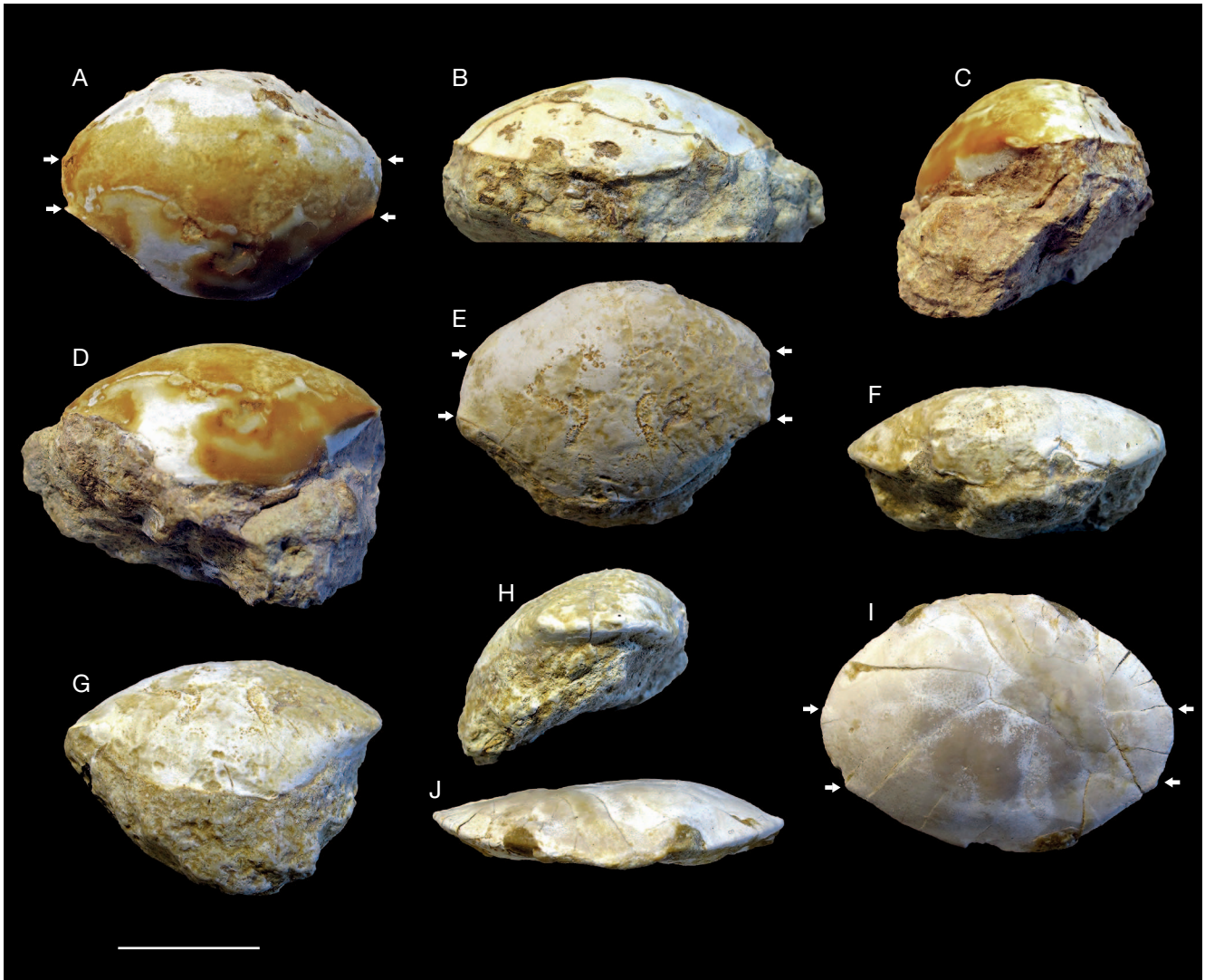
FIG. 3. — Maurocarpilus binodosus n. gen., n. sp., from the Ypresian (early Eocene) of Kelâa M'Gouna (Morocco): A–D , holotype ULB-IV-A(1a); A , dorsal view (digitally cut out of the matrix); B , frontal view; C , right lateral view; D , posterior view; E–H , paratype ULB-IV-A(1b); E , dorsal view; F , frontal view; G , posterior view; H , right lateral view; I, J , paratype ULB-IV-A(1c); I , dorsal view; J , frontal view. Arrows indicate the two anterolateral teeth distinctive of the species. Scale bar: 10 mm.
