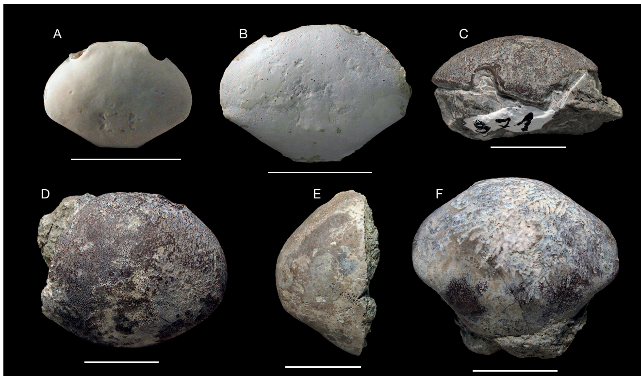
FIG. 4. — A , Braggicarpilius marginatus Beschin, Busulini & Tessier, 2015, holotype MCZ 3998, from the Ypresian (early Eocene) of Vestenanova (NE Italy) (digitally cut out of the matrix); B , Carpilius petreus Beschin, Busulini, De Angeli & Tessier, 2007, holotype MCZ 1809, from the Ypresian of Contrada Gecchelina (NE Italy) (digitally cut out of the matrix); C, D , Eocarpilius ortegai Artal & Van Bakel, 2018, topotype MGSB 77906a, from the Ilerdian (early Ypresian) of Isábena (N Spain); C , frontal view; D , dorsal view; E, F , Oscacarpilius rotundus Artal & Van Bakel, 2018, from the Ilerdian of Isábena (N Spain); E , topotype MGSB 77905b; F , topotype MGSB 77905a. Scale bars: A, 5 mm; B–F, 10 mm.
