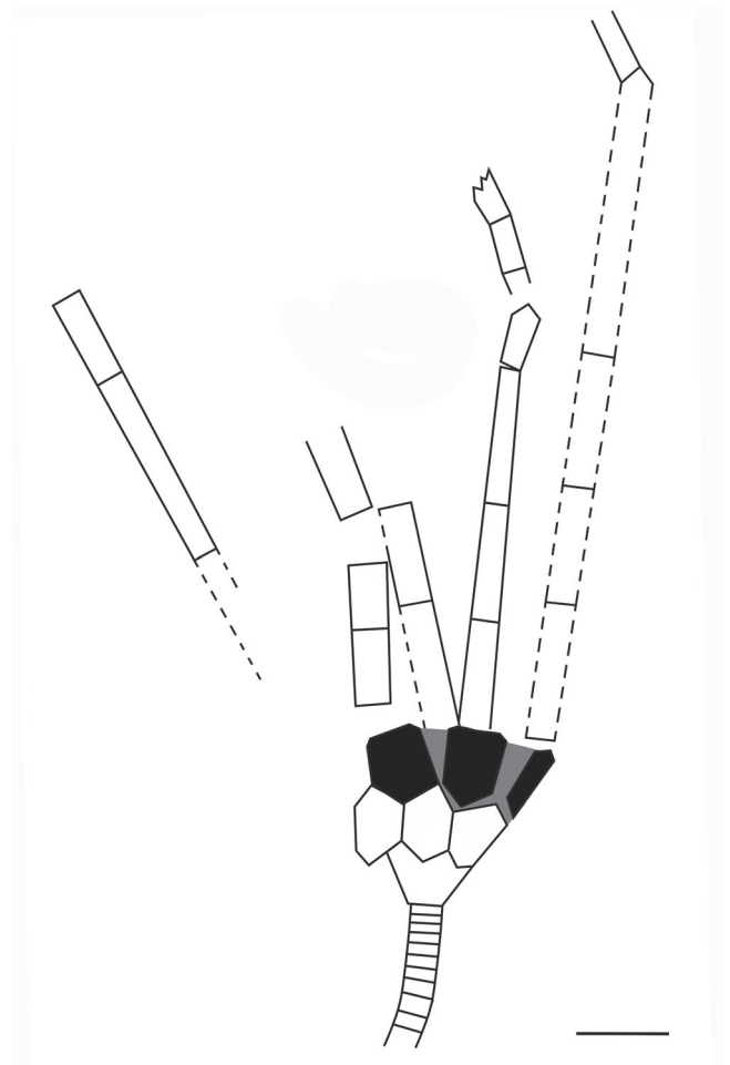
FIG. 4. — Plate diagram of Dendrocrinidae? gen., sp. indet. Black , radial plates; grey , matrix; Scale bar: 1.0 mm.
