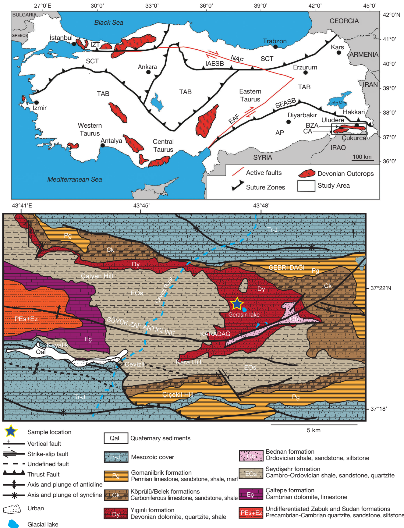
FIG. 1. — Distribution of Devonian units in Turkey (after Göncüoğlu 1997): A , tectonic map of Turkey with Devonian outcrops indicated; B , geological map (after Şenel 2002) of the Büyük Zap Anticline with the location of the crinoid bearing sample. Abbreviations: AP , Arabian Platform; BZA , Büyük Zap Anticline; CA , Çukuroca Anticline; IAESB , İzmir-Ankara-Erzincan Suture Zone; IZZ , İstanbul-Zonguldak Terrane; NAF , North Anatolian Fault; SEASB , Southeast Anatolian Suture Belt; SCT , Sakarya Composite Terrane; TAB , Tauride-Anatolide Belt.
