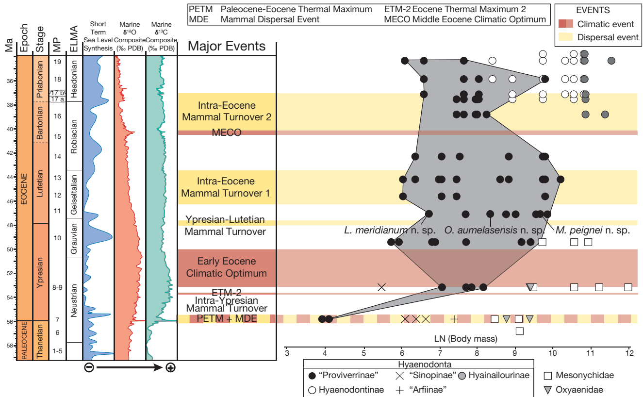
FIG. 5. — Values of the Ln (body mass) of mesonychids, oxyaenids, and hyaenodonts ("Proviverrinae" sensu Solé (2013), "Sinopinae", "Arfiinae", Hyaenodontinae, and Hyainailourinae) from MP7 to MP19 with particular attention on hyaenodonts from Aumelas. Aumelas is here represented to be close to the MP11 reference-level. Abbreviations: ELMA , European Land Mammal Ages; EMP , Mammal Palaeogene. Values are available at Appendix 6.
