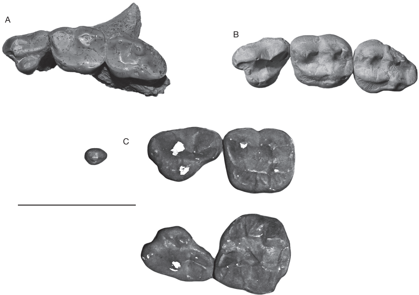
FIG. 7. — Other Indarctos species for comparison with I. punjabiensis (Lydekker, 1884) of Las Casiones: A , I. vireti Villalta & Crusafont, 1943; B , I. arctoides (Depéret, 1895) (from type locality); C , I. punjabiensis (syntype). All images are in occlusal view. Scale bar: 5 cm.
