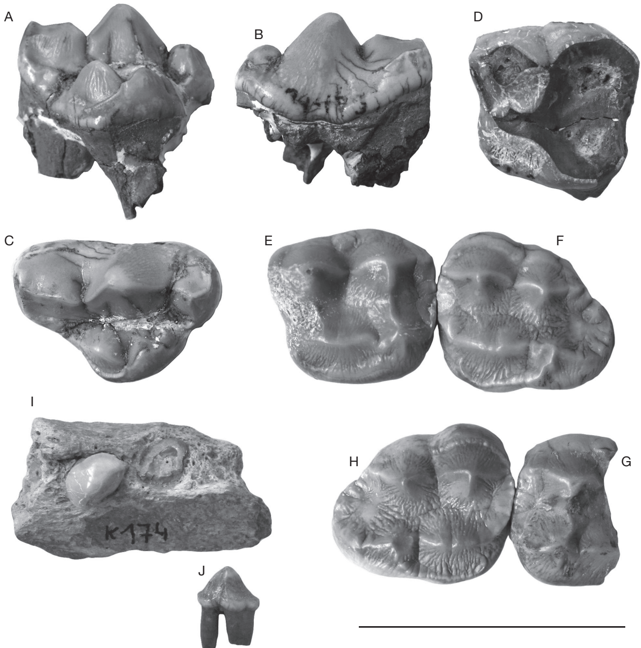
FIG. 2. — Indarctos punjabiensis (Lydekker, 1884) from Las Casiones: A-C , K94-1733, right P4: A , lingual view; B , labial view; C , occlusal view; D , K-162, left M1, occlusal view; E , KS-4316, left M1, occlusal view; F , KS-4317, left M2, occlusal view; G , K-161, distal fragment of right M1, occlusal view; H , KS-4315, right M2, occlusal view; I , K-174, left maxillary fragment with P2 and root of P1 and P3 (occlusal view); J , lower premolar, labial view. Scale bar: 5 cm.
