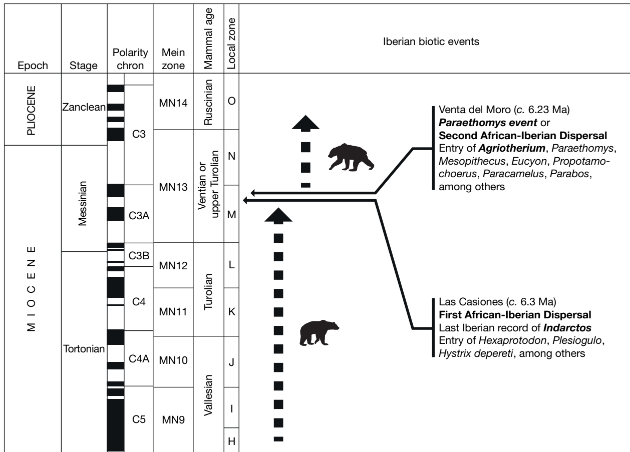
FIG. 8. — Biochronology showing the stratigraphic ranges of the genera Indarctos Pilgrim, 1913 and Agriotherium A. Wagner, 1837 in the Iberian Peninsula, related to the two biotic events recorded during the Messinian. Mammal ages and local zones according to Morales et al. 2013. Absolute age after Gibert et al. 2013.
