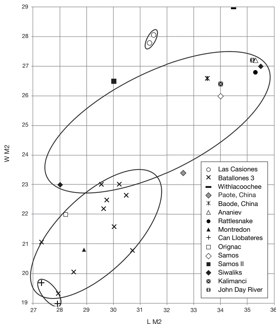
FIG. 6. — Bivariate plot of the M2 of different Indarctos Pilgrim, 1913 species from various sites.
