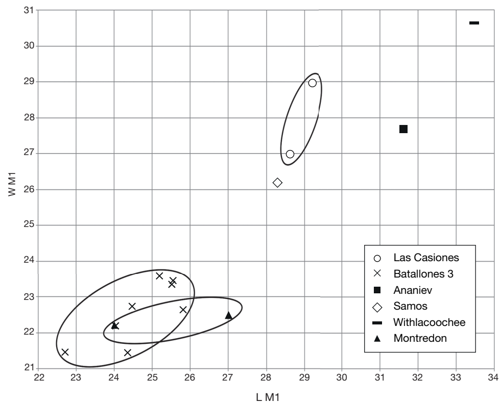
Fig. 5. — Bivariate plot of the M1 of different Indarctos Pilgrim, 1913 species from various sites.
