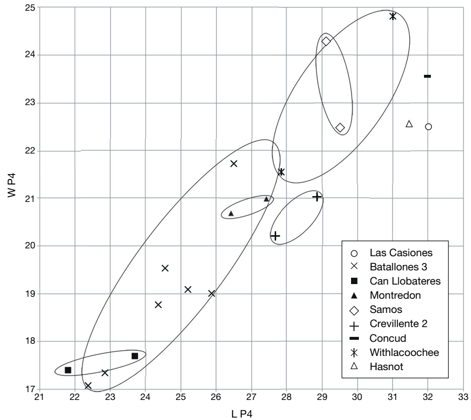
Fig. 4. — Bivariate plot of the P4 of different Indarctos Pilgrim, 1913 species from various sites.
