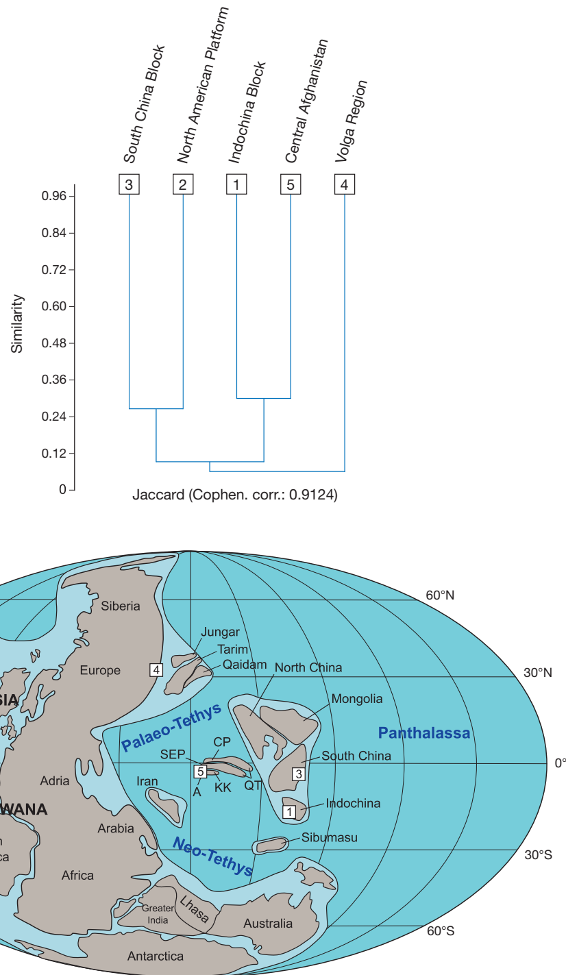
FIG. 9. — Dendrograms of UPGMA analysis based on 5 loci during the Roadian, Middle Permian. The scale indicates the grade of similarity as determined with the Jaccard coefficient of similarity. Schematic reconstruction map of Roadian-Wordian global palaeogeography (modified from Angiolini et al. 2013) with: A , Central Afghanistan; SEP , South East Pamir; CP , Central Pamir; QT , Qiangtang; KK , Karakoram.
