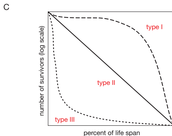
APPENDIX 4H. — Survivors per 2-years (a) and corresponding survivorship curve (b) of the Apollonia bison population, against standard types of survivorship curves (c). The survivors per 2-years curve (red solid line in a) best fits a fourth degree polynomial function model (dotted line in a). The survivorship curve of the Apollonia bison population (b) does not match any of the three standard types (c; see text).
