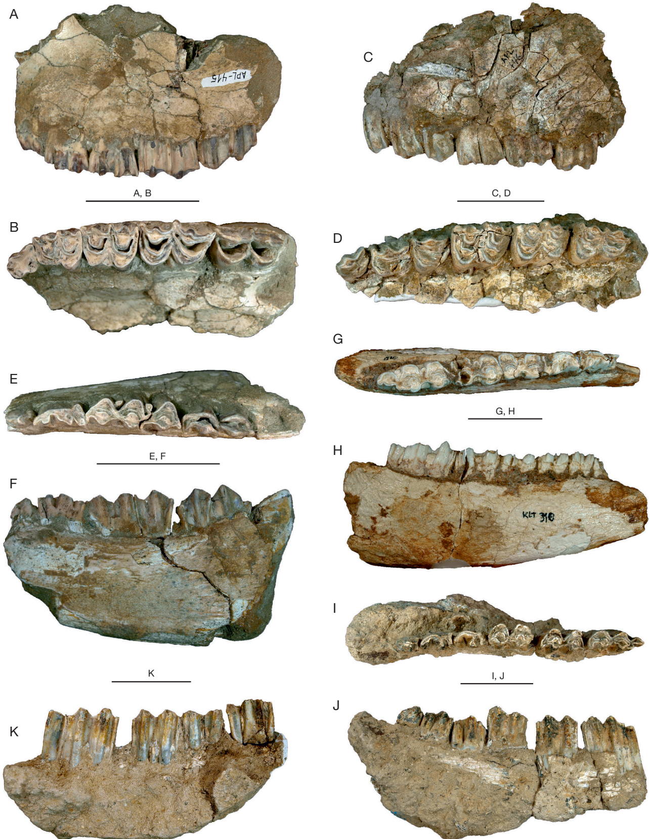
FIG. 3. — Dental remains of Bison cf. degiulii (Masini, Palombo & Rozzi, 2013) from Mygdonia Basin, Greece: A, B , left upper tooththrow with dP2-M2, APL-415, buccal ( A ) and occlusal ( B ) views; C, D , left upper tooththrow with P2-M3, APL-446, buccal ( C ) and occlusal ( D ) views; E, F , right mandible with dp3-m1, APL-420, occlusal ( E ) and lingual ( F ) views; G, H , left mandible with p3-m3, KLT-318, occlusal ( G ) and lingual ( H ) views; I, J , right mandible with p2-m3, TSR F20-16, occlusal ( I ) and lingual ( J ) views; K , left mandible with p4-m3, TSR D20-8, lingual view. Scale bar: 5 cm.
