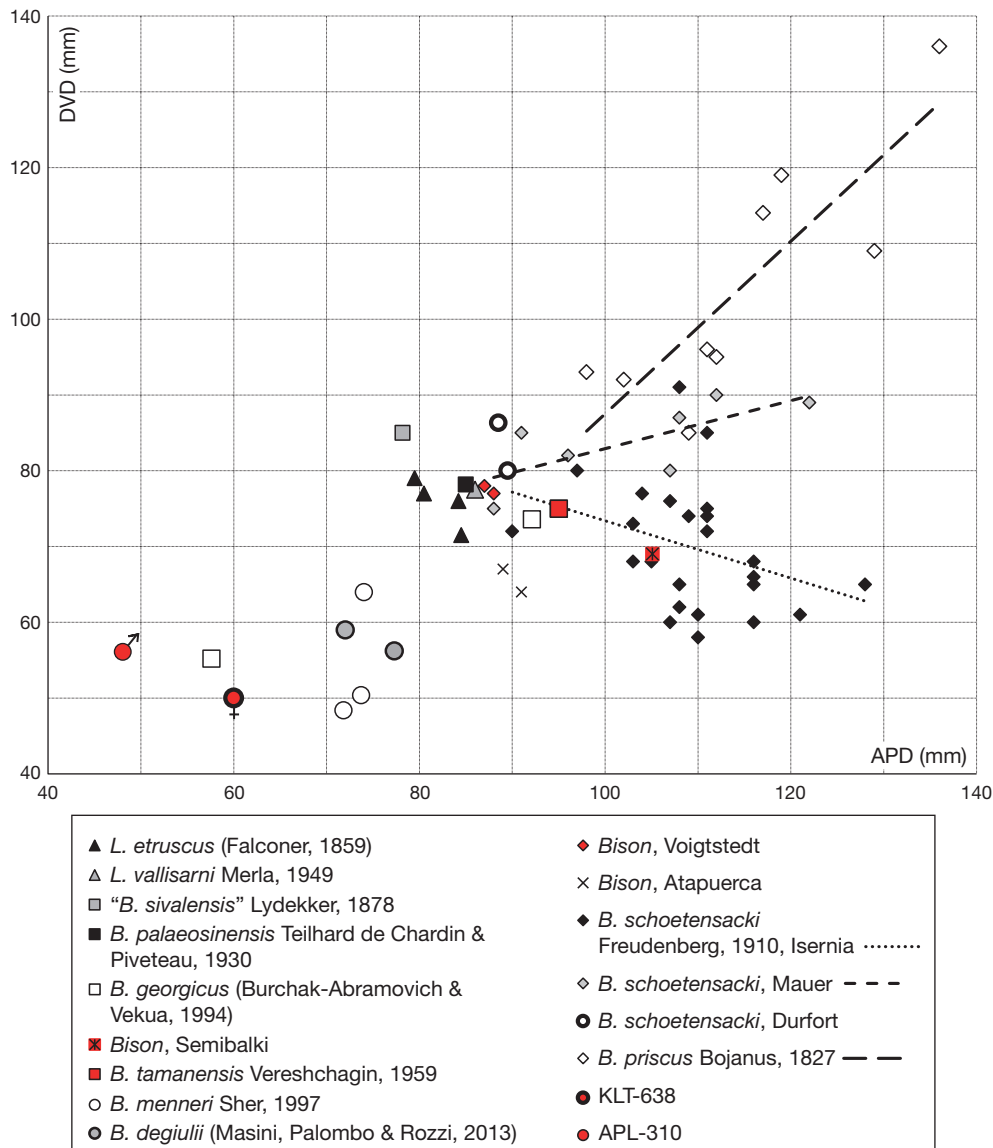
FIG. 12. — Bivariate diagram of basal horncore proportions [rostricaudal (APD) against dorsoventral (DVD) diameter] comparing several European Leptobos Rütimeyer, 1877-1878 and Bison Hamilton Smith, 1827 samples and species. Dashed lines represent regressions of B. schoetensacki (Isernia la Pineta and Mauer) and B. priscus .
