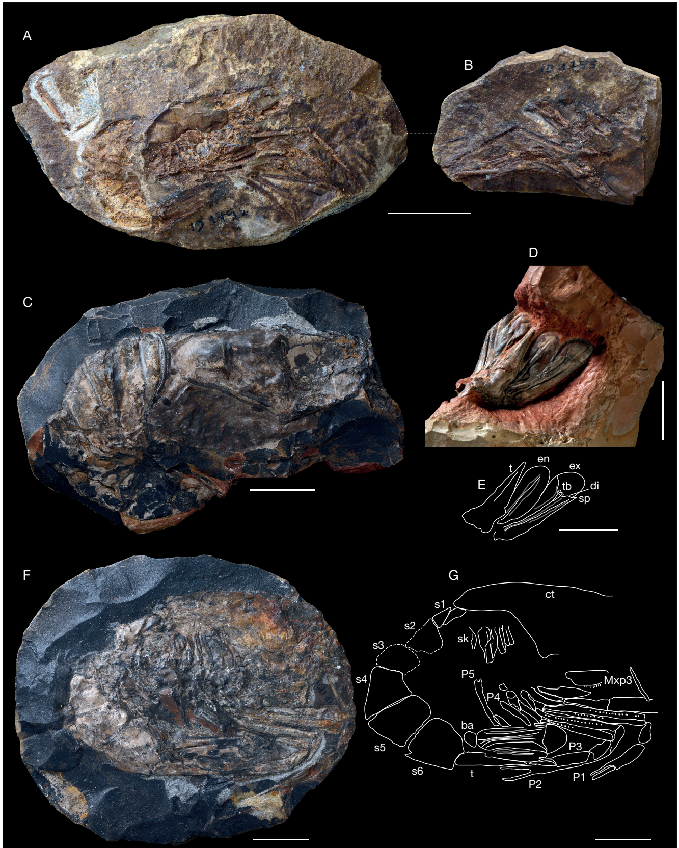
FIG. 1. — Aeger brevirostris Van Straelen, 1923 from the La Voulte Lagerstätte: A, B , specimen UJF-ID.1754-55 (lectotype; coll. Gevrey), right lateral view, part A , UJF-ID.1755) and counterpart ( B , UJF-ID.1754); C-E , specimen UJF-ID.14031 (paralectotype; coll. Gevrey), right dorsolateral view ( C ), detail ( D ) and line drawing ( E ); F, G , specimen UJF-ID.1790 (lectotype of Antrimpos kiliani Van Straelen, 1923; coll. Gevrey), right lateral view ( F ), line drawing ( G ). Abbreviations: ba , basipodite; ct , cephalothorax; di , diaeresis; en , uropodal endopod; ex , uropodal exopod; Mxp3 , third maxilliped; P1-P5 , pereopods 1 to 5; s1-s6 , pleonal somites 1 to 6; sk , endophragmal skeleton; sp , spine; t , telson; tb , tubercles. Photographs: A-C, F , L. Cazes; D, N , PODEVIGNE. Line drawings: C. JAUVION. Scale bars: 20 mm.
