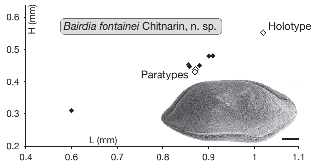
FIG. 5. — Height (H)-length (L) diagram of Bairdia fontainei Chitnarin, n. sp. Scale bar: 100 µm.
