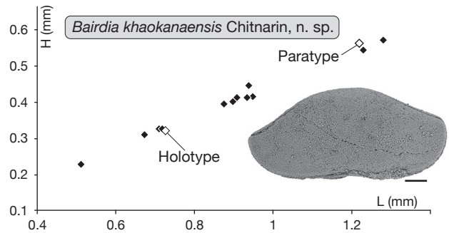
FIG. 4. — Height (H)-length (L) diagram of Bairdia khaokanaensis Chitnarin, n. sp. Scale bar: 100 µm.
