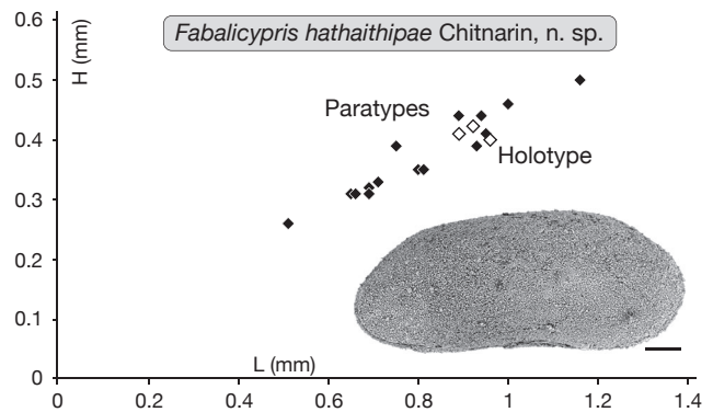
FIG. 18. — Height (H)-length (L) diagram of Fabalicypis hathaithipae Chitnarin, n. sp. Scale bar: 100 µm.
