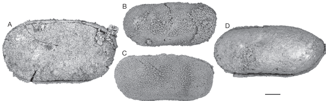
FIG. 17. — Ostracods from Guadalupian-Lopingian boundary interval in South China. A , Sulcella mesopermiana ? Kozur, 1985, P6M3771, 11CHAO88; B , Sulcella suprapermiana ? Kozur, 1985, P6M3772, 11CHAO166; C , P6M3773, 11CHAO81; D , Sulcella sp. 1, P6M3774, sample 11CHAO88. All photographs represent complete carapaces in left lateral view. Scale bar: 100 \mu m.
