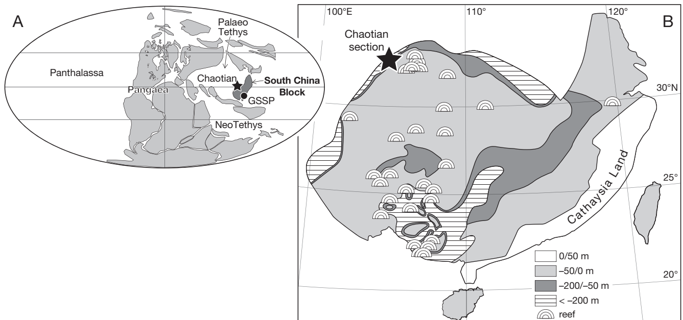
FIG. 3. — A , Palaeogeographic map of the Middle-Late Permian (modified after Golonka 2002); B , distribution of Carboniferous palaeoenvironments in South China (map in present day latitudes, modified from Wang & Jin 2000).
