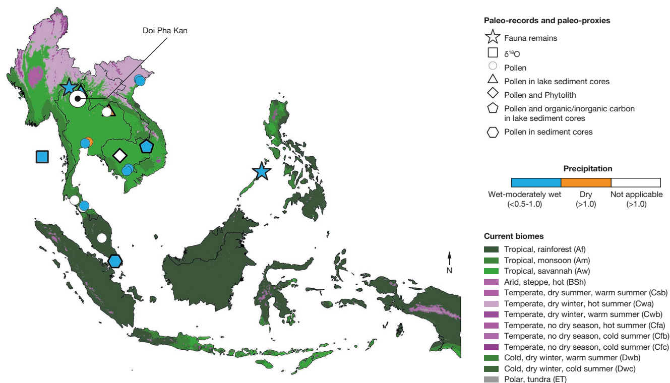
FIG. 4. — Paleo-records and paleo-proxies available in Thailand during Early Holocene (between 10 500 and 8 000 cal BP) (White et al. 2004; Chabangborn 2014; Chawchai 2014; Ochoa et al. 2014; Shoocongdej & Wattanapitaksakul 2020). Base map: Köppen-Geiger climate classification of Southeast Asia (Beck et al. 2018).
