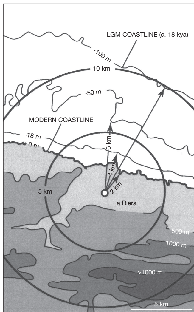
FIG. 4. — La Riera showing simplified topography, bathymetric contours and approximate distance to former coastlines. The -100 m contour approximates the position of the coast at the LGM (c. 18 kya) (redrawn from Bailey & Craighead 2004: 191).
