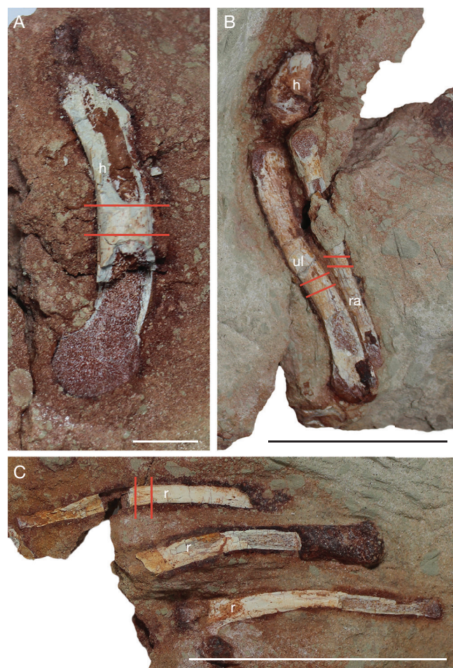
Fig. 1. — Bone elements of Mariliasuchus amarali Carvalho & Bertini, 1999 UFRPE 5311: A , right humerus, lateral view; B , right ulna and radius, lateral view; C , ribs. The red lines mark the sampling location. Abbreviations: h, humerus; r, rib; ra, radius; ul, ulna. Scale bars: A, 1 cm; B, C, 5 cm.
