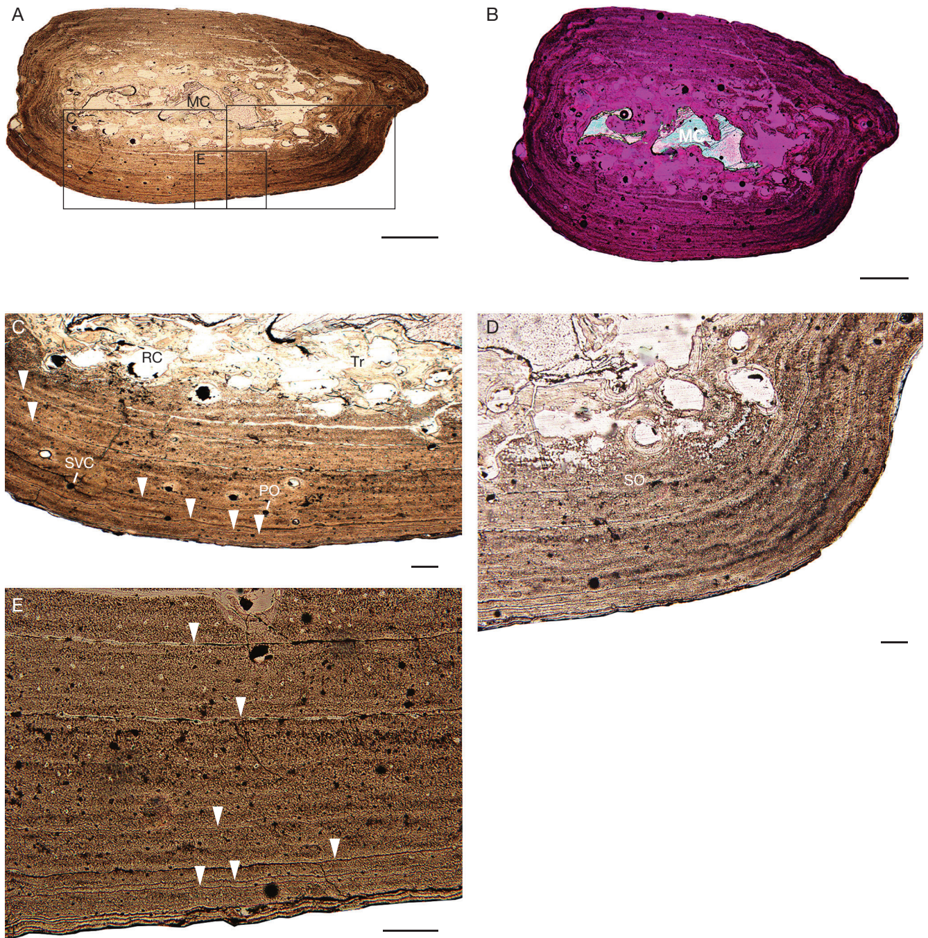
FIG. 2. — Transverse histological sections: A, B , microanatomical overview of the rib of Mariliasuchus amarali Carvalho & Bertini, 1999 UFRPE 5311; C , close-up of A , showing typical features of the cortex of the rib: parallel-fibered tissue and LAGs; D , close-up of A , the medullary region is marked by secondary trabeculae, resorption cavities and a secondary osteon; E , close-up of A , showing five distinct growth zones separated by LAGs in the cortex, the third zone is the largest. Abbreviations: MC , medullary cavity; PO , primary osteon; RC , resorption cavity; SO , secondary osteon; SVC , simple vascular canal; Tr , trabecula. The white arrows correspond to LAGs. Images: normal transmitted light ( A, C and D ) and cross polarized light with lambda compensator ( B ). Scale bars: A, B , 1 mm; C , 100 \mu m; D, E , 200 \mu m.
