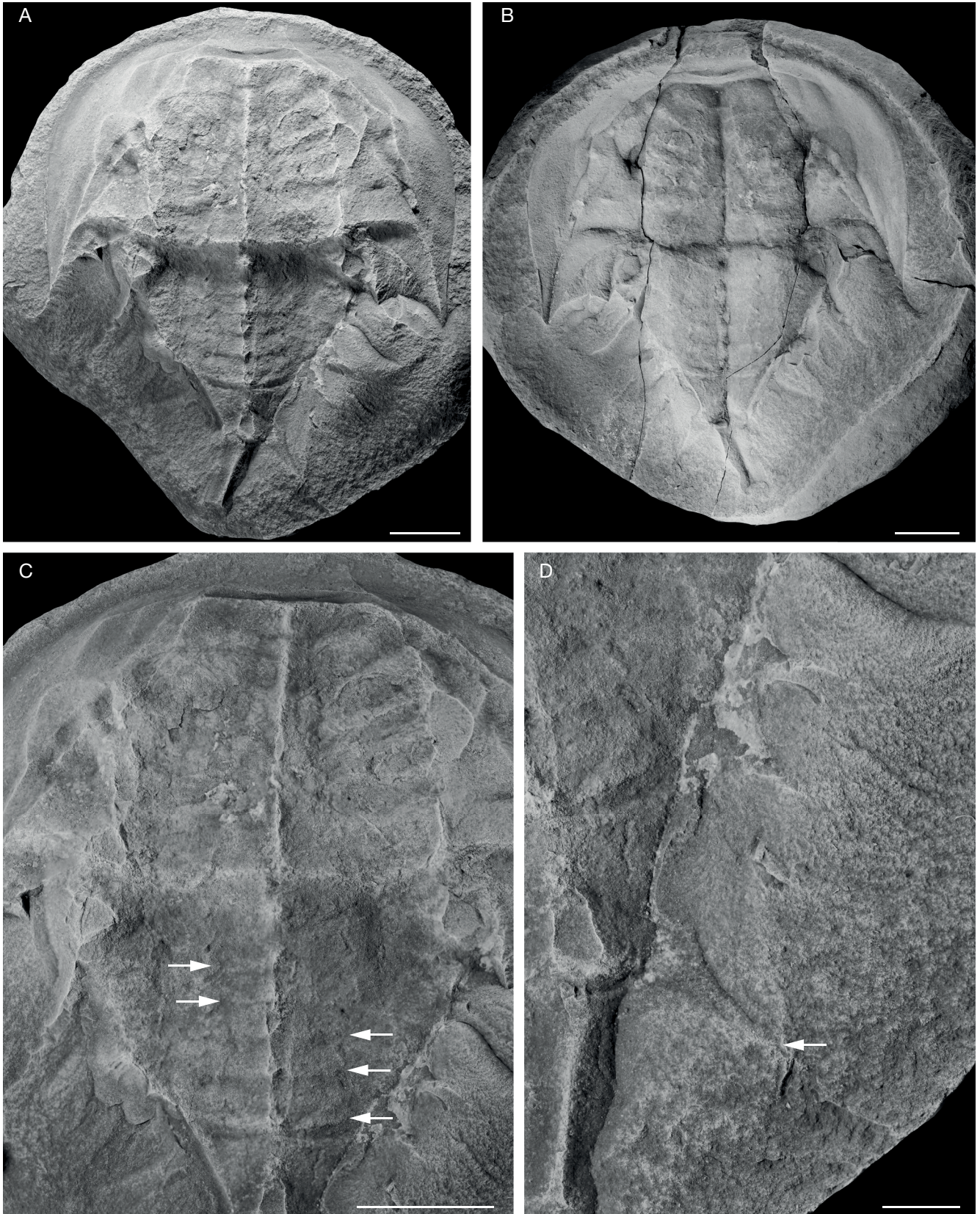
FIG. 5. — Paleolimulus mazonensis n. sp. showing possible posterolaterally deflected terminal spine: A–D , FMNH PE 84078. A , C , D , FMNH PE 84078a, part: A , complete specimen; C , close up of prosoma and thoracetrone showing longitudinal thoracetrone ridges ( white arrows ); D , close up of right pleural lobe showing possible posterolaterally deflected terminal spine ( white arrow ). B , FMNH PE 84078b, counterpart. All specimens coated in ammonium chloride sublimate and images converted to greyscale. Image credits: Russell Bicknell. Scale bars: A–C, 5 mm; D, 2 mm.
