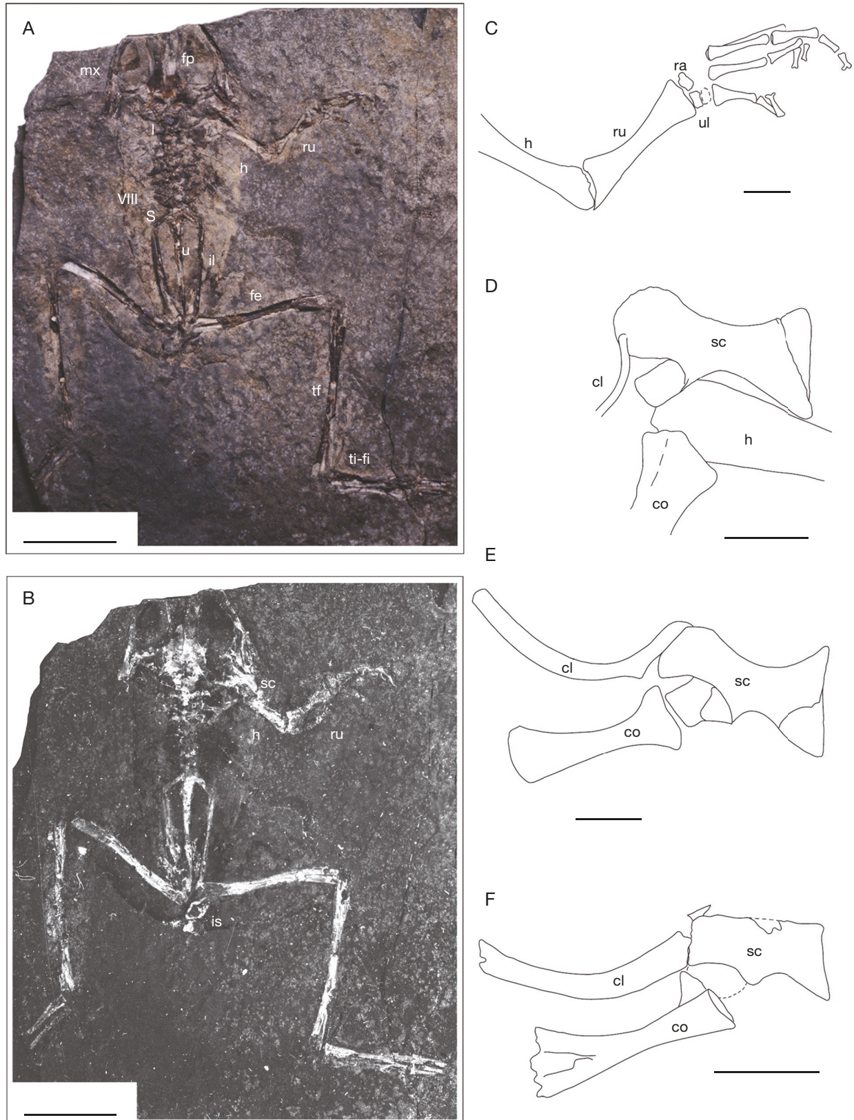
FIG. 2. — Wealdenbatrachus Fey, 1988 sp. (MUPA-LH 00004, individual exposed in ventral view): A , general view (photograph under incandescent light); B , general view (photograph under UV light); C , interpretive drawing of left anterior limb; D , interpretive drawing of part of left pectoral girdle in ventral view; E , Wealdenbatrachus jucarensis Fey, 1988 from Uña, restoration of part of the pectoral girdle in ventral view (redrawn from Báez & Gómez 2019); F , MUPA-LH 05429, interpretive drawing of part of the right side of pectoral girdle in ventral view, reversed for comparison. Abbreviations: cl , clavicle; co , coracoid; fe , femur; fp , frontoparietal; h , humerus; il , ilium; is , ischion; mc , metacarpal; mx , maxilla; ra , radiale; ru , radioulna; s , sacrum; sc , scapula; tf , tibiofibular; ti-fi , tibiale-fibulare; u , urostyle; ul , ulna; I-VIII , presacral vertebrae I-VIII. Scale bars: A, B, 10 mm; C-F, 2 mm.
