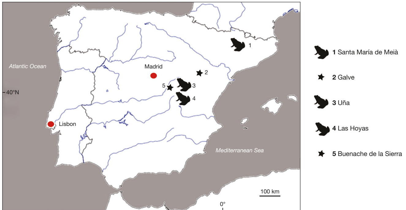
FIG. 1. — Map of the Iberian Peninsula showing the geographical location of Barremian sites from which anuran remains have been collected. Stars denote scarce, fragmentary, disarticulated bones; frog silhouettes denote more complete or articulated remains.
