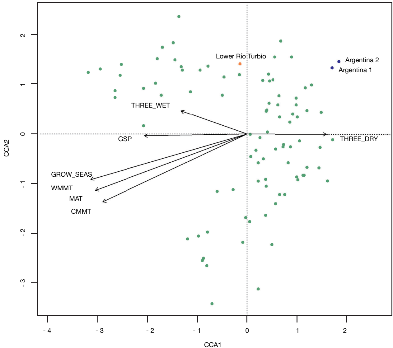
Fig. 4. — Canonical Correspondence Analysis using CLAMP SH90 dataset. The axes CCA1 and CCA2 accumulate a total of 0.32% of the variance.
