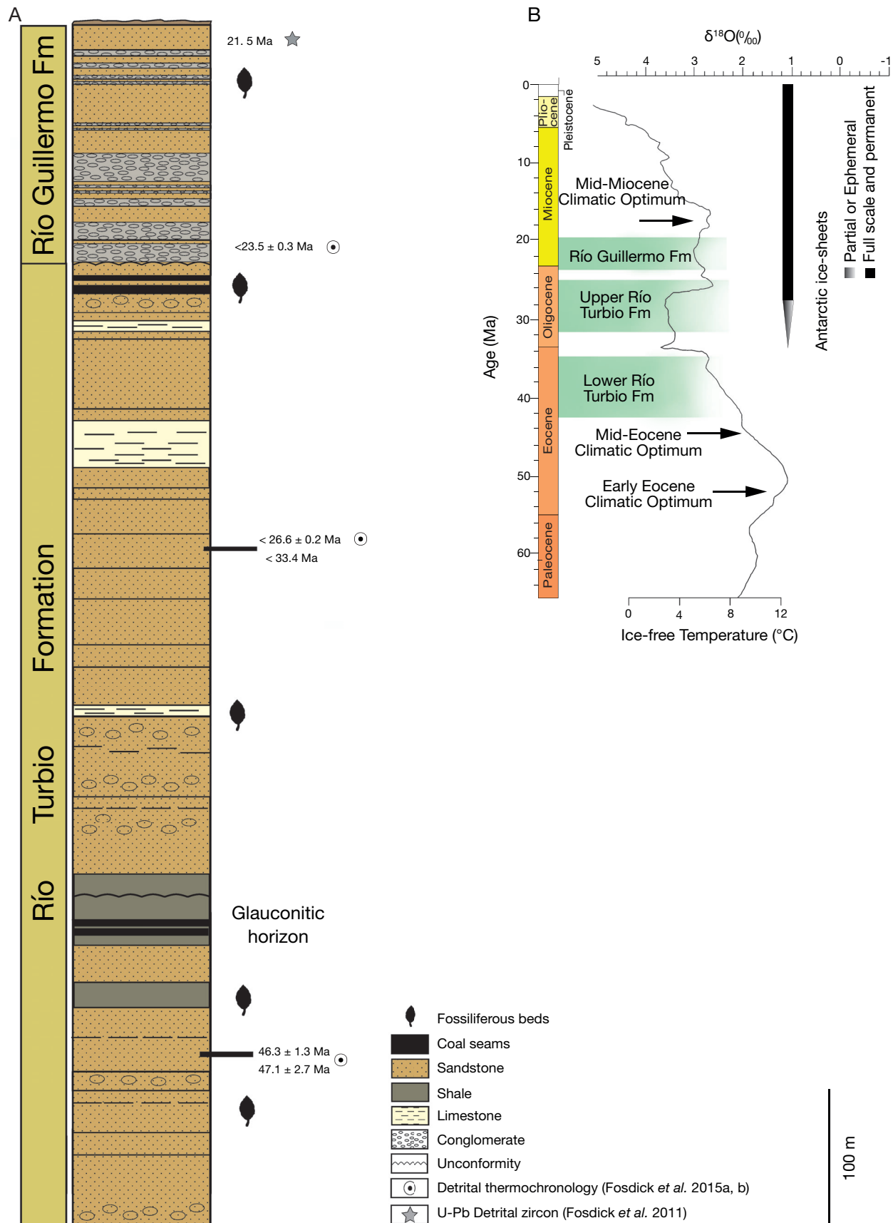
FIG. 2. — A , Stratigraphic composite profile from Río Turbio and Río Guillermo formations (modified from Hünicken 1967) with U/Pb detrital zircon age calibration based on Fosdick et al. (2011, 2015a, b); B , global climate fluctuations from stable isotopes (Zachos et al. 2008).
