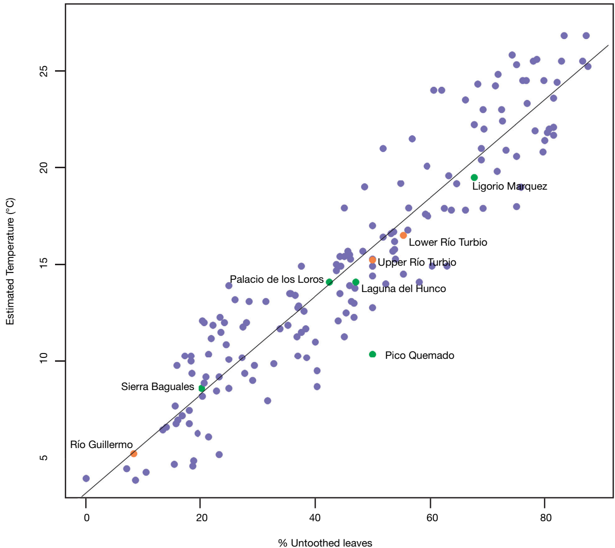
FIG. 5. — Correlation between mean annual temperature and leaf margin from the Río Turbio and Río Guillermo formations and published fossil sites in South America during the Eocene-Oligocene-Miocene.
