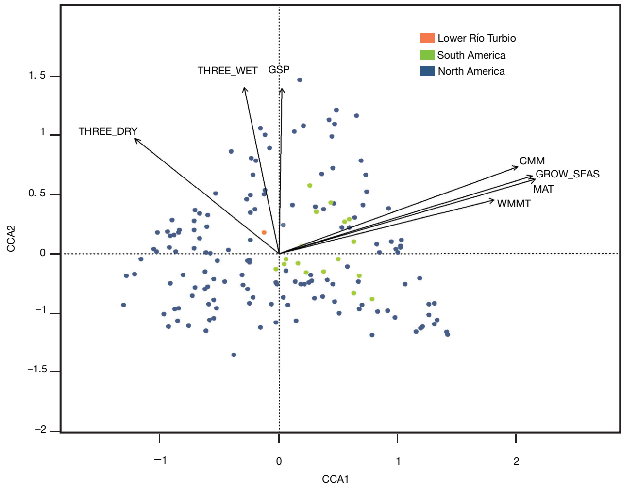
FIG. 3. — Canonical Correspondence Analysis using CLAMP3B SA dataset. The axes CCA1 and CCA2 accumulate a total of 0.64% of the variance.
