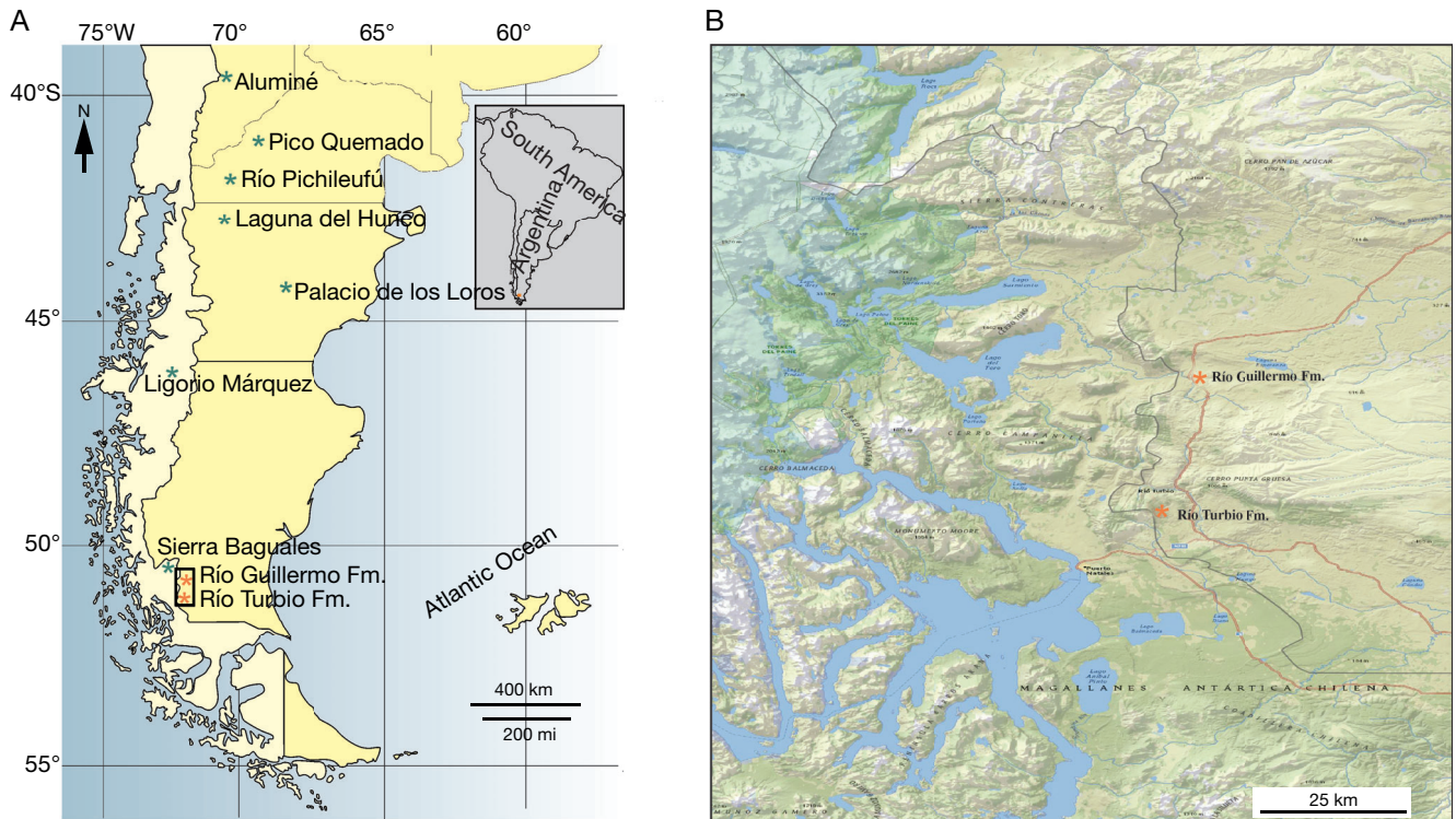
FIG. 1. — A , Map of southernmost South America with the location of the studied formations: Río Turbio and Río Guillermo and other sites from southernmost Chile and Argentina, which were used for the discussion; B , detailed of the location of the two studied areas in southern Argentina where the fossil leaves come from.
