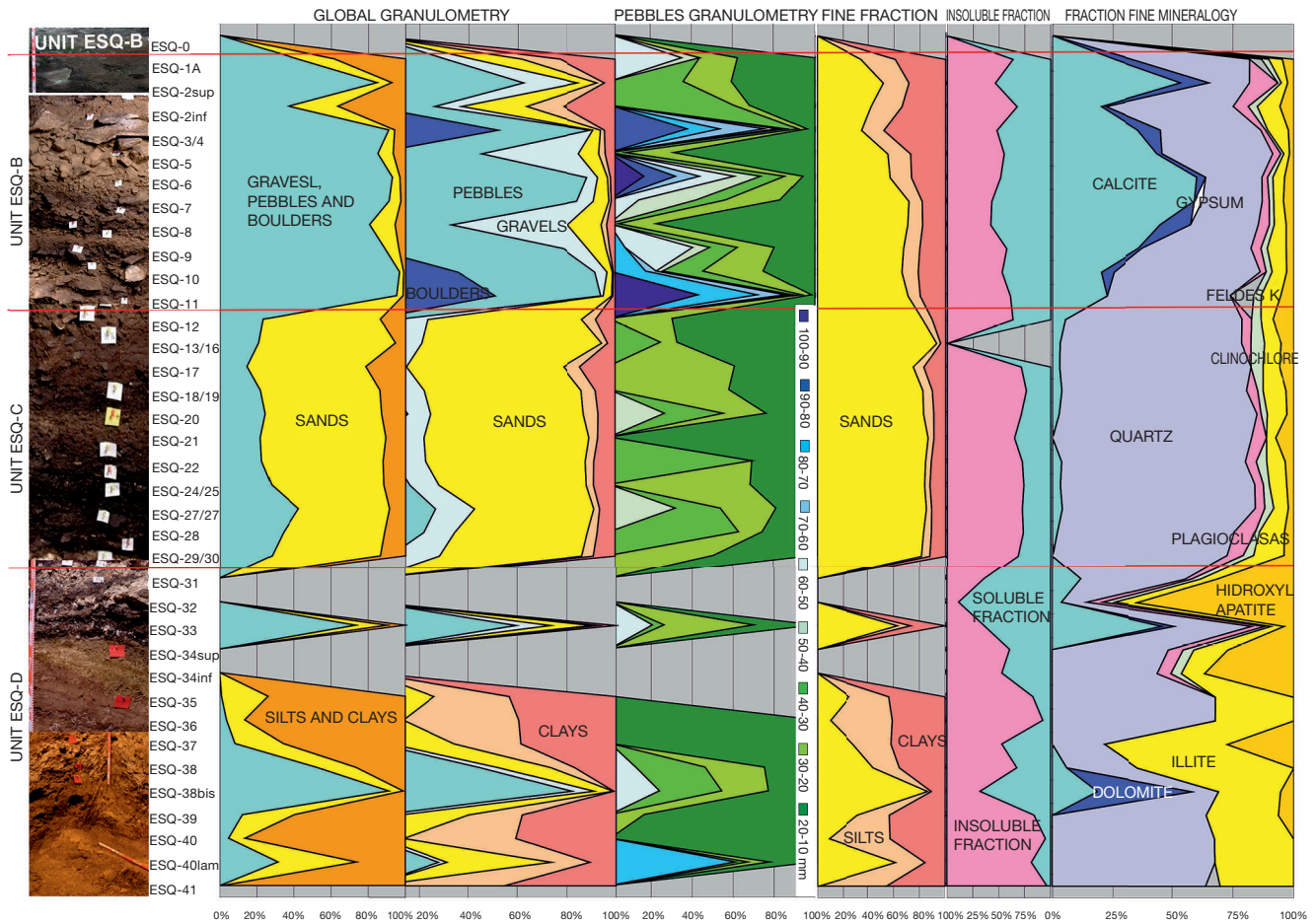
FIG. 3. — Summary of the lithostratigraphic sequence of the El Esquilleu cave showing the field, textural, and mineralogical characteristics as well as the differentiated lithostratigraphic units.
