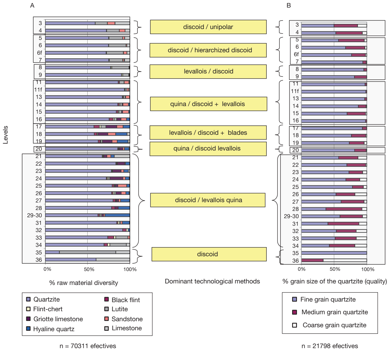
Fig. 5. — Raw material diversity, dominant technological methods and quartzite grain size (quality) along the El Esquilleu sequence.
