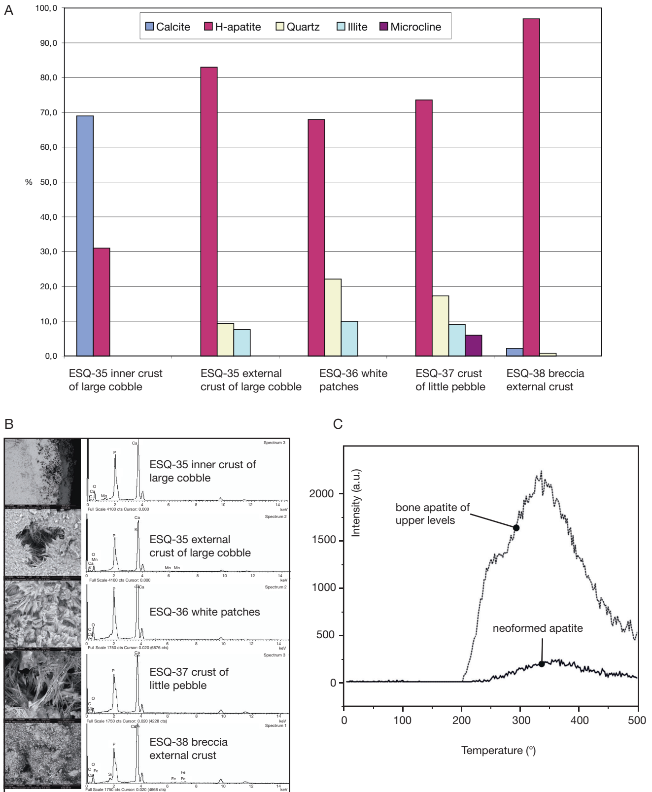
FIG. 4. — Esquilleu apatite crusts: A , Mineralogy (XRD) of the crusts of low levels of ESQ-D unit of the El Esquilleu cave sequence; B , ESEM photomicrographies under secondary electrons of different aggregates of fibrous hydroxyapatite and chemical analyses by dispersive energies of hydroxyapatites with changeable accessory quantities of silica, iron, magnesium and manganese; C , Thermoluminescence (TL) curves of primary apatite of a bone of upper units with TL's big signal due to its long geological history receiving environmental irradiations, in comparison with masses of recent neoformed apatite and with many minor doses of natural irradiations (TL's minor sign).
