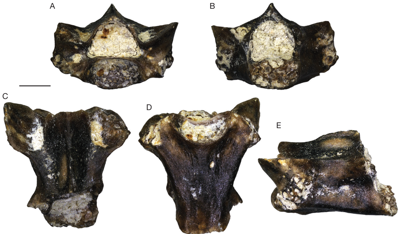
FIG. 10. — Ophisaurus sp. from Kavakdere: presacral vertebra EUNMH PV 14056 in anterior (A), posterior (B), dorsal (C), ventral (D), and left lateral (E) views. Scale bar: 1 mm.
