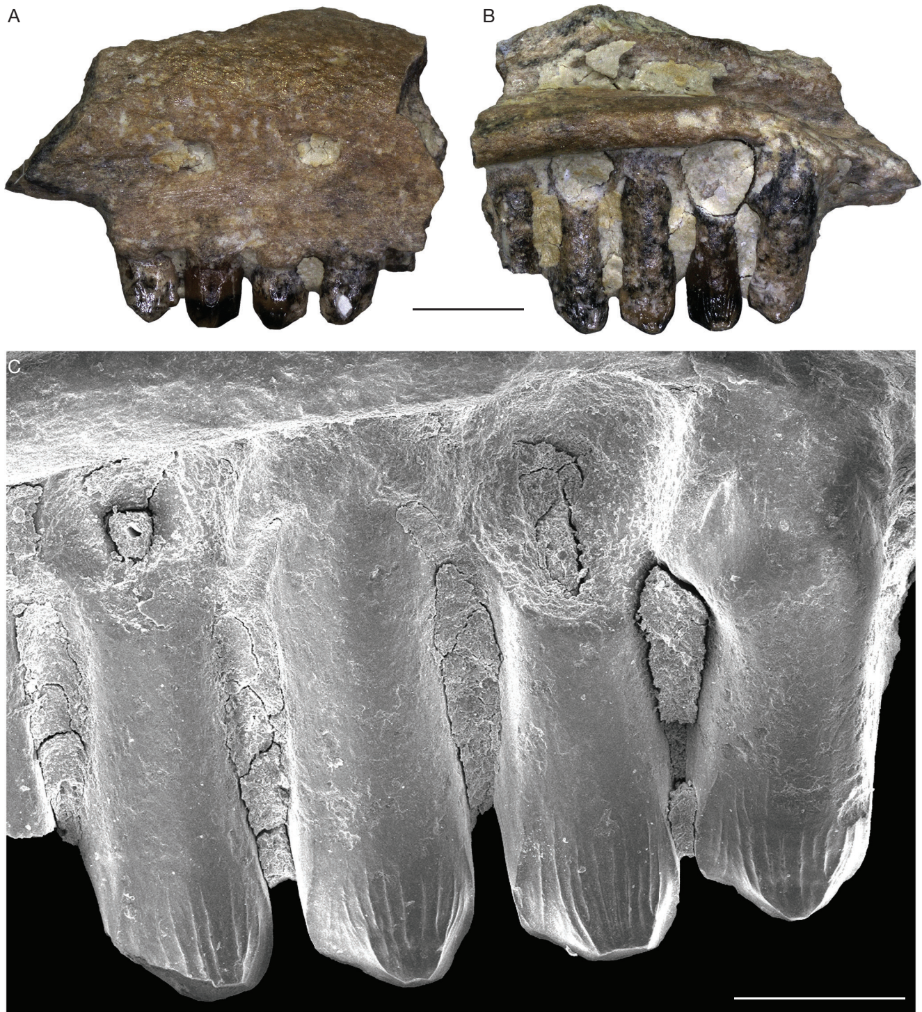
FIG. 6. — Lacertidae indet. (morphotype 1) from Kavakdere. Right maxilla EUNMH PV 14052 in labial (A) and lingual (B) views; C, close up SEM photograph of the same specimen showing the striation of the teeth. Scale bars: A, B, 1 mm; C, 0.5 mm.
