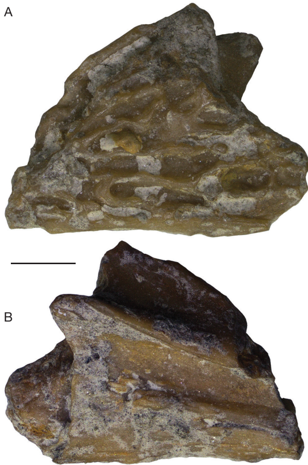
FIG. 3. — ? Eopelobates sp. from Kocayarma. Left maxilla EUNMH PV 14065 in labial (A) and lingual (B) views. Scale bar: 1 mm.
