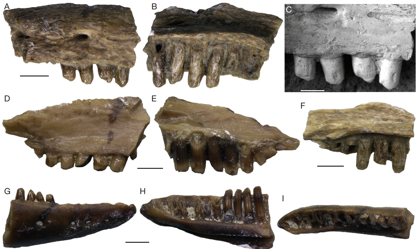
FIG. 7. — Lacertidae indet. (morphotype 1) from Kocayarma: A–B , maxilla EUNMH PV 14061 in labial ( A ) and lingual ( B ) views; C , close SEM photograph of the teeth of the same specimen; D, E , maxilla EUNMH PV 14064 in labial ( D ) and lingual ( E ) views; F , maxilla EUNMH PV 14066 in lingual view; G–I , Dentary EUNMH PV 14063 in labial ( G ), lingual ( H ), and dorsal ( I ) views. Scale bars: A, B, D–I, 1 mm; C, 0.5 mm.
