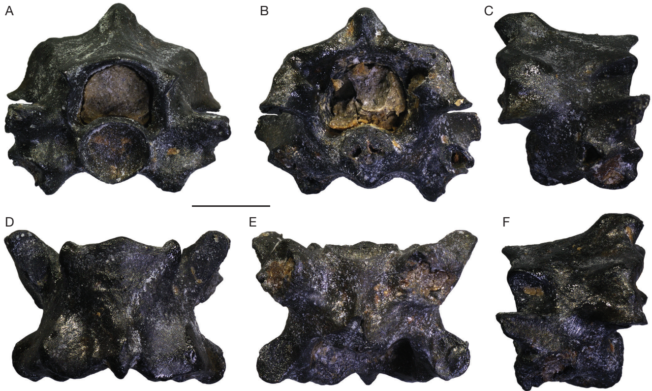
FIG. 12. — cf. Platyspondylia sp. from Kargi 2. Cloacal vertebra (EUNMH PV 14070) in anterior (A), posterior (B), right lateral (C), dorsal (D), ventral (E), and left lateral (F) views. Scale bar: 1 mm.
