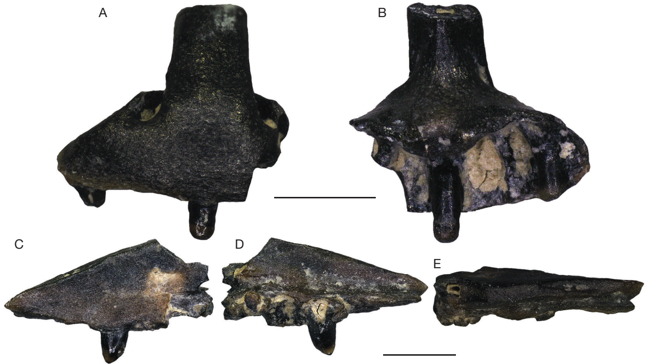
FIG. 8. — Lacertidae indet. (morphotype 2) from Kavakdere: A, B , premaxilla EUNMH PV 14055 in anterior ( A ) and posterior ( B ) views; C-E , right maxilla EUNMH PV 14058 in labial ( C ), lingual ( D ), and dorsal ( E ) views. Scale bars: A, B, 0.5 mm; C-E, 1 mm.
