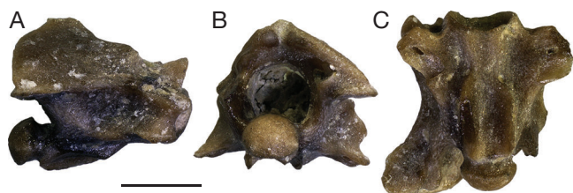
FIG. 13. — “Tropidophiidae” indet. from Kargi 2. Mid-caudal vertebra EUNMH PV 14072 in right lateral (A), posterior (B), and ventral (C) views. Scale bar: 1 mm.
