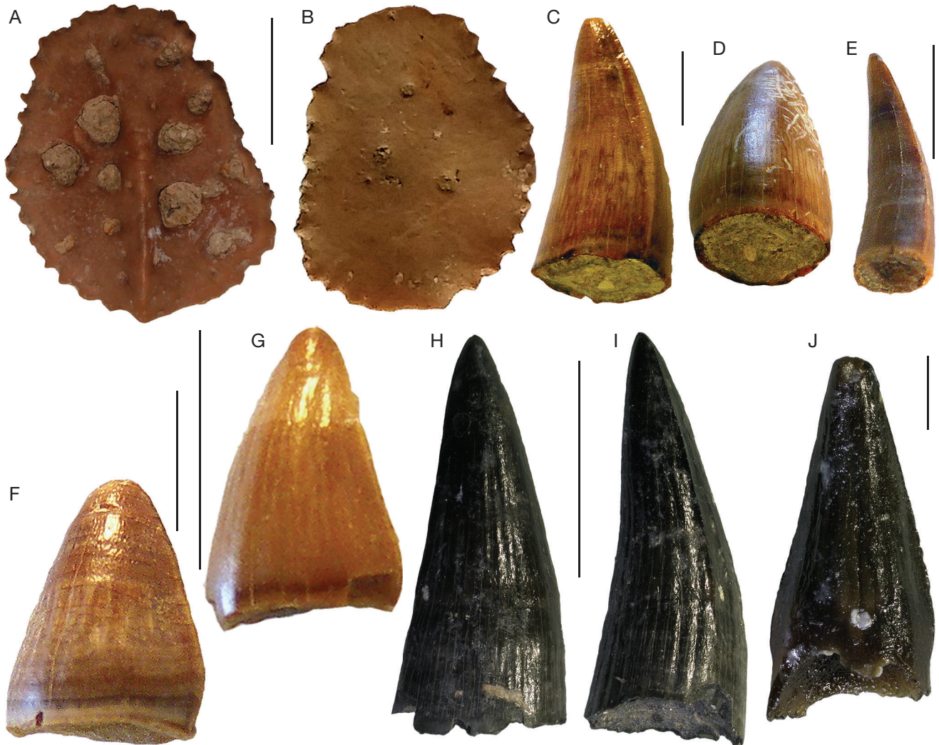
FIG. 5. — A, B , Crocodylia indet. from Kavakdere: osteoderm EUNMH PV 14073 in dorsal ( A ) and ventral ( B ) views. C–G , Crocodylia indet. from Kocayarma: C, D , tooth EUNMH PV 14087 in lingual ( C ) and ventrolingual ( D ) views; E , tooth EUNMH PV 14082 in mesial view; F , tooth EUNMH PV 14085 in lingual view; G , tooth EUNMH PV 14076 in labial view. H–J , Crocodylia indet. from Kargi 2: H, I , tooth EUNMH PV 14068 in labial ( H ) and mesial ( I ) views; J , tooth EUNMH PV 14069 in lingual view. Scale bars: A–I, 5 mm; J, 1 mm.
