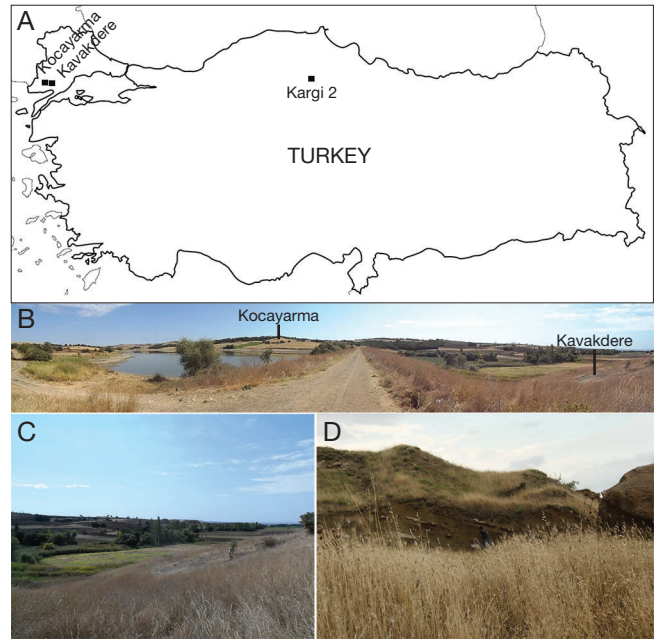
FIG. 1. — A , Map of Turkey, showing the localities Kocayarma, Kavakdere, and Kargi 2; B , panoramic photograph of the area of the nearby localities of Kavakdere and Kocayarma, showing their precise positions; C , photograph of the locality of Kavakdere; D , photograph of the locality of Kocayarma.
